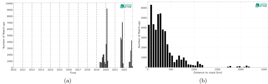
Figure 2: Number of match-ups between Saildrone and SMAP SSS L2 v5.0 (JPL) SSS as a function of time (a) and as function of the distance to coast (b) over the Atlantic Ocean Pi-MEP region and for the full satellite product period.
