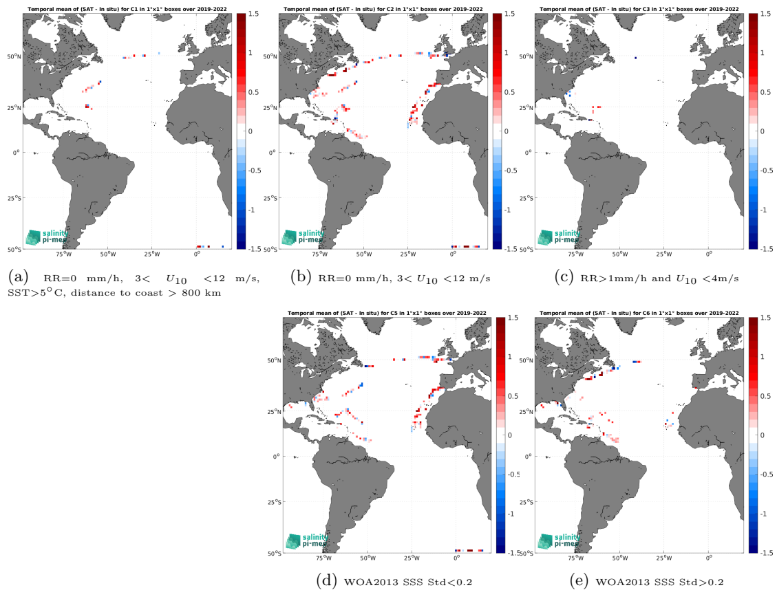
Figure 14: Temporal mean gridded over spatial boxes of size 1^\circ \times 1^\circ of \Delta\text{SSS} (SMAP SSS L2 v5.0 (JPL) - Saildrone) for 5 different subdatasets corresponding to:RR=0 mm/h, 3 < U_{10} < 12 m/s, SST >5^\circ\text{C} , distance to coast > 800 km (a), RR=0 mm/h, 3 < U_{10} < 12 m/s (b), RR >1 mm/h and U_{10} < 4 m/s (c), WOA2013 SSS Std <0.2 (d), WOA2013 SSS Std >0.2 (e).
