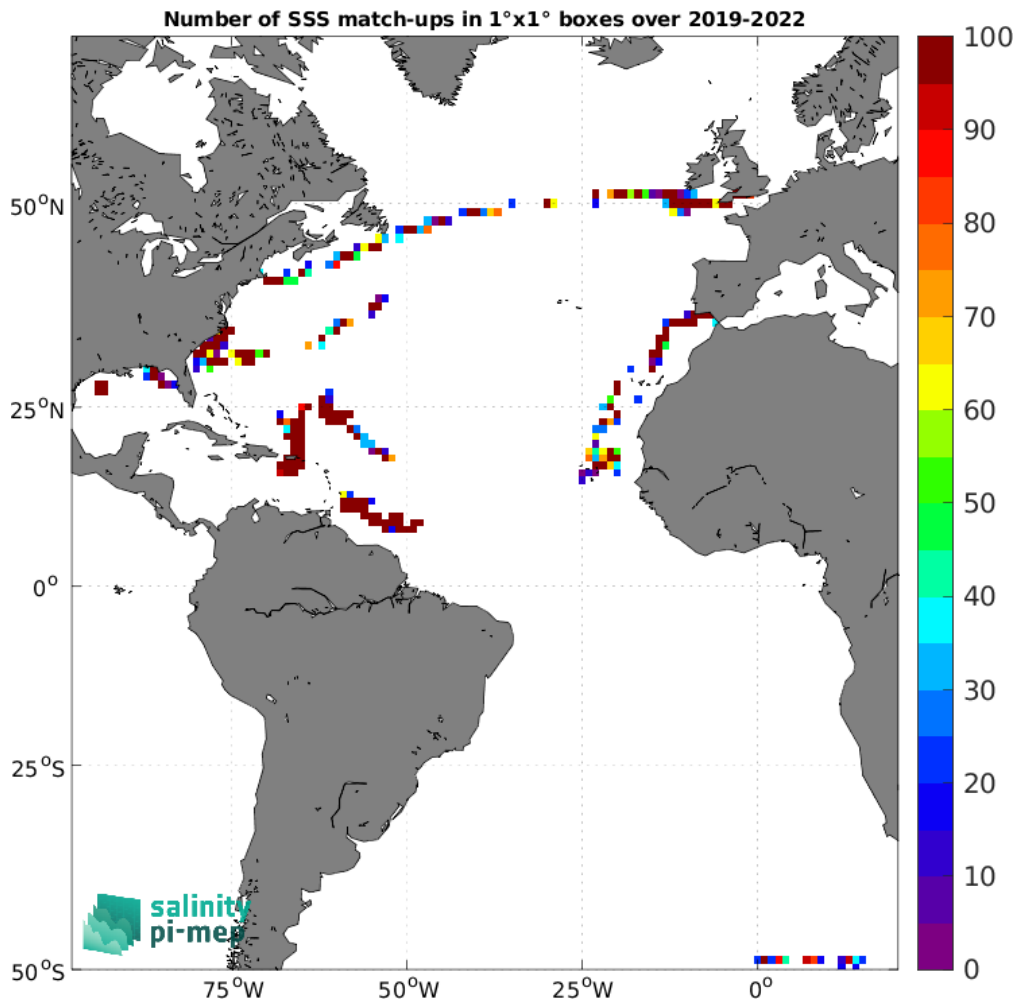
Figure 5: Number of SSS match-ups between Saildrone SSS and the SMAP SSS L2 v5.0 (JPL) SSS product for the Atlantic Ocean Pi-MEP region over 1°×1° boxes and for the full satellite product period.
