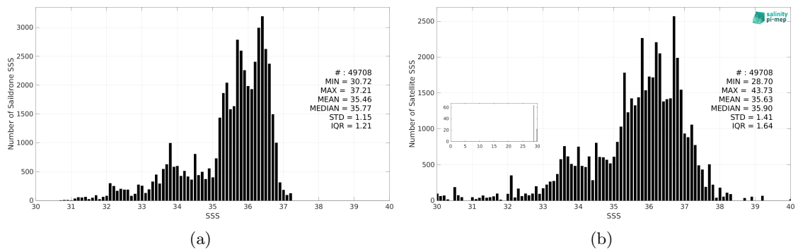
Figure 3: Histograms of SSS from Saildrone (a) and SMAP SSS L2 v5.0 (JPL) (b) considering all match-up pairs per bins of 0.1 over the Atlantic Ocean Pi-MEP region and for the full satellite product period.
