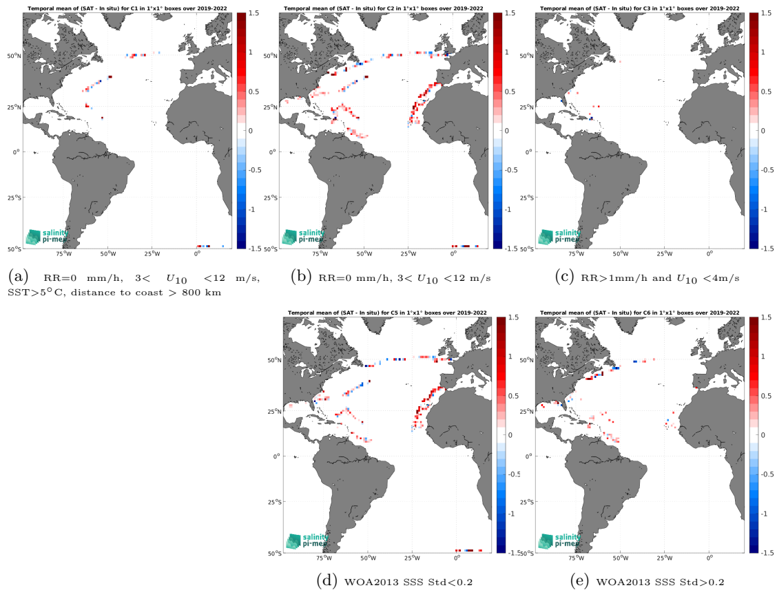
Figure 12: Temporal mean gridded over spatial boxes of size 1^\circ \times 1^\circ of \Delta SSS (SMAP SSS L2 v5.0 (JPL) - Saicdrone) for 5 different subdatasets corresponding to:RR=0 mm/h, 3 < U_{10} < 12 m/s, SST >5^\circ\text{C} , distance to coast > 800 km (a), RR=0 mm/h, 3 < U_{10} < 12 m/s (b), RR >1 mm/h and U_{10} < 4 m/s (c), WOA2013 SSS Std <0.2 (d), WOA2013 SSS Std >0.2 (e).
