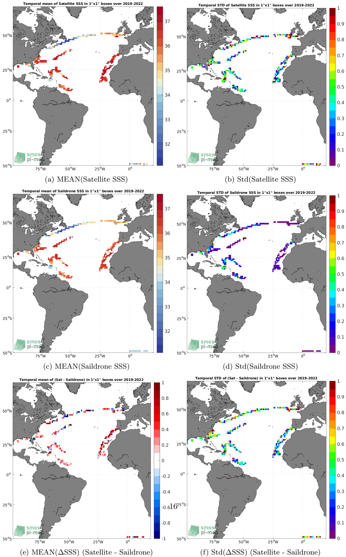
Figure 6: Temporal mean (left) and Std (right) of SSS from SMAP SSS L2 v5.0 (JPL) (top), Saildrone (middle), and of \Delta SSS (Satellite - Saildrone). Only match-up pairs are used to generate these maps.
