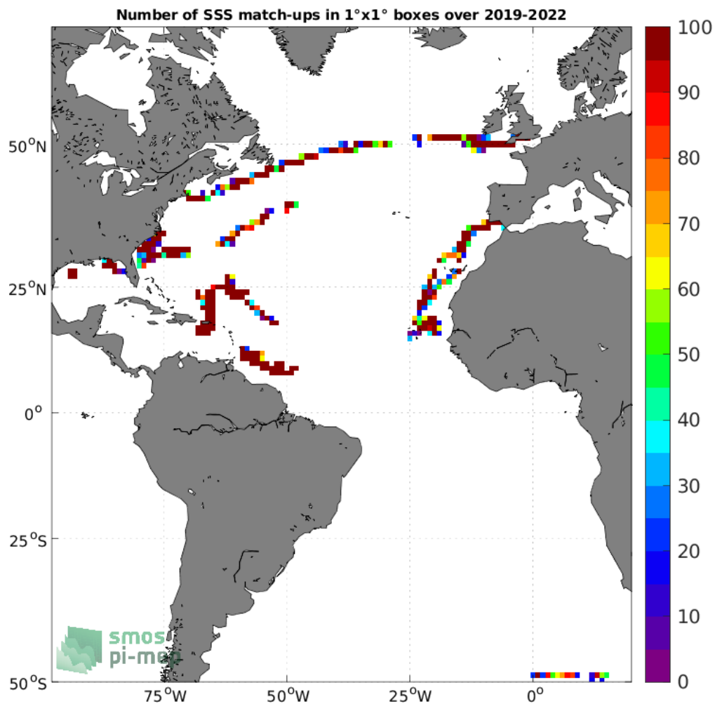
Figure 4: Number of SSS match-ups between Saildrone SSS and the SMAP SSS L2 v5.0 (JPL) SSS product for the Atlantic Ocean Pi-MEP region over 1°×1° boxes and for the full satellite product period.
