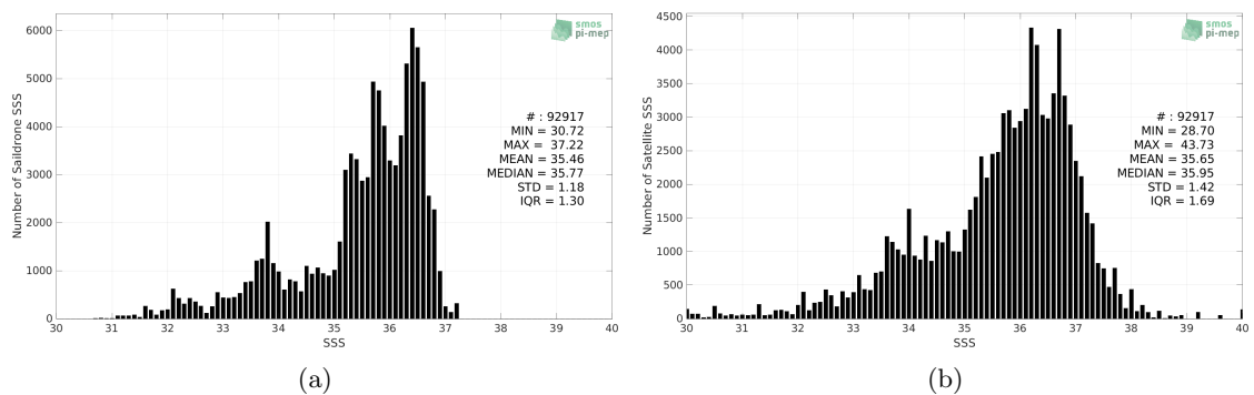
Figure 2: Histograms of SSS from Saildrone (a) and SMAP SSS L2 v5.0 (JPL) (b) considering all match-up pairs per bins of 0.1 over the Atlantic Ocean Pi-MEP region and for the full satellite product period.
