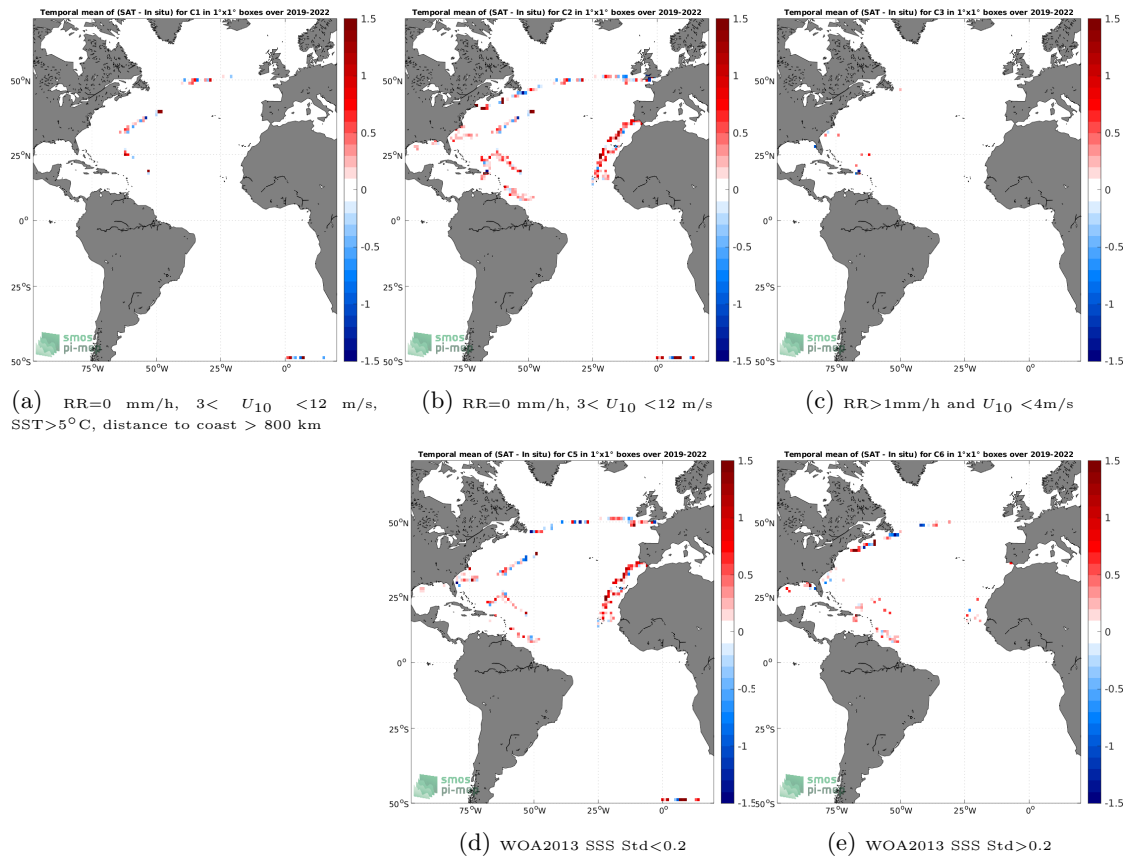
Figure 12: Temporal mean gridded over spatial boxes of size 1^\circ \times 1^\circ of \Delta SSS (SMAP SSS L2 v5.0 (JPL) - Saildrone) for 5 different subdatasets corresponding to:RR=0 mm/h, 3 < U_{10} < 12 m/s, SST >5^\circ\text{C} , distance to coast > 800 km (a), RR=0 mm/h, 3 < U_{10} < 12 m/s (b), RR >1 mm/h and U_{10} < 4 m/s (c), WOA2013 SSS Std <0.2 (d), WOA2013 SSS Std >0.2 (e).
