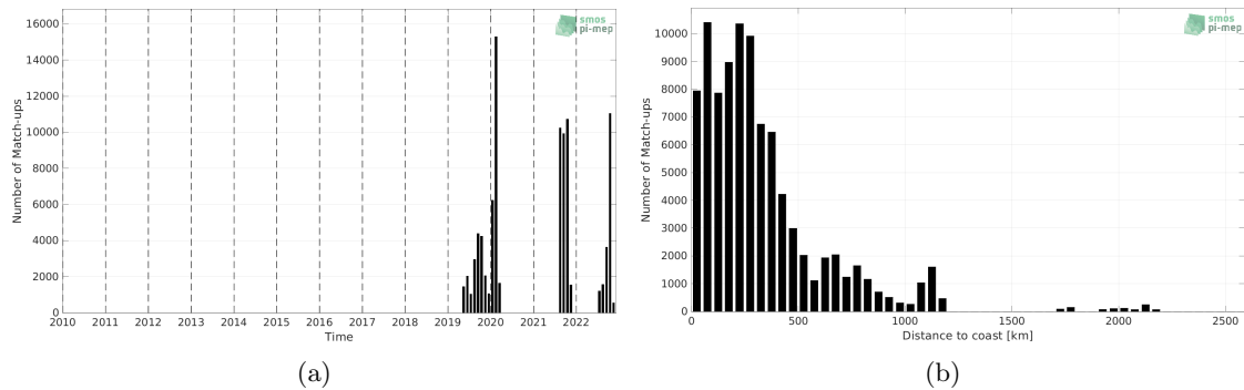
Figure 1: Number of match-ups between Saildrone and SMAP SSS L2 v5.0 (JPL) SSS as a function of time (a) and as function of the distance to coast (b) over the Atlantic Ocean Pi-MEP region and for the full satellite product period.
