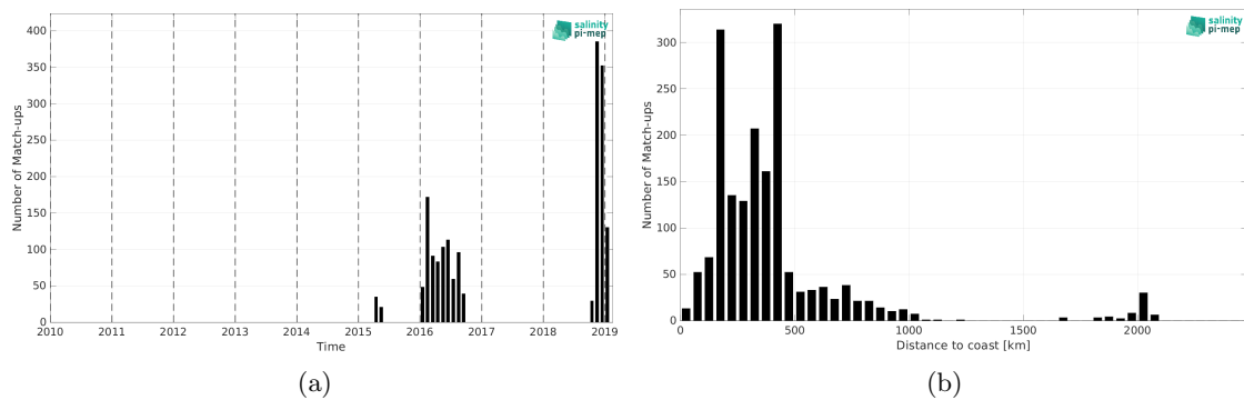
Figure 1: Number of match-ups between Marine mammals and SMAP SSS L2 v5.0 (JPL) SSS as a function of time (a) and as function of the distance to coast (b) over the Atlantic Ocean Pi-MEP region and for the full satellite product period.
