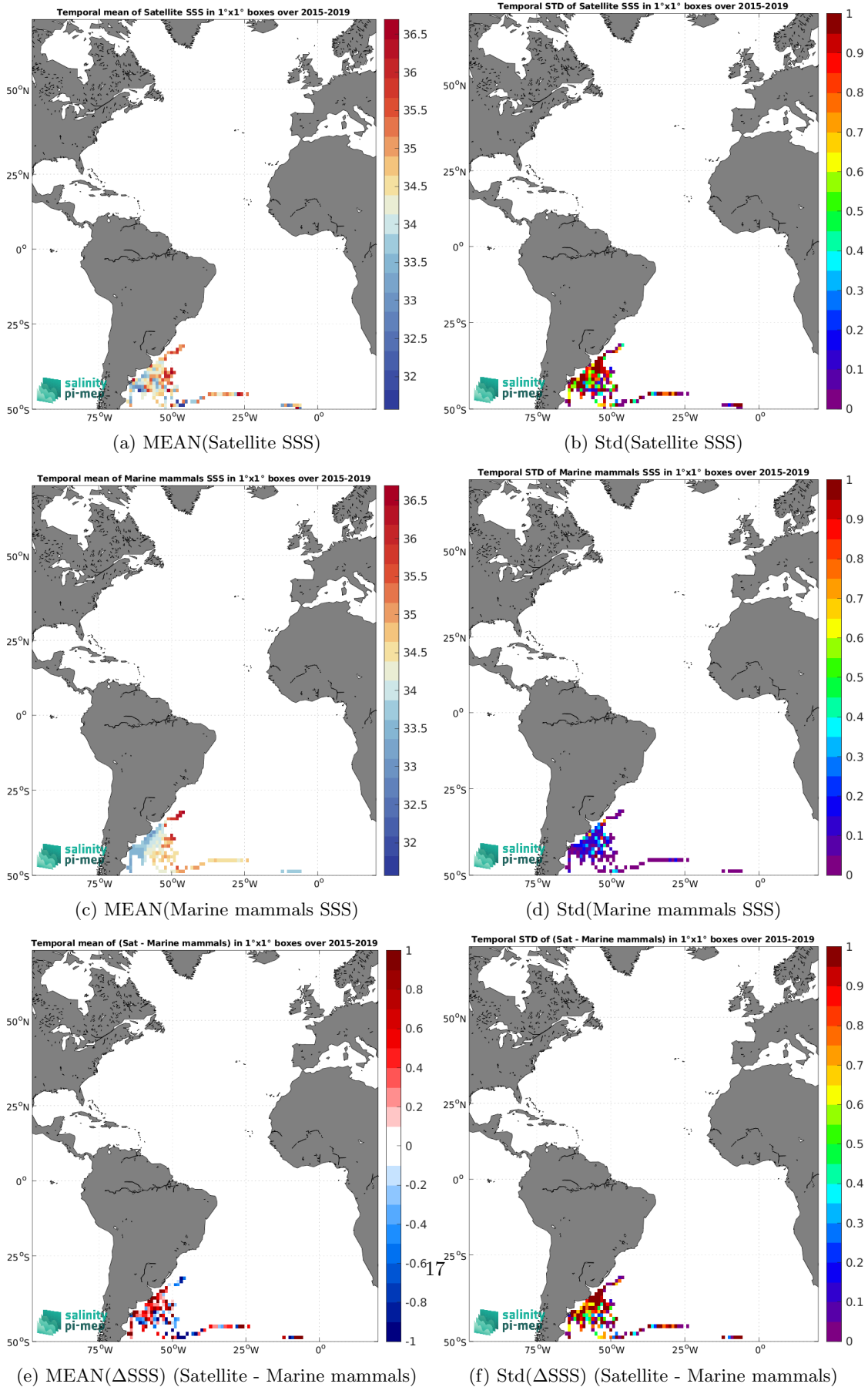
Figure 6: Temporal mean (left) and Std (right) of SSS from SMAP SSS L2 v5.0 (JPL) (top), Marine mammals (middle), and of \Delta SSS (Satellite - Marine mammals). Only match-up pairs are used to generate these maps.
