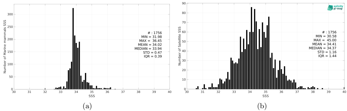
Figure 2: Histograms of SSS from Marine mammals (a) and SMAP SSS L2 v5.0 (JPL) (b) considering all match-up pairs per bins of 0.1 over the Atlantic Ocean Pi-MEP region and for the full satellite product period.
