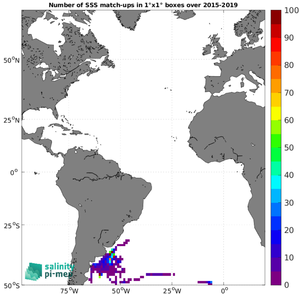
Figure 4: Number of SSS match-ups between Marine mammals SSS and the SMAP SSS L2 v5.0 (JPL) SSS product for the Atlantic Ocean Pi-MEP region over 1^\circ \times 1^\circ boxes and for the full satellite product period.
