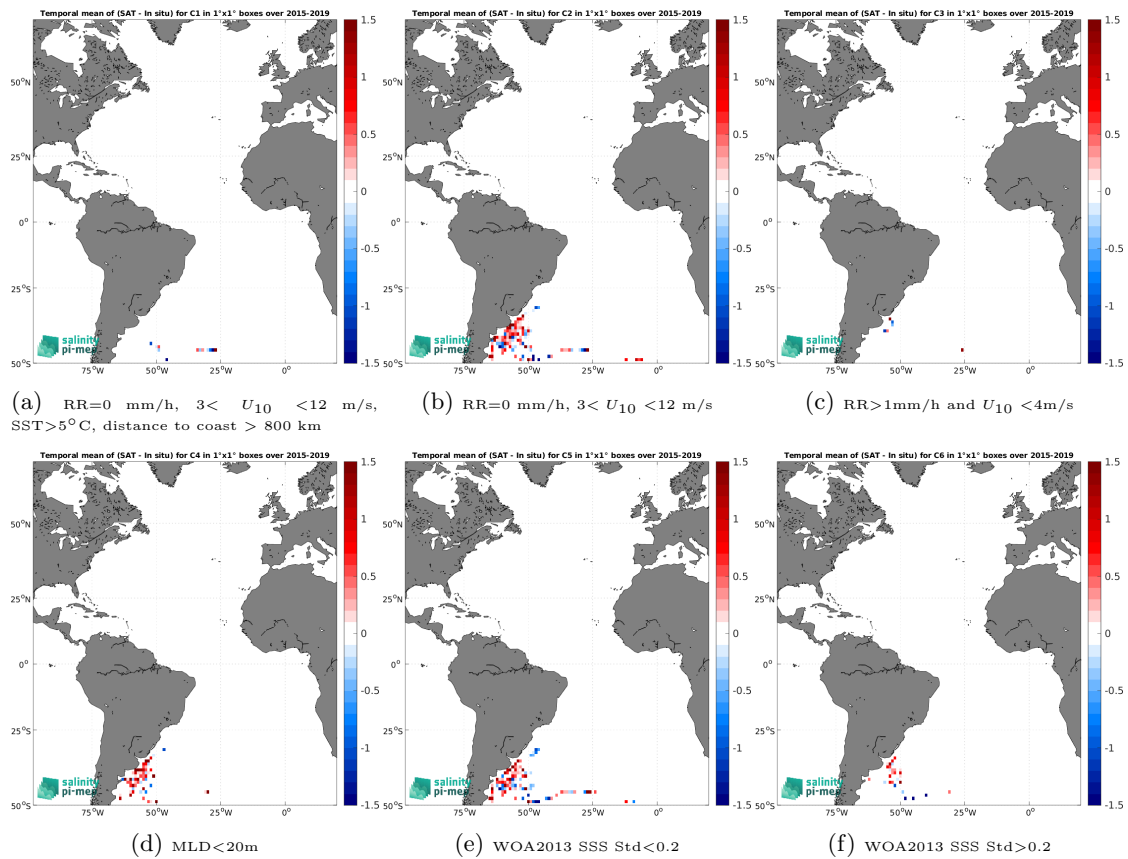
Figure 12: Temporal mean gridded over spatial boxes of size 1^\circ \times 1^\circ of \Delta SSS (SMAP SSS L2 v5.0 (JPL) - Marine mammals) for 6 different subdatasets corresponding to:RR=0 mm/h, 3 < U_{10} < 12 m/s, SST >5^\circ C, distance to coast > 800 km (a), RR=0 mm/h, 3 < U_{10} < 12 m/s (b), RR >1 mm/h and U_{10} < 4 m/s (c),MLD <20 m (d),WOA2013 SSS Std <0.2 (e),WOA2013 SSS Std >0.2 (f).
