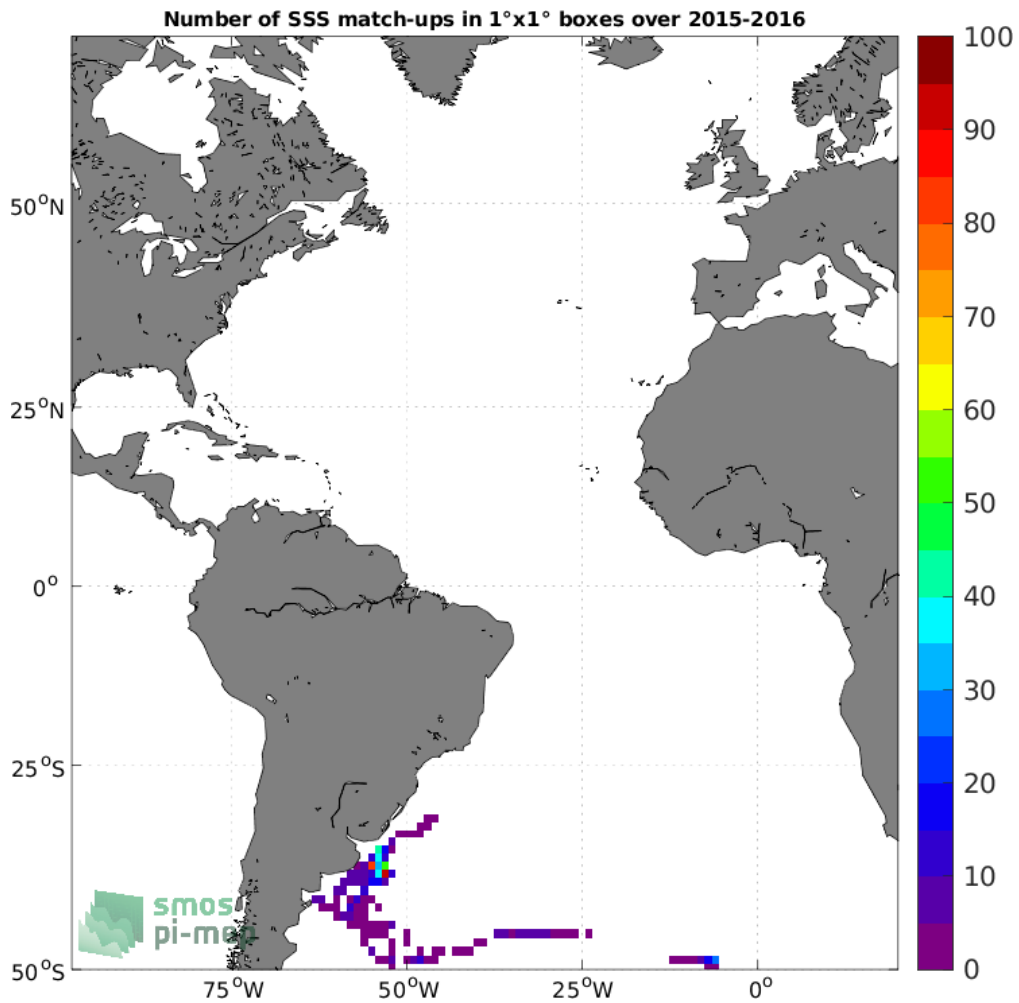
Figure 4: Number of SSS match-ups between Marine mammals SSS and the SMAP SSS L2 v5.0 (JPL) SSS product for the Atlantic Ocean Pi-MEP region over 1°x1° boxes and for the full satellite product period.
