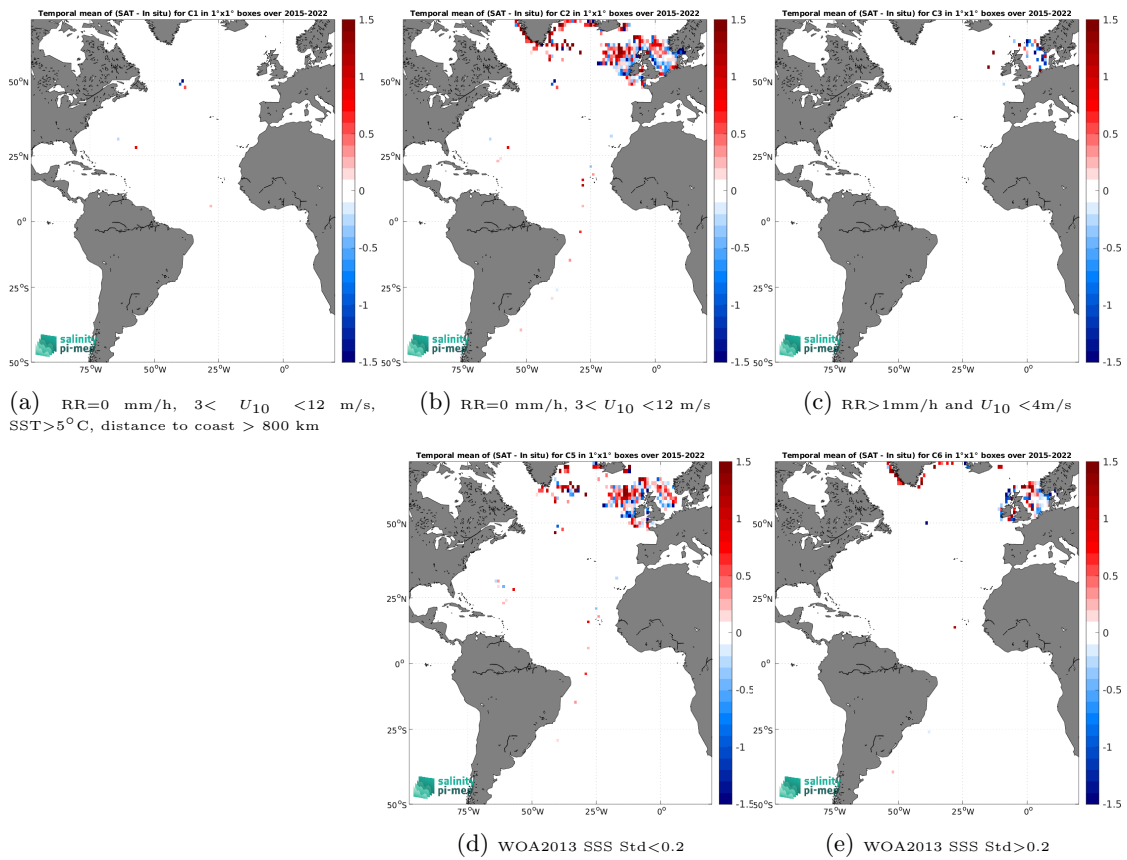
Figure 14: Temporal mean gridded over spatial boxes of size 1^\circ \times 1^\circ of \Delta SSS (SMAP SSS L2 v5.0 (JPL) - ICES) for 5 different subdatasets corresponding to:RR=0 mm/h, 3 < U_{10} < 12 m/s, SST>5°C, distance to coast > 800 km (a), RR=0 mm/h, 3 < U_{10} < 12 m/s (b), RR>1mm/h and U_{10} < 4 m/s (c), WOA2013 SSS Std<0.2 (d), WOA2013 SSS Std>0.2 (e).
