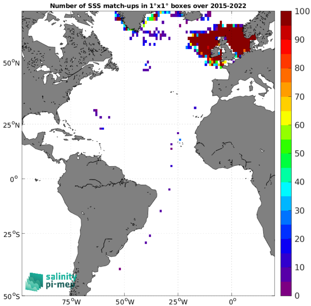
Figure 5: Number of SSS match-ups between ICES SSS and the SMAP SSS L2 v5.0 (JPL) SSS product for the Atlantic Ocean Pi-MEP region over 1°×1° boxes and for the full satellite product period.
