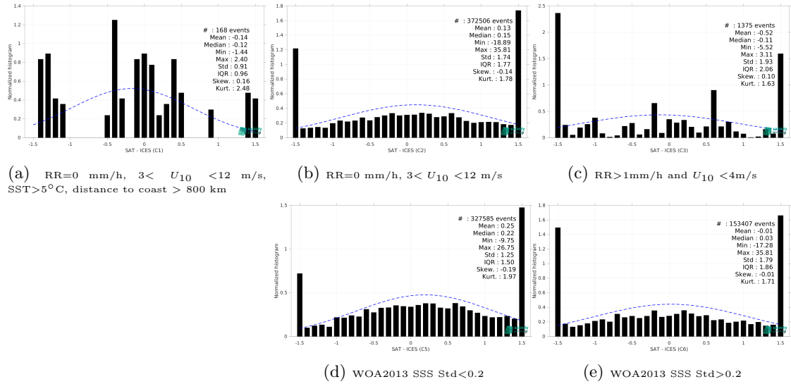
Figure 13: Normalized histogram of \Delta SSS (SMAP SSS L2 v5.0 (JPL) - ICES) for 5 different subdatasets corresponding to: RR=0 mm/h, 3 < U_{10} < 12 m/s, SST > 5°C, distance to coast > 800 km (a), RR=0 mm/h, 3 < U_{10} < 12 m/s (b), RR > 1mm/h and U_{10} < 4 m/s (c), WOA2013 SSS Std < 0.2 (d), WOA2013 SSS Std > 0.2 (e).
