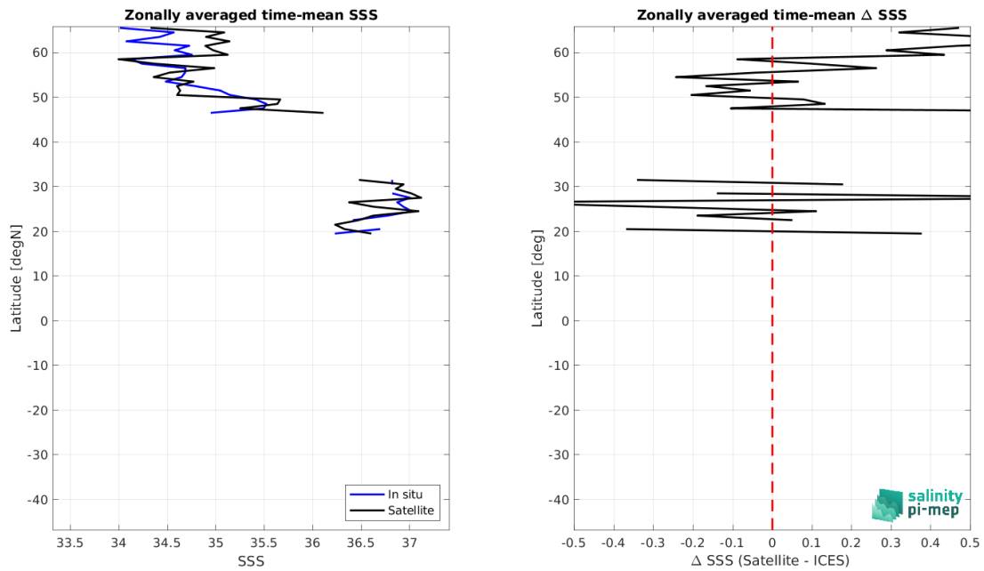
Figure 8: Left panel: Zonal mean SSS from SMAP SSS L2 v5.0 (JPL) satellite product (black) and from ICES (blue). Right panel: Zonal mean of \Delta SSS (Satellite - ICES) for all the collected Pi-MEP match-up pairs estimated over the full satellite product period.
