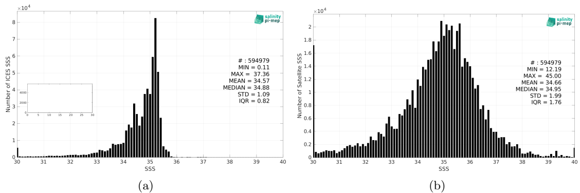
Figure 2: Histograms of SSS from ICES (a) and SMAP SSS L2 v5.0 (JPL) (b) considering all match-up pairs per bins of 0.1 over the Atlantic Ocean Pi-MEP region and for the full satellite product period.
