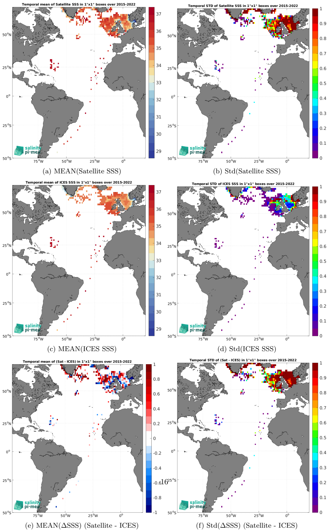
Figure 6: Temporal mean (left) and Std (right) of SSS from SMAP SSS L2 v5.0 (JPL) (top), ICES (middle), and of \Delta SSS (Satellite - ICES). Only match-up pairs are used to generate these maps.
