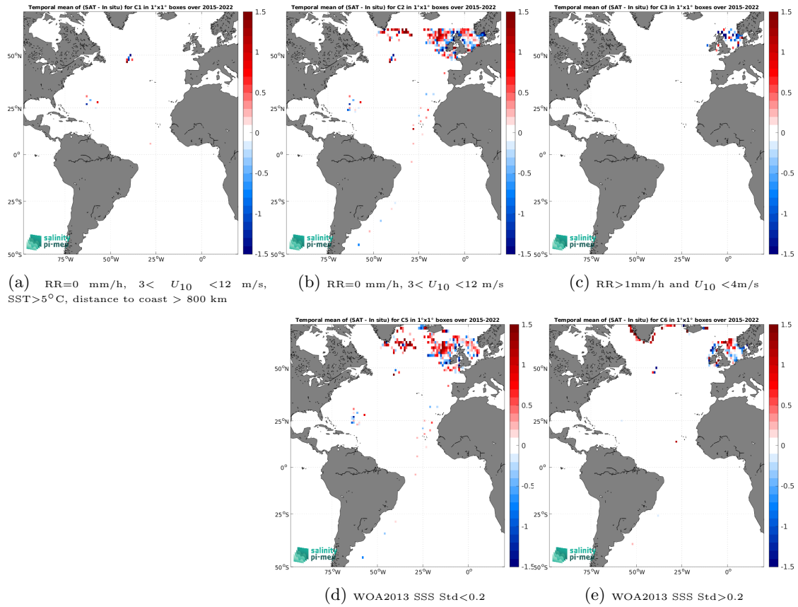
Figure 12: Temporal mean gridded over spatial boxes of size 1^\circ \times 1^\circ of \Delta SSS (SMAP SSS L2 v5.0 (JPL) - ICES) for 5 different subdatasets corresponding to:RR=0 mm/h, 3 < U_{10} < 12 m/s, SST>5°C, distance to coast > 800 km (a), RR=0 mm/h, 3 < U_{10} < 12 m/s (b), RR>1mm/h and U_{10} < 4 m/s (c), WOA2013 SSS Std<0.2 (d), WOA2013 SSS Std>0.2 (e).
