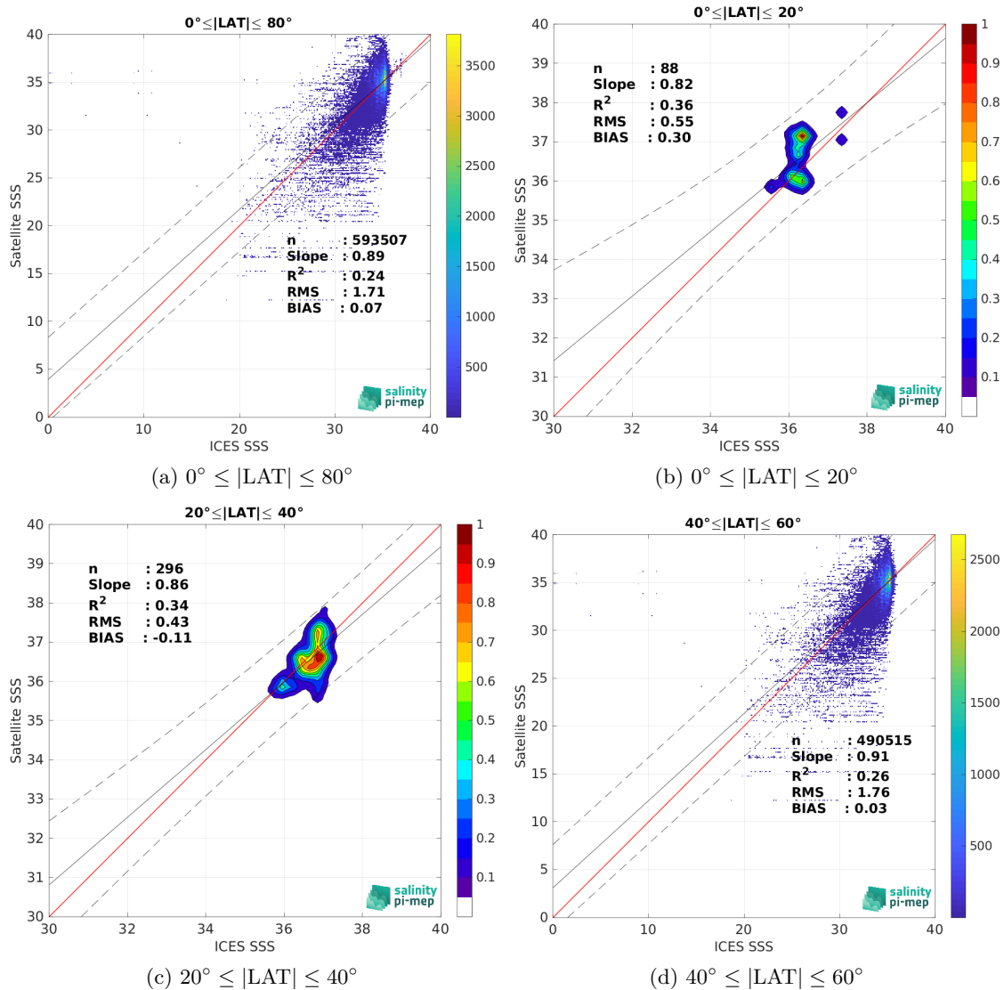
Figure 9: Contour maps of the concentration of SMAP SSS L2 v5.0 (JPL) SSS (y-axis) versus ICES SSS (x-axis) at match-up pairs for different latitude bands. For each plot, the red line shows x=y . The black thin and dashed lines indicate a linear fit through the data cloud and the \pm 95\% confidence levels, respectively. The number match-up pairs n , the slope and R^2 coefficient of the linear fit, the root mean square (RMS) and the mean bias between satellite and in situ data are indicated for each latitude band in each plots.
