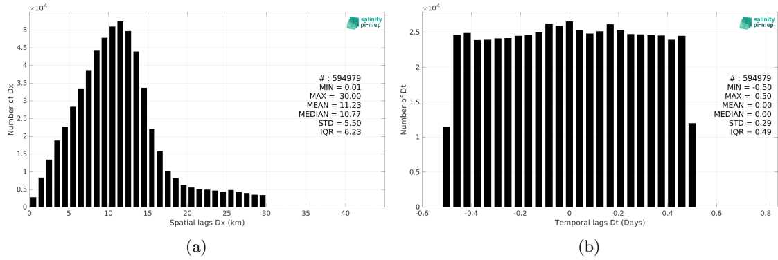
Figure 5: Histograms of the spatial (a) and temporal (b) lags between the location/time of the ICES measurement and the date of the corresponding SMAP SSS L2 v5.0 (JPL) SSS pixel.
