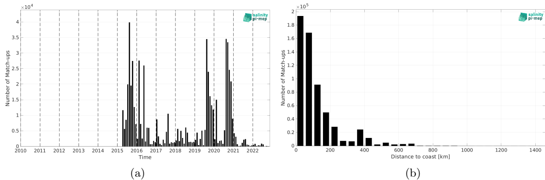
Figure 1: Number of match-ups between ICES and SMAP SSS L2 v5.0 (JPL) SSS as a function of time (a) and as function of the distance to coast (b) over the Atlantic Ocean Pi-MEP region and for the full satellite product period.
