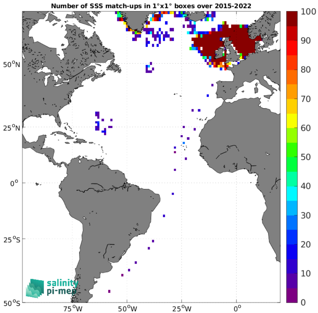
Figure 4: Number of SSS match-ups between ICES SSS and the SMAP SSS L2 v5.0 (JPL) SSS product for the Atlantic Ocean Pi-MEP region over 1^{\circ} \times 1^{\circ} boxes and for the full satellite product period.
