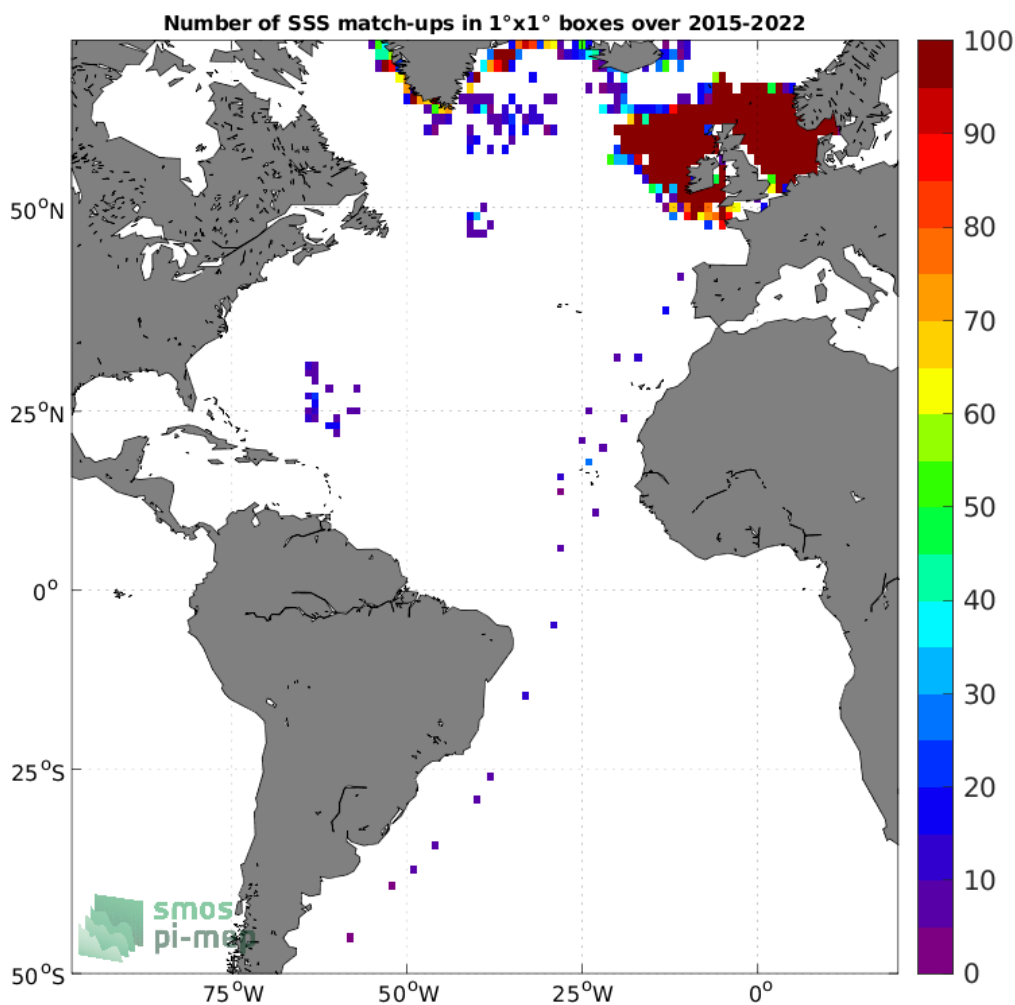
Figure 4: Number of SSS match-ups between ICES SSS and the SMAP SSS L2 v5.0 (JPL) SSS product for the Atlantic Ocean Pi-MEP region over 1°x1° boxes and for the full satellite product period.
