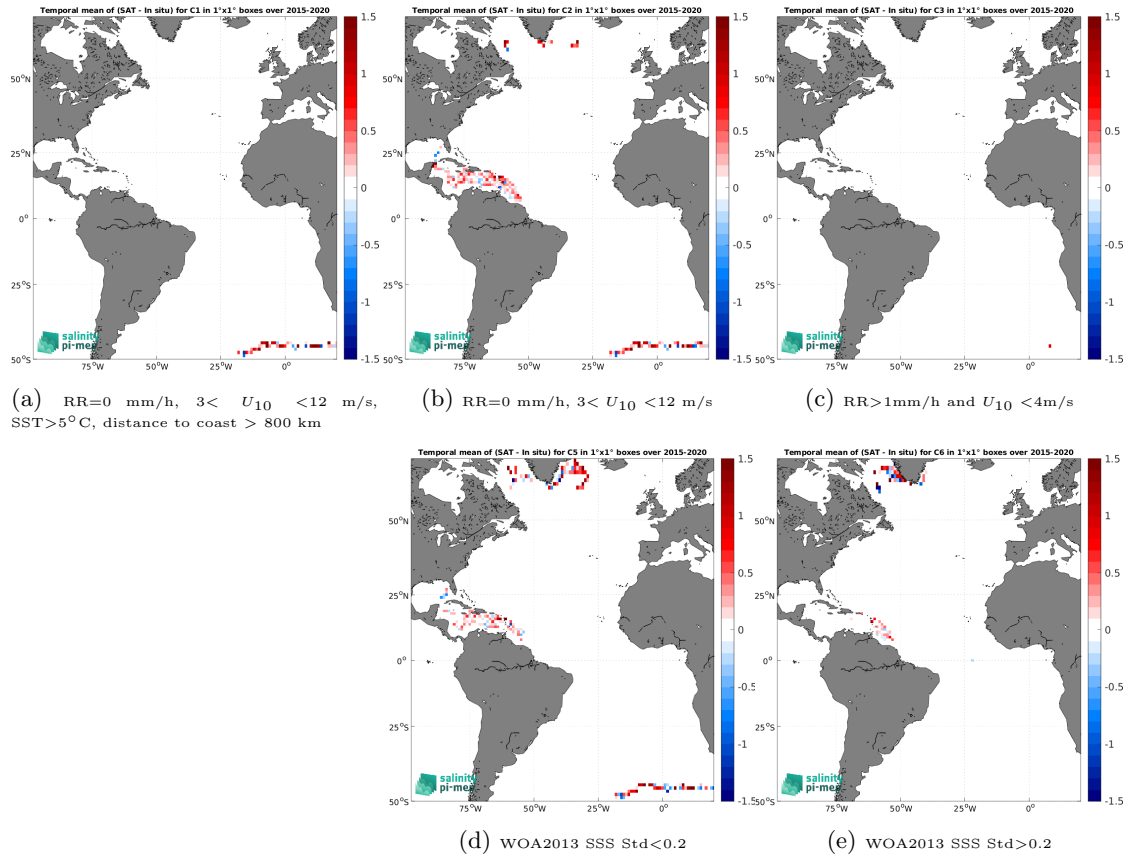
Figure 11: Temporal mean gridded over spatial boxes of size 1^\circ \times 1^\circ of \Delta\text{SSS} (SMAP SSS L2 v5.0 (JPL) - Surface drifters) for 5 different subdatasets corresponding to:RR=0 mm/h, 3 < U_{10} < 12 m/s, SST >5^\circ\text{C} , distance to coast > 800 km (a), RR=0 mm/h, 3 < U_{10} < 12 m/s (b), RR >1 mm/h and U_{10} < 4 m/s (c), WOA2013 SSS Std <0.2 (d), WOA2013 SSS Std >0.2 (e).
