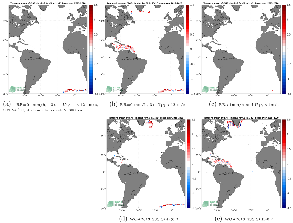
Figure 11: Temporal mean gridded over spatial boxes of size 1^\circ \times 1^\circ of \Delta SSS (SMAP SSS L2 v5.0 (JPL) - Surface drifters) for 5 different subdatasets corresponding to:RR=0 mm/h, 3 < U_{10} < 12 m/s, SST >5^\circ\text{C} , distance to coast > 800 km (a), RR=0 mm/h, 3 < U_{10} < 12 m/s (b), RR >1 mm/h and U_{10} < 4 m/s (c), WOA2013 SSS Std <0.2 (d), WOA2013 SSS Std >0.2 (e).
