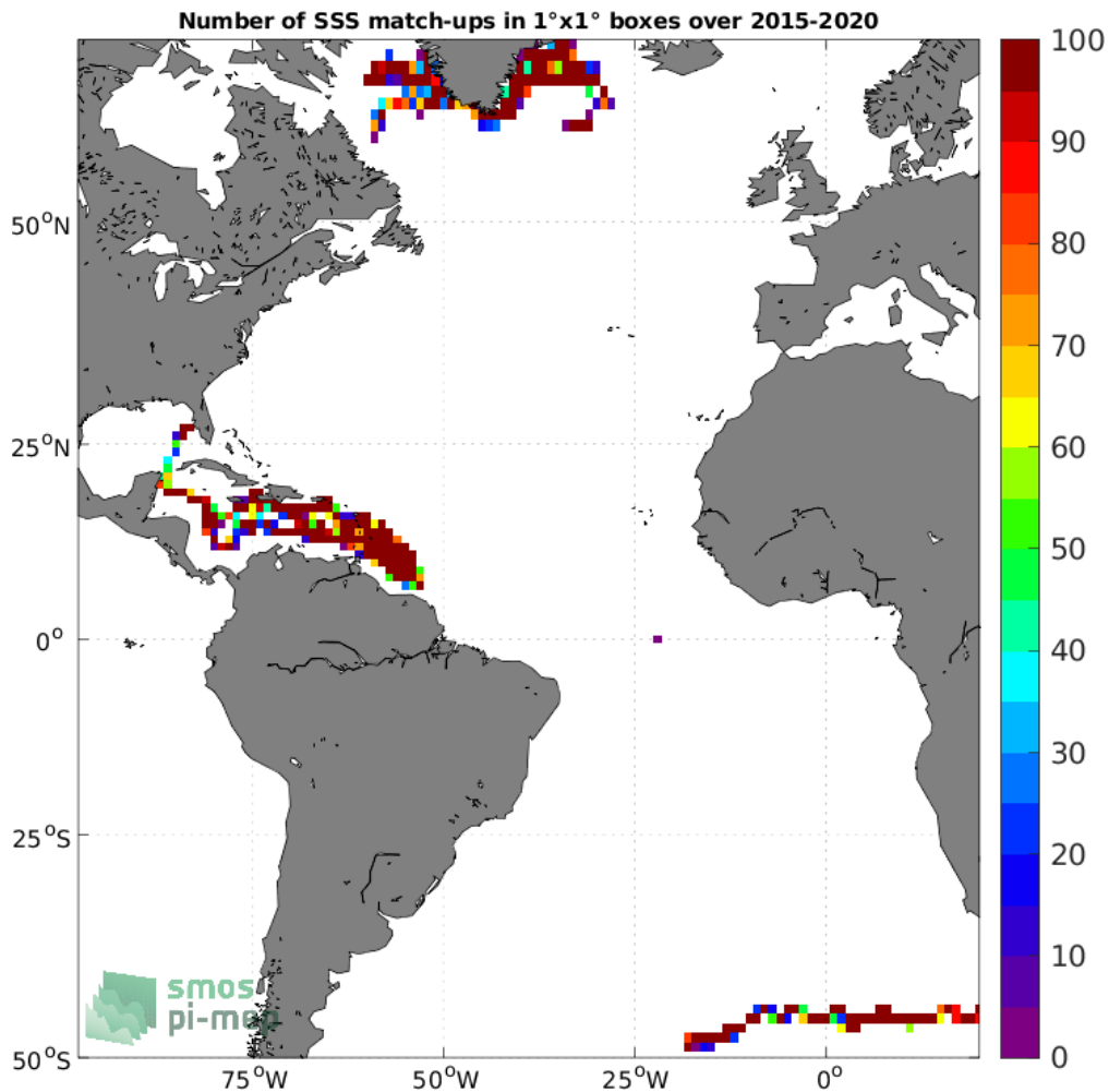
Figure 3: Number of SSS match-ups between Surface drifters SSS and the SMAP SSS L2 v5.0 (JPL) SSS product for the Atlantic Ocean Pi-MEP region over 1°x1° boxes and for the full satellite product period.
