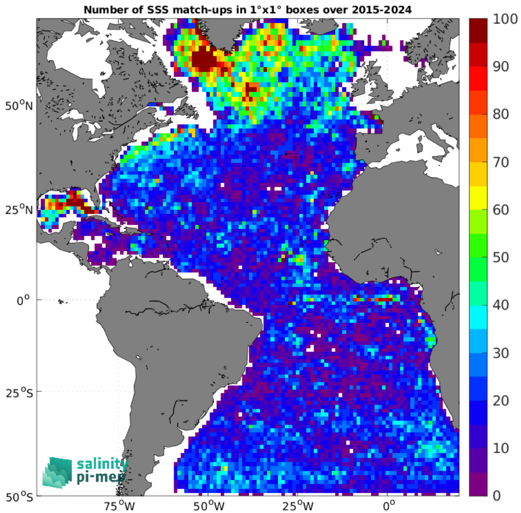
Figure 5: Number of SSS match-ups between Argo SSS and the SMAP SSS L2 v5.0 (JPL) SSS product for the Atlantic Ocean Pi-MEP region over 1^\circ \times 1^\circ boxes and for the full satellite product period.
