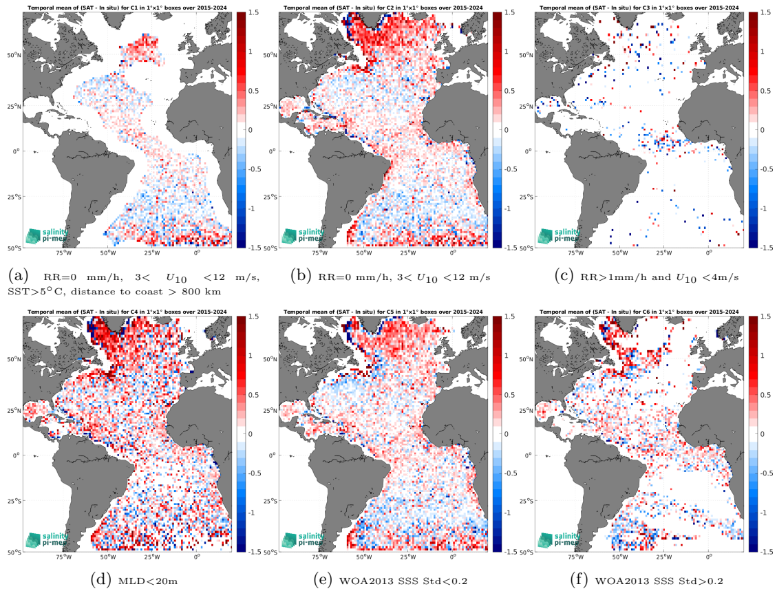
Figure 14: Temporal mean gridded over spatial boxes of size 1^\circ \times 1^\circ of \Delta SSS (SMAP SSS L2 v5.0 (JPL) - Argo) for 6 different subdatasets corresponding to:RR=0 mm/h, 3 < U_{10} < 12 m/s, SST>5°C, distance to coast > 800 km (a), RR=0 mm/h, 3 < U_{10} < 12 m/s (b), RR>1mm/h and U_{10} < 4 m/s (c),MLD<20m (d),WOA2013 SSS Std<0.2 (e),WOA2013 SSS Std>0.2 (f).
