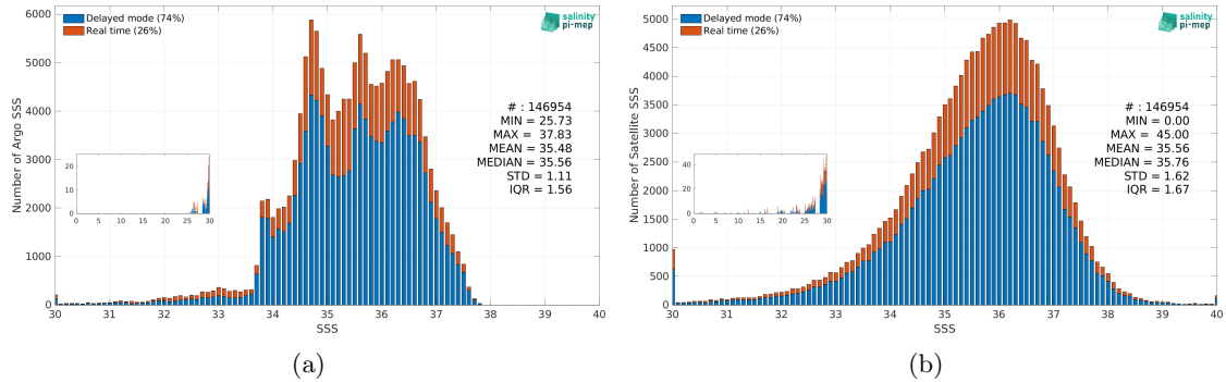
Figure 3: Histograms of SSS from Argo (a) and SMAP SSS L2 v5.0 (JPL) (b) considering all match-up pairs per bins of 0.1 over the Atlantic Ocean Pi-MEP region and for the full satellite product period.
