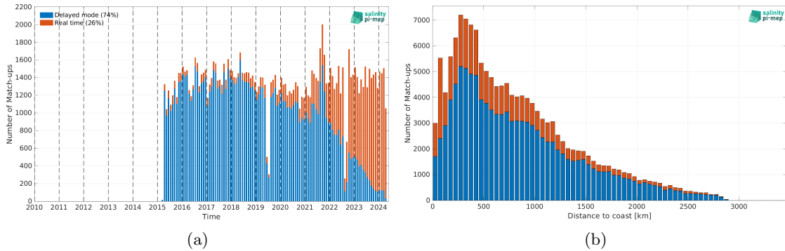
Figure 2: Number of match-ups between Argo and SMAP SSS L2 v5.0 (JPL) SSS as a function of time (a) and as function of the distance to coast (b) over the Atlantic Ocean Pi-MEP region and for the full satellite product period.
