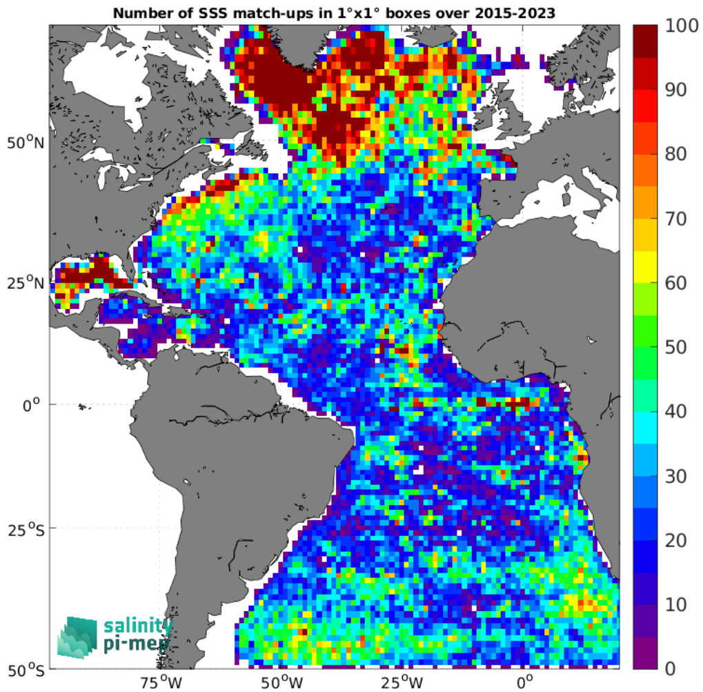
Figure 4: Number of SSS match-ups between Argo SSS and the SMAP SSS L2 v5.0 (JPL) SSS product for the Atlantic Ocean Pi-MEP region over 1^\circ \times 1^\circ boxes and for the full satellite product period.
