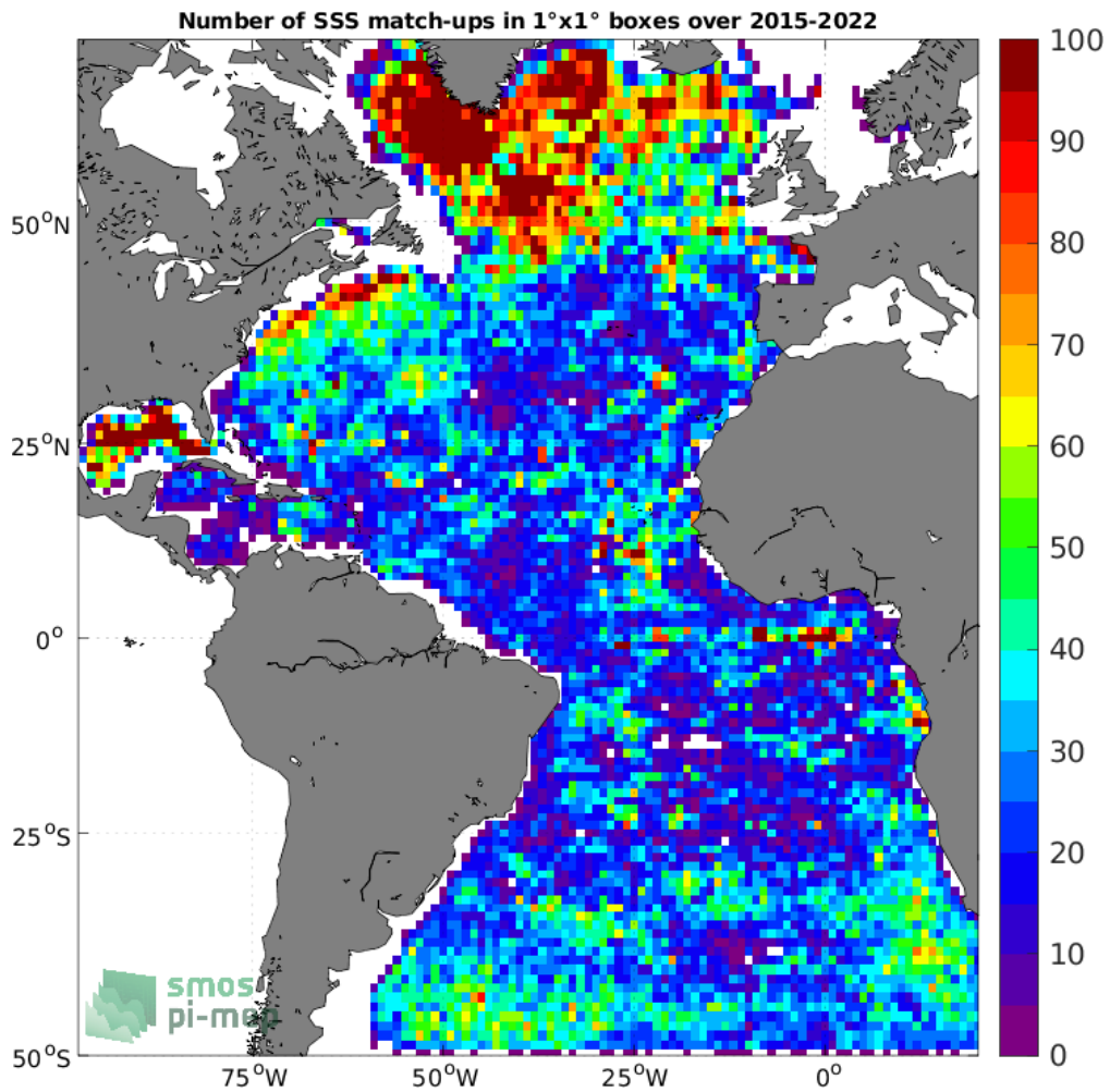
Figure 4: Number of SSS match-ups between Argo SSS and the SMAP SSS L2 v5.0 (JPL) SSS product for the Atlantic Ocean Pi-MEP region over 1°×1° boxes and for the full satellite product period.
