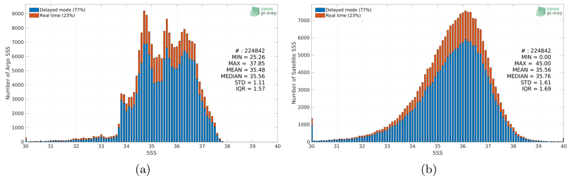
Figure 2: Histograms of SSS from Argo (a) and SMAP SSS L2 v5.0 (JPL) (b) considering all match-up pairs per bins of 0.1 over the Atlantic Ocean Pi-MEP region and for the full satellite product period.
