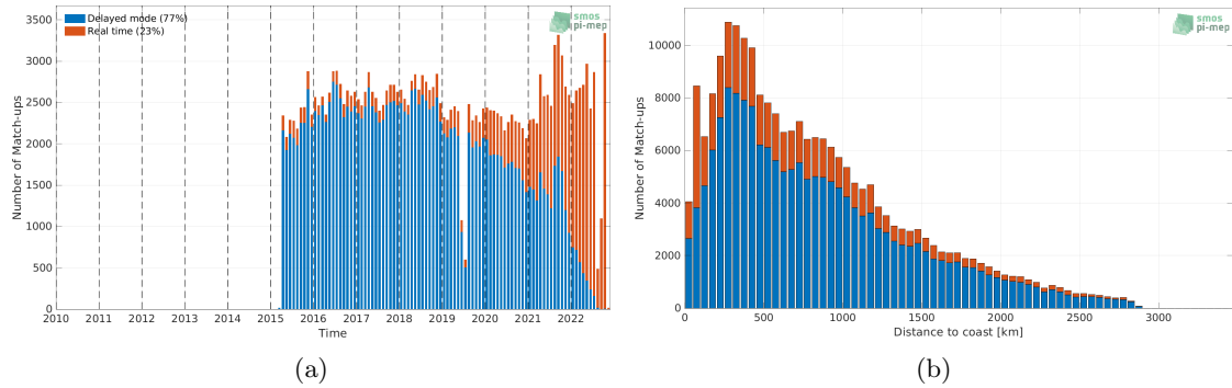
Figure 1: Number of match-ups between Argo and SMAP SSS L2 v5.0 (JPL) SSS as a function of time (a) and as function of the distance to coast (b) over the Atlantic Ocean Pi-MEP region and for the full satellite product period.
