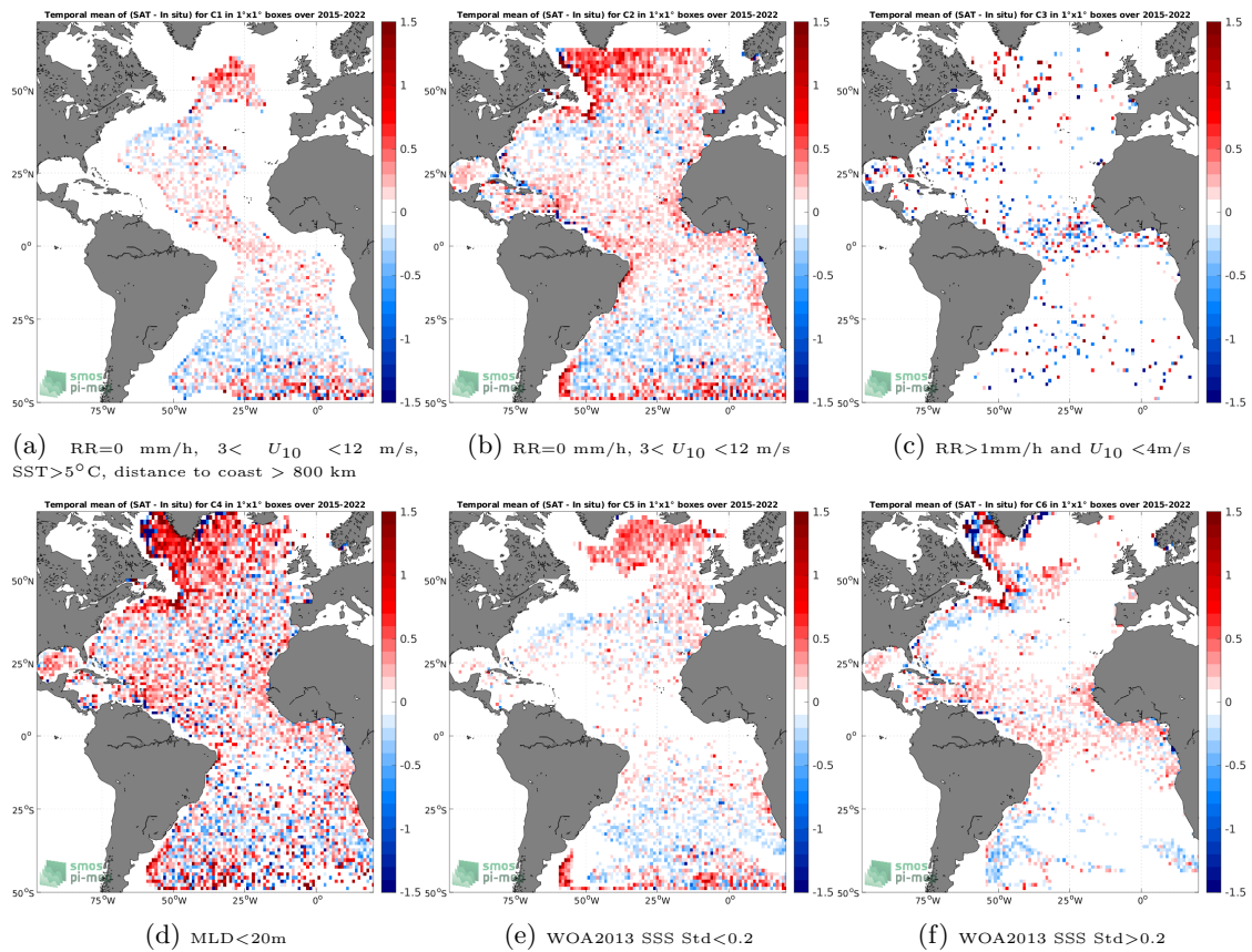
Figure 12: Temporal mean gridded over spatial boxes of size 1^\circ \times 1^\circ of \Delta SSS (SMAP SSS L2 v5.0 (JPL) - Argo) for 6 different subdatasets corresponding to:RR=0 mm/h, 3 < U_{10} < 12 m/s, SST >5^\circ C, distance to coast > 800 km (a), RR=0 mm/h, 3 < U_{10} < 12 m/s (b), RR >1 mm/h and U_{10} < 4 m/s (c),MLD <20 m (d),WOA2013 SSS Std <0.2 (e),WOA2013 SSS Std >0.2 (f).
