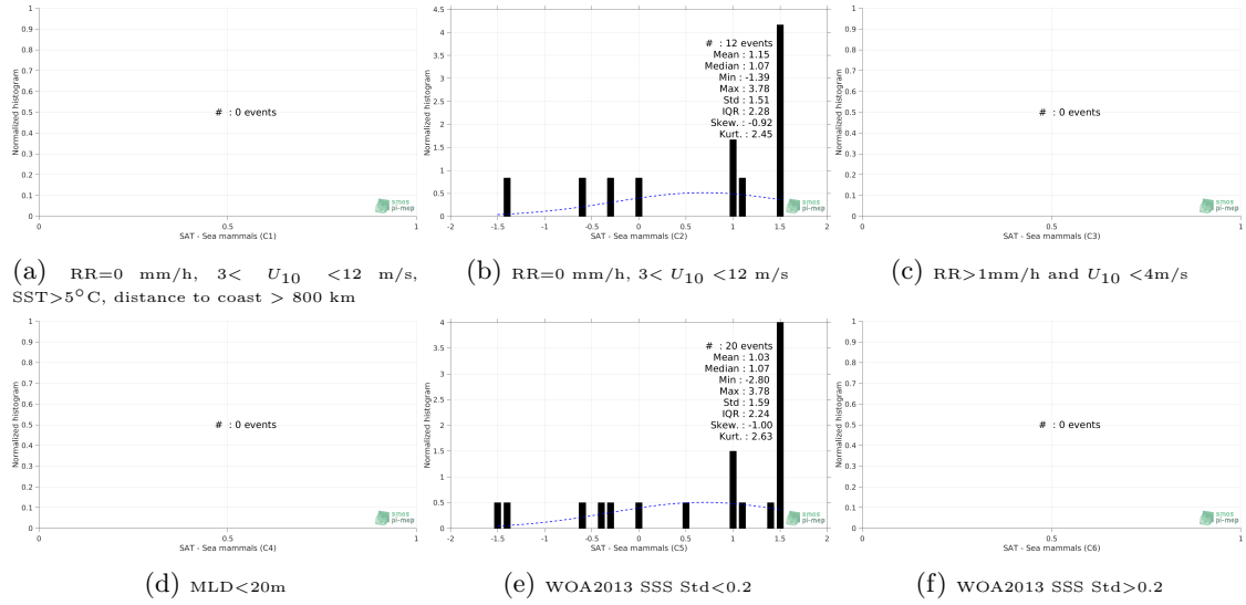
Figure 13: Normalized histogram of \Delta SSS (SMAP-L2-JPL-V4.3 - Sea mammals) for 6 different subdatasets corresponding to: RR=0 mm/h, 3 < U_{10} < 12 m/s, SST>5°C, distance to coast > 800 km (a), RR=0 mm/h, 3 < U_{10} < 12 m/s (b), RR>1mm/h and U_{10} < 4 m/s (c), MLD<20m (d), WOA2013 SSS Std<0.2 (e), WOA2013 SSS Std>0.2 (f).
