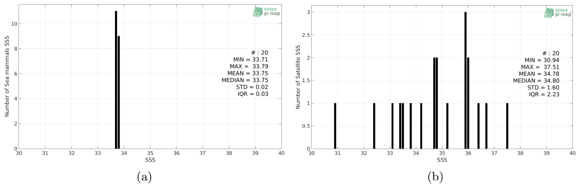
Figure 2: Histograms of SSS from Sea mammals (a) and SMAP-L2-JPL-V4.3 (b) considering all match-up pairs per bins of 0.1 over the Atlantic Ocean Pi-MEP region and for the full satellite product period.
