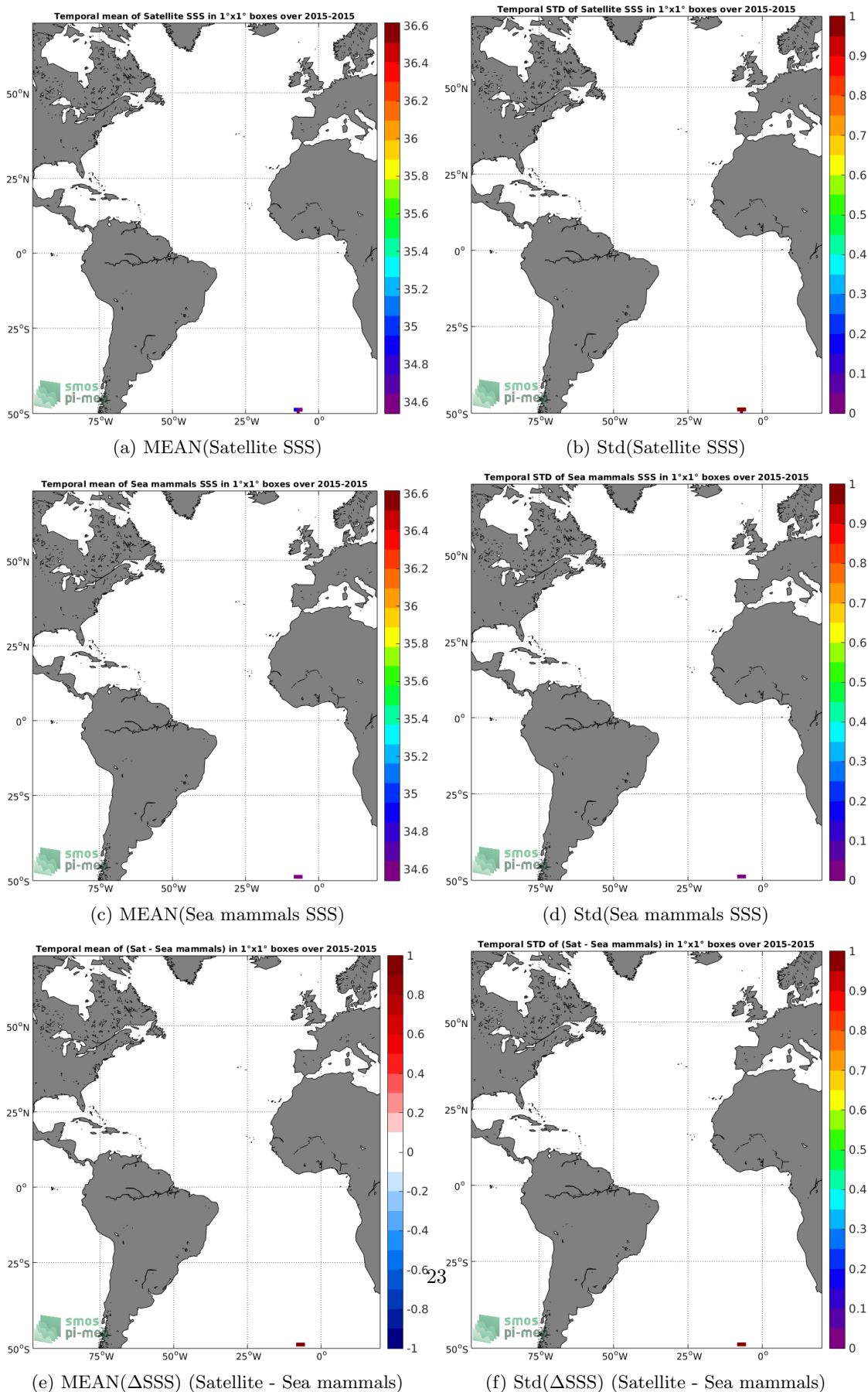
Figure 6: Temporal mean (left) and Std (right) of SSS from SMAP-L2-JPL-V4.3 (top), Sea mammals (middle), and of \Delta SSS (Satellite - Sea mammals). Only match-up pairs are used to generate these maps.
