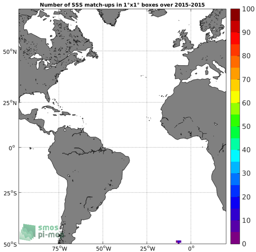
Figure 4: Number of SSS match-ups between Sea mammals SSS and the SMAP-L2-JPL-V4.3 SSS product for the Atlantic Ocean Pi-MEP region over 1°x1° boxes and for the full satellite product period.
