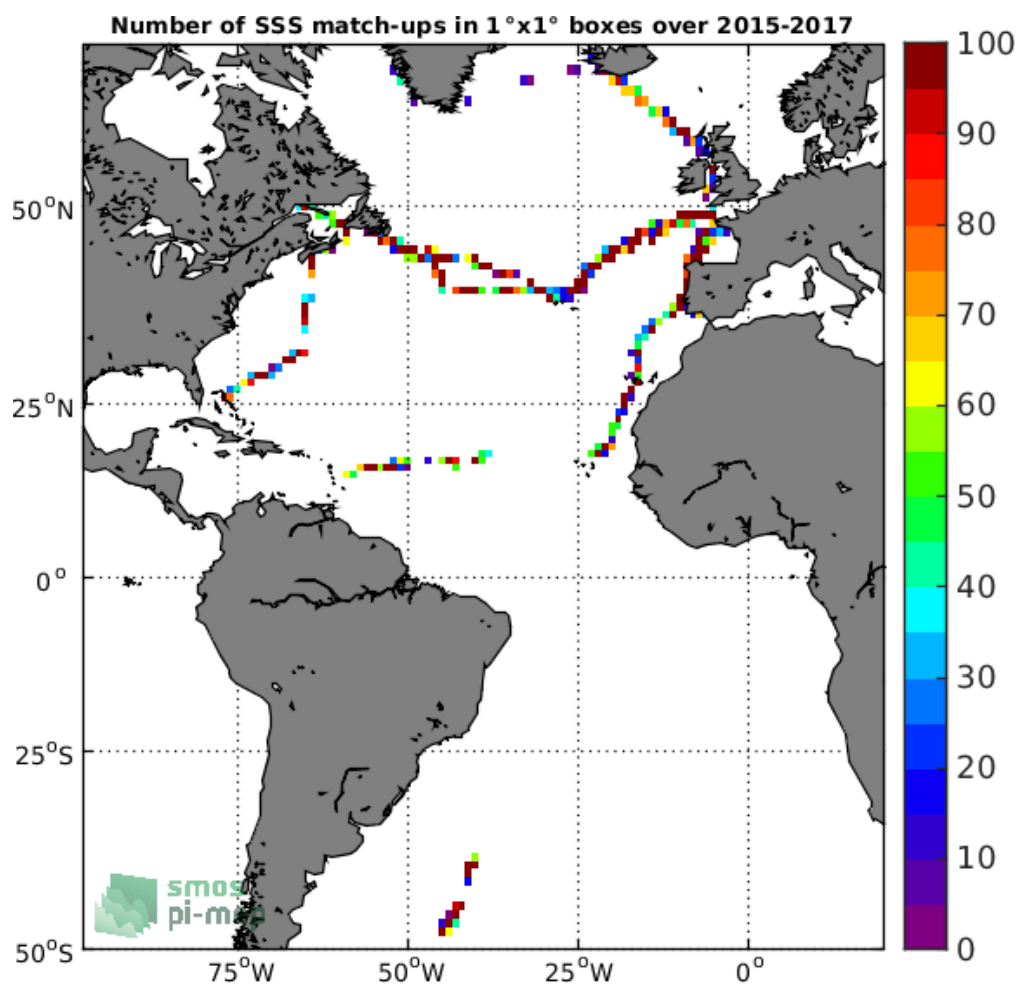
Figure 4: Number of SSS match-ups between TSG-GOSUD-Sailing-ship SSS and the SMAP-L2-JPL-V4.2 SSS product for the Atlantic Ocean Pi-MEP region over 1^\circ \times 1^\circ boxes and for the full satellite product period.
