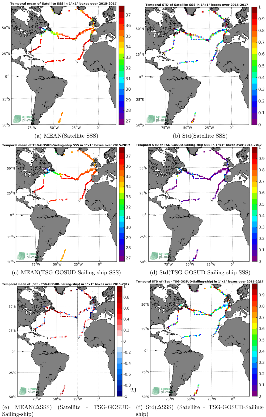
Figure 6: Temporal mean (left) and Std (right) of SSS from SMAP-L2-JPL-V4.2 (top), TSG-GOSUD-Sailing-ship (middle), and of \Delta SSS (Satellite - TSG-GOSUD-Sailing-ship). Only match-up pairs are used to generate these maps.
