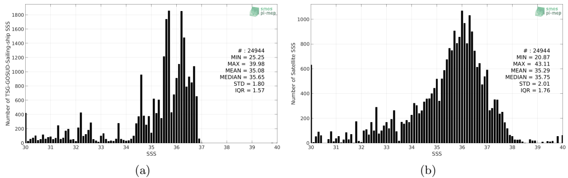
Figure 2: Histograms of SSS from TSG-GOSUD-Sailing-ship (a) and SMAP-L2-JPL-V4.2 (b) considering all match-up pairs per bins of 0.1 over the Atlantic Ocean Pi-MEP region and for the full satellite product period.
