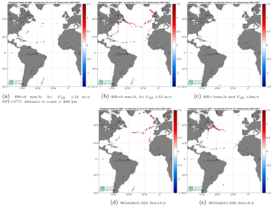
Figure 12: Temporal mean gridded over spatial boxes of size 1^\circ \times 1^\circ of \Delta SSS (SMAP-L2-JPL-V4.2 - TSG-GOSUD-Sailing-ship) for 5 different subdatasets corresponding to:RR=0 mm/h, 3 < U_{10} < 12 m/s, SST>5°C, distance to coast > 800 km (a), RR=0 mm/h, 3 < U_{10} < 12 m/s (b), RR>1mm/h and U_{10} < 4 m/s (c), WOA2013 SSS Std<0.2 (d), WOA2013 SSS Std>0.2 (e).
