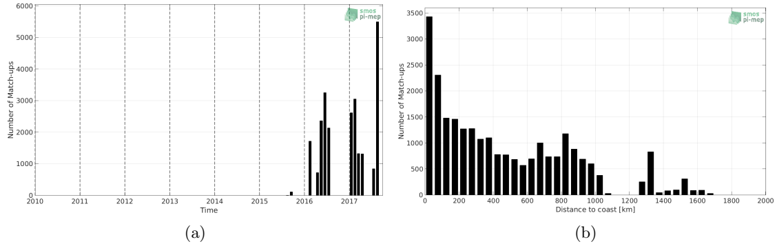
Figure 1: Number of match-ups between TSG-GOSUD-Sailing-ship and SMAP-L2-JPL-V4.2 SSS as a function of time (a) and as function of the distance to coast (b) over the Atlantic Ocean Pi-MEP region and for the full satellite product period.
