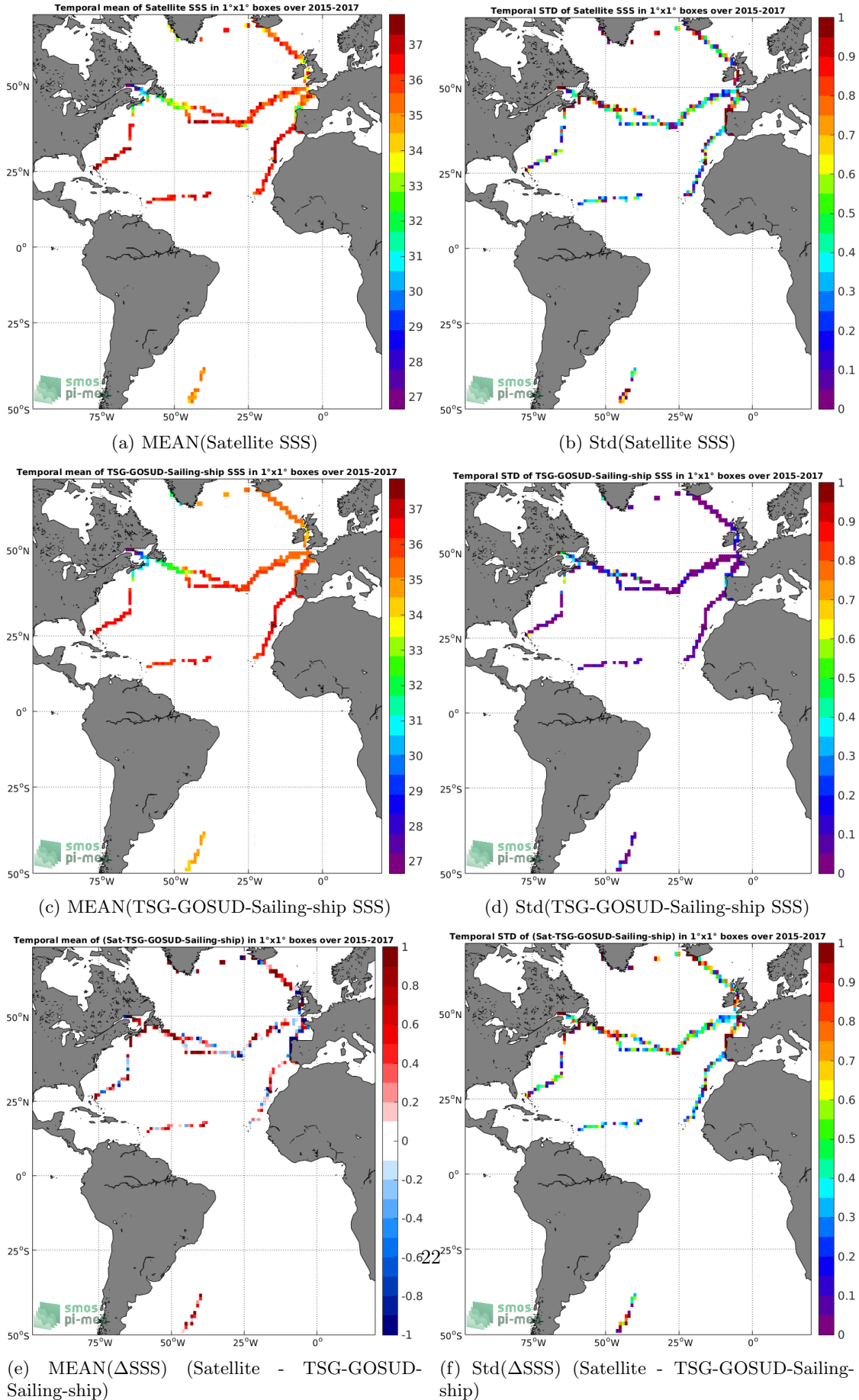
Figure 6: Temporal mean (left) and Std (right) of SSS from SMAP-L2-JPL-V4.2 (top), TSG-GOSUD-Sailing-ship (middle), and of \Delta SSS (Satellite - TSG-GOSUD-Sailing-ship). Only match-up pairs are used to generate these maps.
