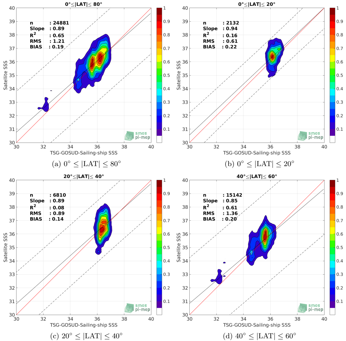
Figure 9: Contour maps of the concentration of SMAP-L2-JPL-V4.2 SSS (y-axis) versus TSG-GOSUD-Sailing-ship SSS (x-axis) at match-up pairs for different latitude bands. For each plot, the red line shows x=y . The black thin and dashed lines indicate a linear fit through the data cloud and the \pm 95\% confidence levels, respectively. The number match-up pairs n , the slope and R^2 coefficient of the linear fit, the root mean square (RMS) and the mean bias between satellite and in situ data are indicated for each latitude band in each plots.
