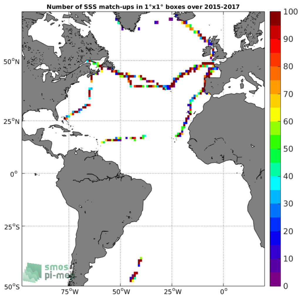
Figure 4: Number of SSS match-ups between TSG-GOSUD-Sailing-ship SSS and the SMAP-L2-JPL-V4.2 SSS product for the Atlantic Ocean Pi-MEP region over 1°x1° boxes and for the full satellite product period.
