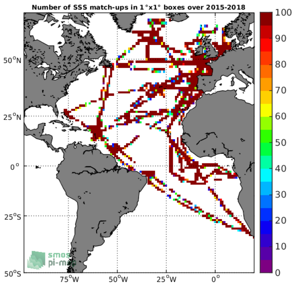
Figure 4: Number of SSS match-ups between TSG-GOSUD-Research-vessel SSS and the SMAP-L2-JPL-V4.2 SSS product for the Atlantic Ocean Pi-MEP region over 1°x1° boxes and for the full satellite product period.
