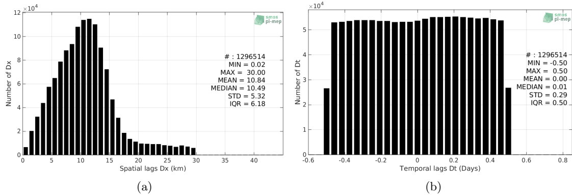
Figure 5: Histograms of the spatial (a) and temporal (b) lags between the time of the TSG-GOSUD-Research-vessel measurements and the date of the corresponding SMAP-L2-JPL-V4.2 SSS product.
