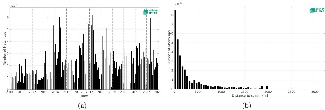
Figure 2: Number of match-ups between TSG (GOSUD-Research-vessel) and ISAS v7 - Monthly (Ifremer-LOPS-CMEMS) SSS as a function of time (a) and as function of the distance to coast (b) over the Atlantic Ocean Pi-MEP region and for the full satellite product period.
