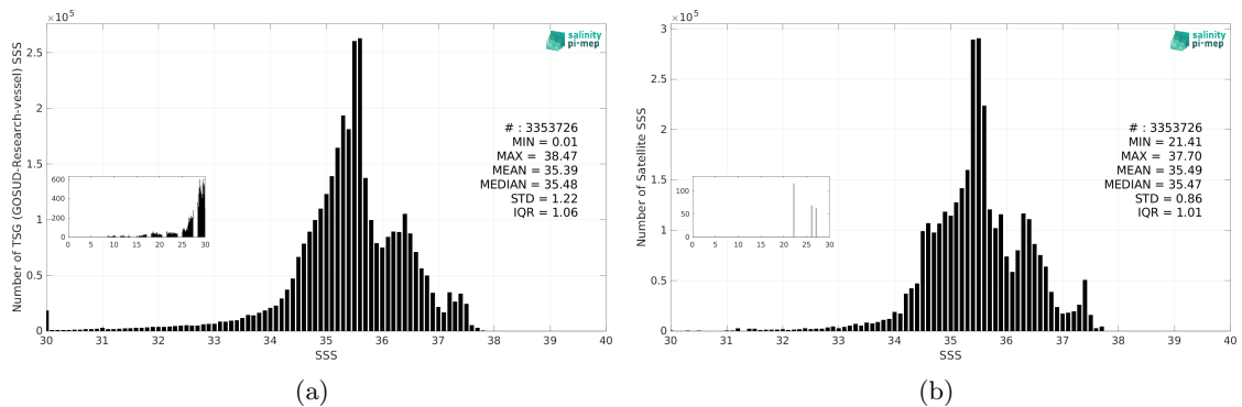
Figure 3: Histograms of SSS from TSG (GOSUD-Research-vessel) (a) and ISAS v7 - Monthly (Ifremer-LOPS-CMEMS) (b) considering all match-up pairs per bins of 0.1 over the Atlantic Ocean Pi-MEP region and for the full satellite product period.
