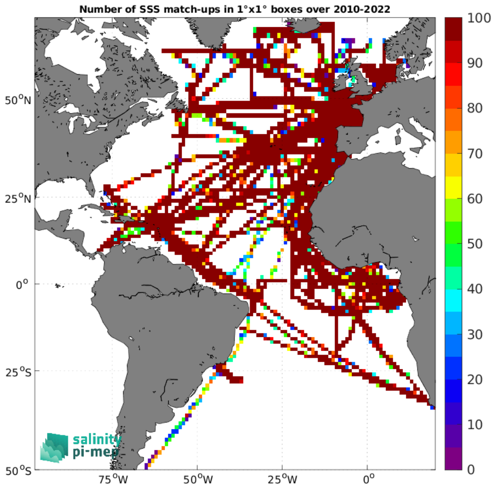
Figure 5: Number of SSS match-ups between TSG (GOSUD-Research-vessel) SSS and the ISAS v7 - Monthly (Ifremer-LOPS-CMEMS) SSS product for the Atlantic Ocean Pi-MEP region over 1° × 1° boxes and for the full satellite product period.
