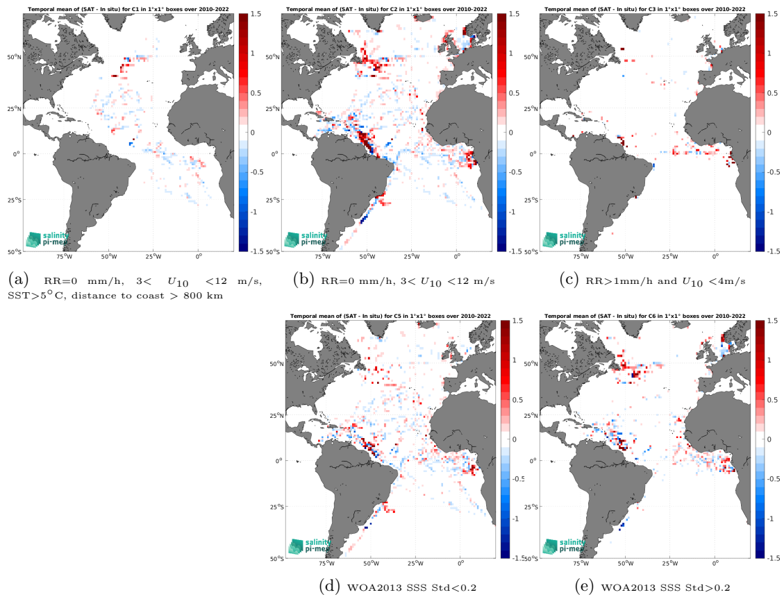
Figure 14: Temporal mean gridded over spatial boxes of size 1^\circ \times 1^\circ of \Delta SSS (ISAS v7 - Monthly (Ifremer-LOPS-CMEMS) - TSG (GOSUD-Research-vessel)) for 5 different subdatasets corresponding to:RR=0 mm/h, 3 < U_{10} < 12 m/s, SST >5^\circ\text{C} , distance to coast > 800 km (a), RR=0 mm/h, 3 < U_{10} < 12 m/s (b), RR >1 mm/h and U_{10} < 4 m/s (c), WOA2013 SSS Std <0.2 (d), WOA2013 SSS Std >0.2 (e).
