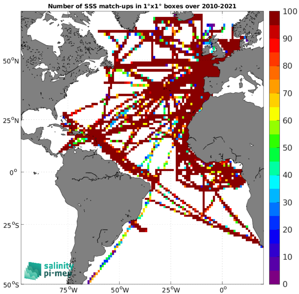
Figure 5: Number of SSS match-ups between TSG (GOSUD-Research-vessel) SSS and the ISAS SSS product for the Atlantic Ocean Pi-MEP region over 1^\circ \times 1^\circ boxes and for the full satellite product period.
