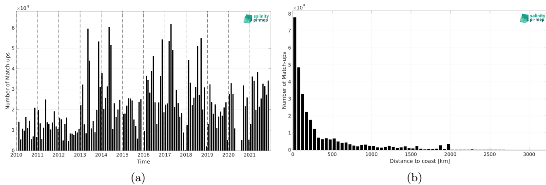
Figure 2: Number of match-ups between TSG (GOSUD-Research-vessel) and ISAS SSS as a function of time (a) and as function of the distance to coast (b) over the Atlantic Ocean Pi-MEP region and for the full satellite product period.
