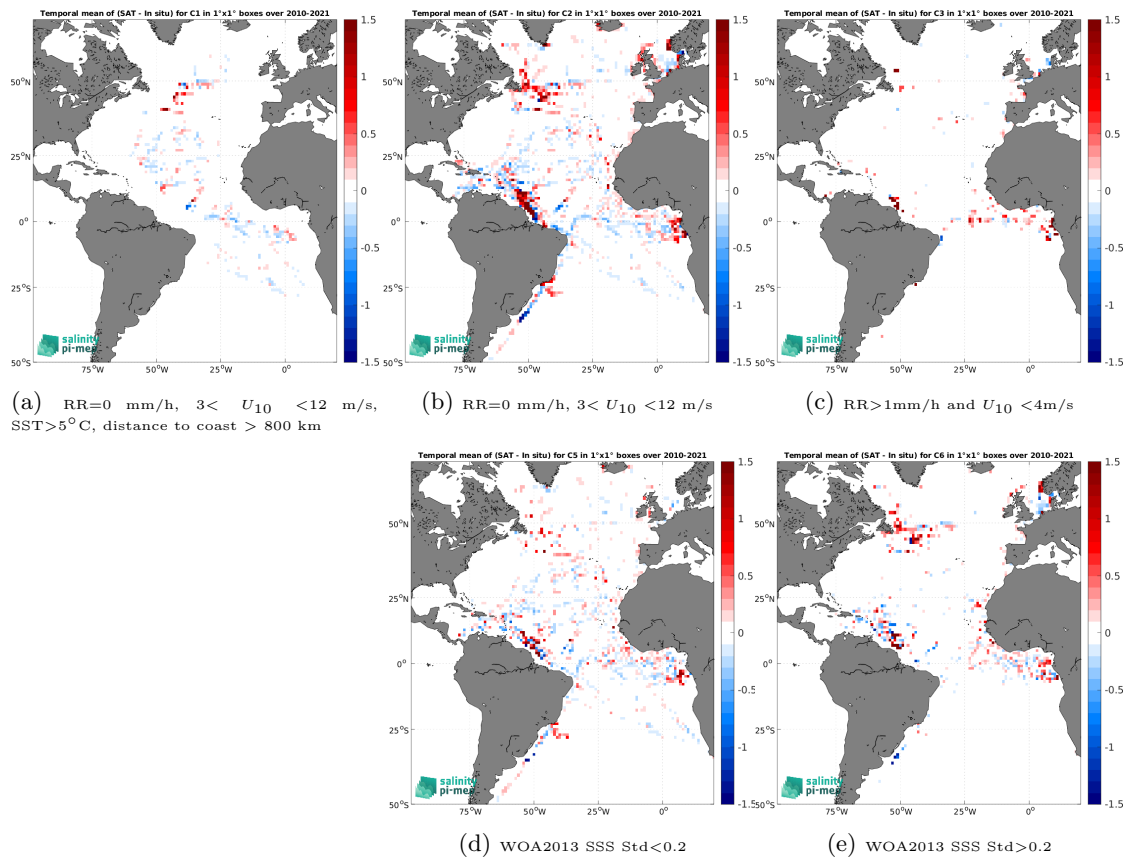
Figure 14: Temporal mean gridded over spatial boxes of size 1^\circ \times 1^\circ of \Delta SSS (ISAS - TSG (GOSUD-Research-vessel)) for 5 different subdatasets corresponding to:RR=0 mm/h, 3 < U_{10} < 12 m/s, SST>5°C, distance to coast > 800 km (a), RR=0 mm/h, 3 < U_{10} < 12 m/s (b), RR>1mm/h and U_{10} < 4 m/s (c), WOA2013 SSS Std<0.2 (d), WOA2013 SSS Std>0.2 (e).
