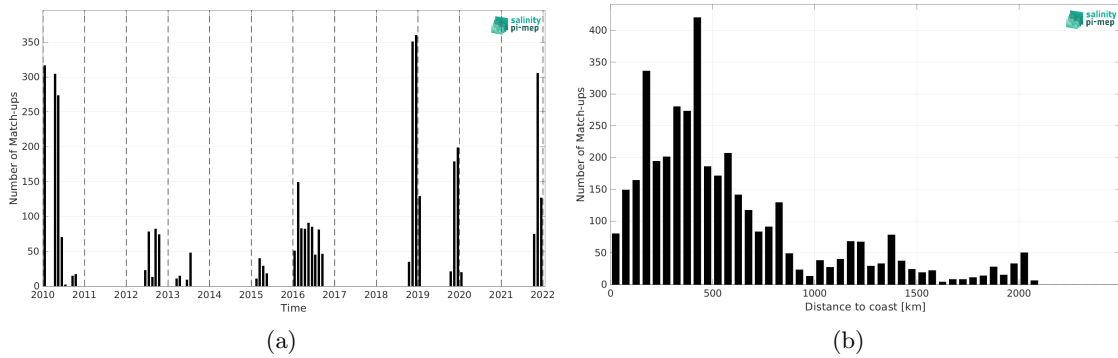
Figure 2: Number of match-ups between Marine mammals and ISAS v7 - Monthly (Ifremer-LOPS-CMEMS) SSS as a function of time (a) and as function of the distance to coast (b) over the Atlantic Ocean Pi-MEP region and for the full satellite product period.
