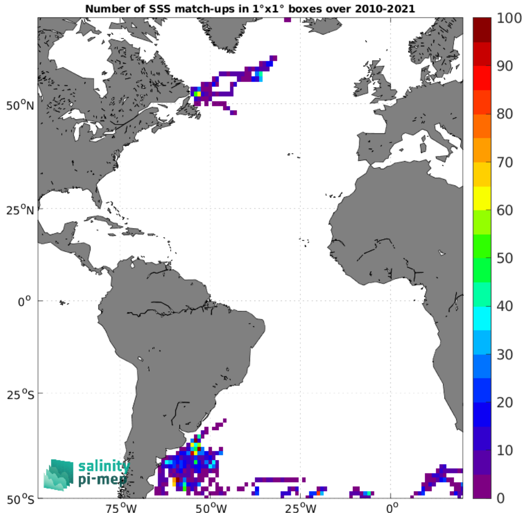
Figure 5: Number of SSS match-ups between Marine mammals SSS and the ISAS v7 - Monthly (Ifremer-LOPS-CMEMS) SSS product for the Atlantic Ocean Pi-MEP region over 1^\circ \times 1^\circ boxes and for the full satellite product period.
