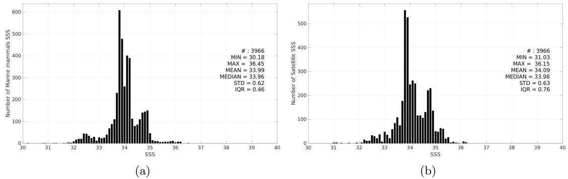
Figure 3: Histograms of SSS from Marine mammals (a) and ISAS v7 - Monthly (Ifremer-LOPS-CMEMS) (b) considering all match-up pairs per bins of 0.1 over the Atlantic Ocean Pi-MEP region and for the full satellite product period.
