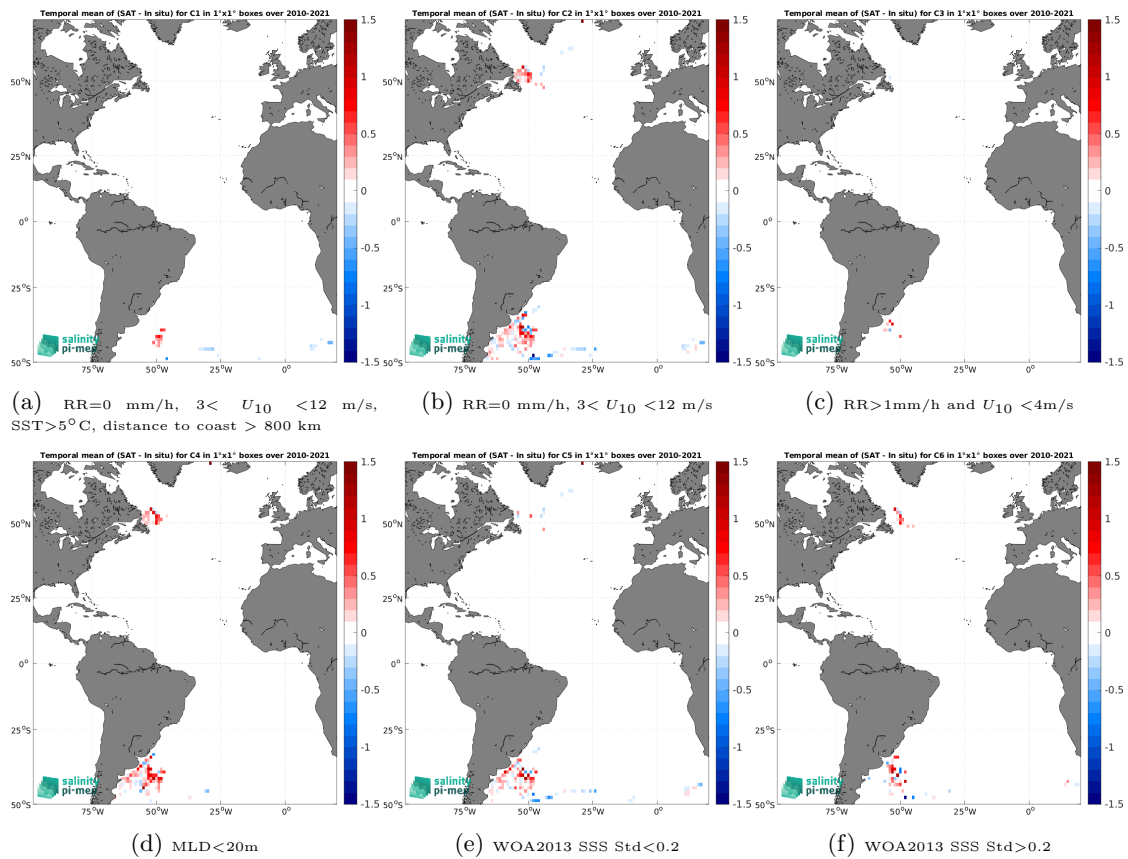
Figure 14: Temporal mean gridded over spatial boxes of size 1^\circ \times 1^\circ of \Delta SSS (ISAS v7 - Monthly (Ifremer-LOPS-CMEMS) - Marine mammals) for 6 different subdatasets corresponding to:RR=0 mm/h, 3 < U_{10} < 12 m/s, SST >5^\circ C, distance to coast > 800 km (a), RR=0 mm/h, 3 < U_{10} < 12 m/s (b), RR >1 mm/h and U_{10} < 4 m/s (c),MLD <20 m (d),WOA2013 SSS Std <0.2 (e),WOA2013 SSS Std >0.2 (f).
