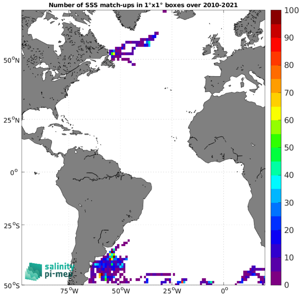
Figure 5: Number of SSS match-ups between Marine mammals SSS and the ISAS SSS product for the Atlantic Ocean Pi-MEP region over 1^\circ \times 1^\circ boxes and for the full satellite product period.
