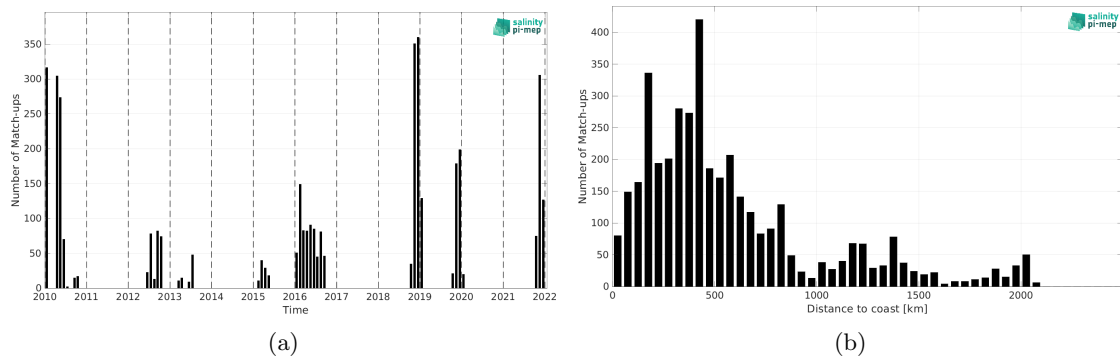
Figure 2: Number of match-ups between Marine mammals and ISAS SSS as a function of time (a) and as function of the distance to coast (b) over the Atlantic Ocean Pi-MEP region and for the full satellite product period.
