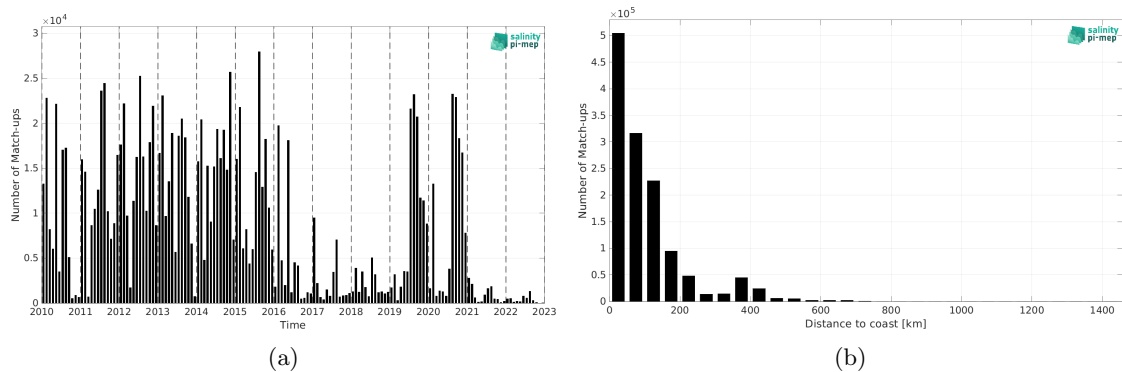
Figure 2: Number of match-ups between ICES and ISAS v7 - Monthly (Ifremer-LOPS-CMEMS) SSS as a function of time (a) and as function of the distance to coast (b) over the Atlantic Ocean Pi-MEP region and for the full satellite product period.
