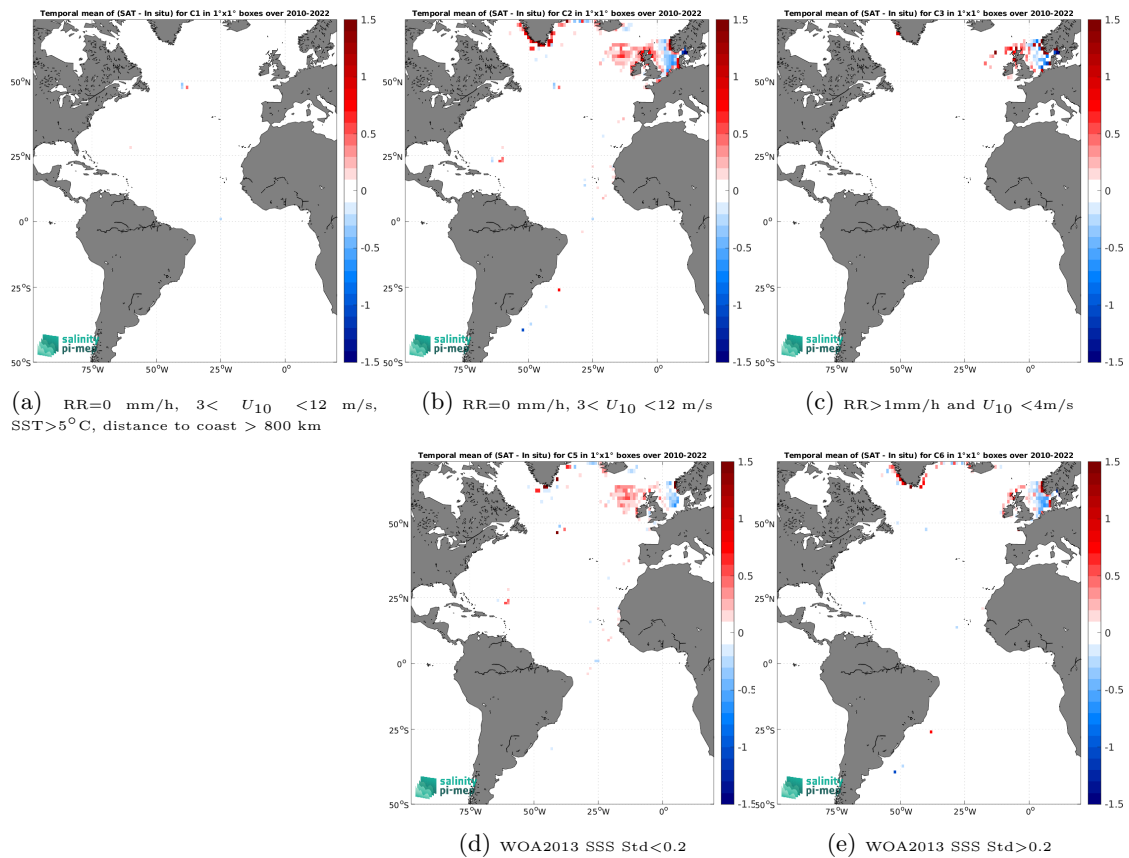
Figure 14: Temporal mean gridded over spatial boxes of size 1^\circ \times 1^\circ of \Delta\text{SSS} (ISAS v7 - Monthly (Ifremer-LOPS-CMEMS) - ICES) for 5 different subdatasets corresponding to:RR=0 mm/h, 3 < U_{10} < 12 m/s, SST >5^\circ\text{C} , distance to coast > 800 km (a), RR=0 mm/h, 3 < U_{10} < 12 m/s (b), RR >1 mm/h and U_{10} < 4 m/s (c), WOA2013 SSS Std <0.2 (d), WOA2013 SSS Std >0.2 (e).
