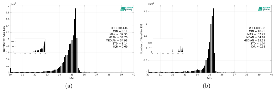
Figure 3: Histograms of SSS from ICES (a) and ISAS v7 - Monthly (Ifremer-LOPS-CMEMS) (b) considering all match-up pairs per bins of 0.1 over the Atlantic Ocean Pi-MEP region and for the full satellite product period.
