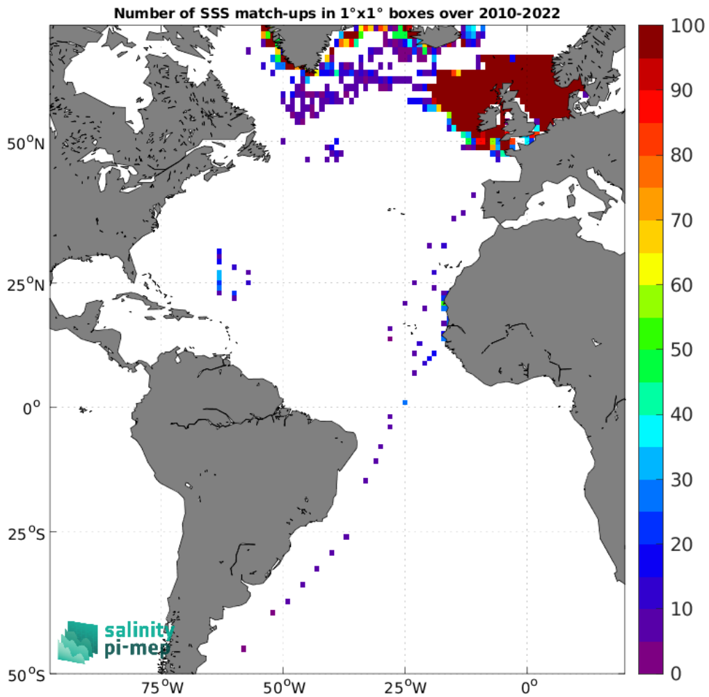
Figure 5: Number of SSS match-ups between ICES SSS and the ISAS v7 - Monthly (Ifremer-LOPS-CMEMS) SSS product for the Atlantic Ocean Pi-MEP region over 1^\circ \times 1^\circ boxes and for the full satellite product period.
