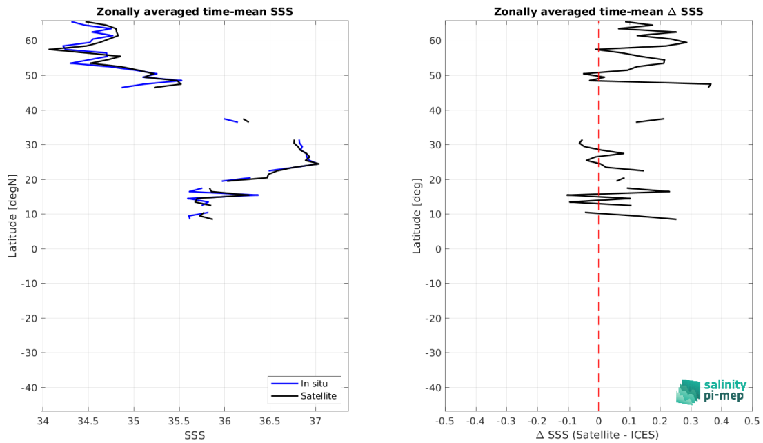
Figure 9: Left panel: Zonal mean SSS from ISAS satellite product (black) and from ICES (blue). Right panel: Zonal mean of \Delta SSS (Satellite - ICES) for all the collected Pi-MEP match-up pairs estimated over the full satellite product period.
