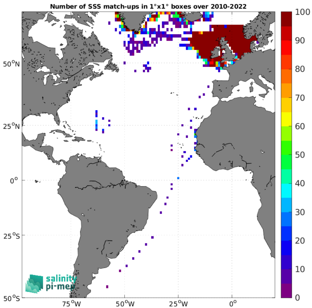
Figure 5: Number of SSS match-ups between ICES SSS and the ISAS SSS product for the Atlantic Ocean Pi-MEP region over 1^{\circ} \times 1^{\circ} boxes and for the full satellite product period.
