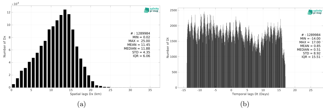
Figure 6: Histograms of the spatial (a) and temporal (b) lags between the location/time of the ICES measurement and the date of the corresponding ISAS SSS pixel.
