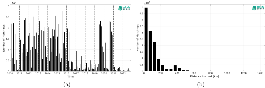
Figure 2: Number of match-ups between ICES and ISAS SSS as a function of time (a) and as function of the distance to coast (b) over the Atlantic Ocean Pi-MEP region and for the full satellite product period.
