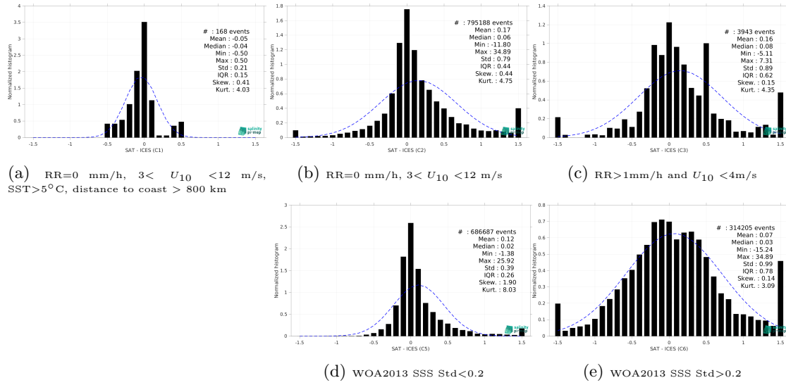
Figure 15: Normalized histogram of \Delta SSS (ISAS - ICES) for 5 different subdatasets corresponding to: RR=0 mm/h, 3 < U_{10} < 12 m/s, SST > 5°C, distance to coast > 800 km (a), RR=0 mm/h, 3 < U_{10} < 12 m/s (b), RR > 1mm/h and U_{10} < 4 m/s (c), WOA2013 SSS Std < 0.2 (d), WOA2013 SSS Std > 0.2 (e).
