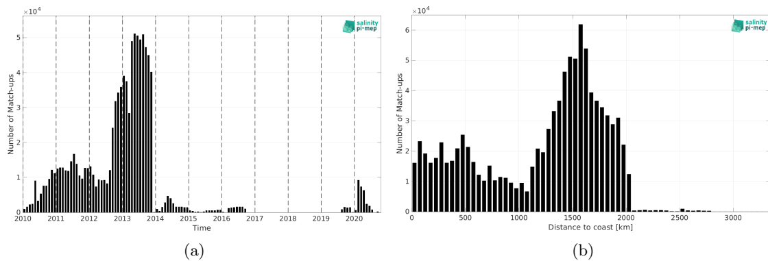
Figure 2: Number of match-ups between Surface drifters and ISAS v7 - Monthly (Ifremer-LOPS-CMEMS) SSS as a function of time (a) and as function of the distance to coast (b) over the Atlantic Ocean Pi-MEP region and for the full satellite product period.
