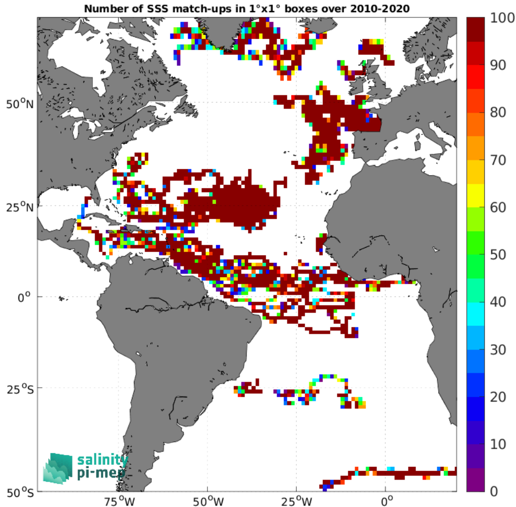
Figure 4: Number of SSS match-ups between Surface drifters SSS and the ISAS v7 - Monthly (Ifremer-LOPS-CMEMS) SSS product for the Atlantic Ocean Pi-MEP region over 1^\circ \times 1^\circ boxes and for the full satellite product period.
