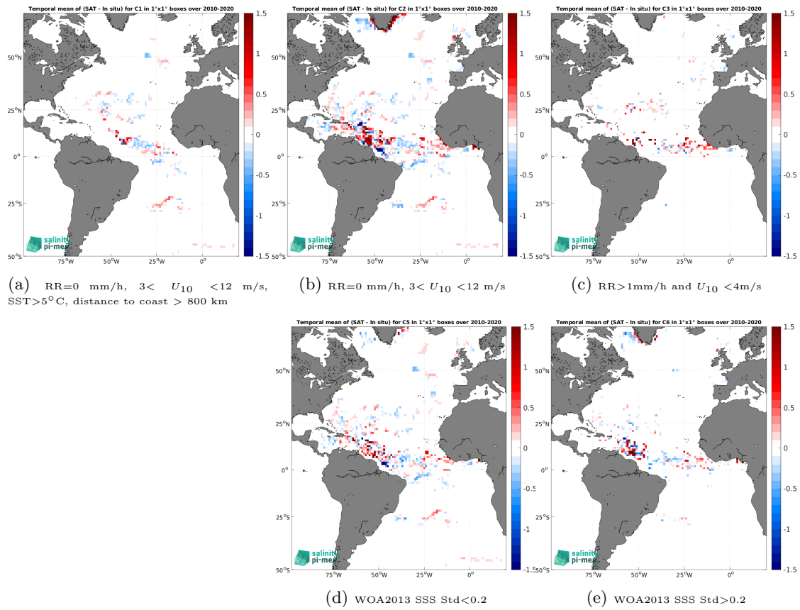
Figure 13: Temporal mean gridded over spatial boxes of size 1^\circ \times 1^\circ of \Delta SSS (ISAS v7 - Monthly (Ifremer-LOPS-CMEMS) - Surface drifters) for 5 different subdatasets corresponding to:RR=0 mm/h, 3 < U_{10} < 12 m/s, SST >5^\circ\text{C} , distance to coast > 800 km (a), RR=0 mm/h, 3 < U_{10} < 12 m/s (b), RR >1 mm/h and U_{10} < 4 m/s (c), WOA2013 SSS Std <0.2 (d), WOA2013 SSS Std >0.2 (e).
