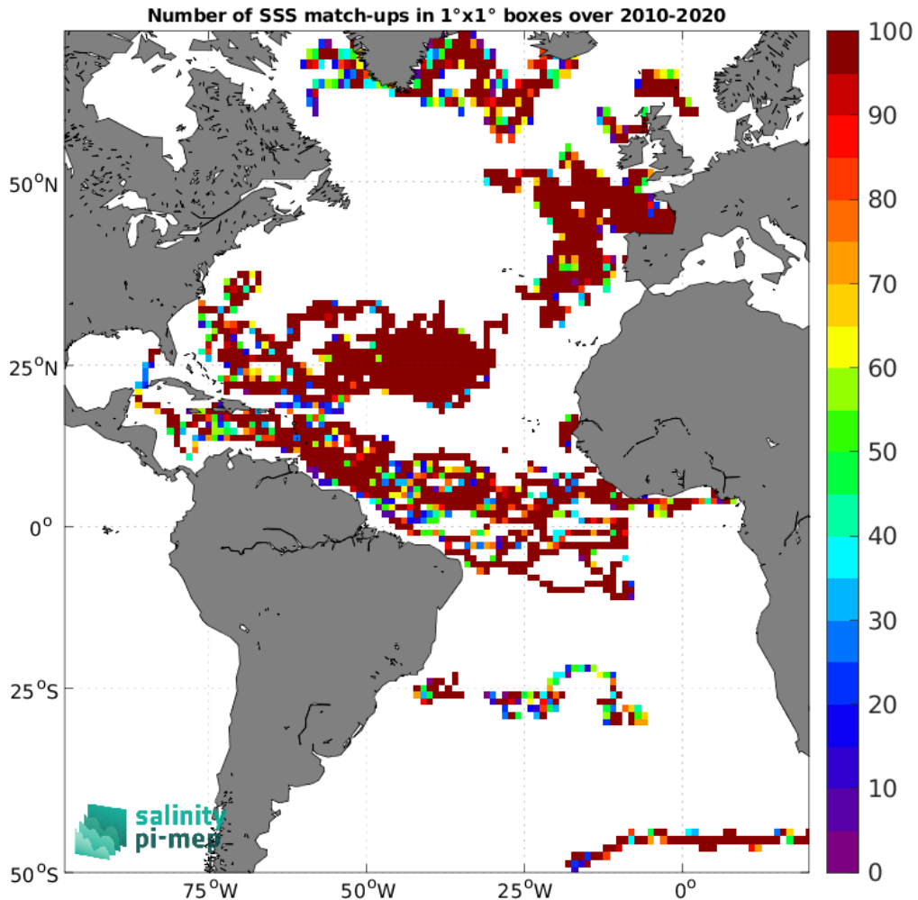
Figure 4: Number of SSS match-ups between Surface drifters SSS and the ISAS SSS product for the Atlantic Ocean Pi-MEP region over 1^\circ \times 1^\circ boxes and for the full satellite product period.
