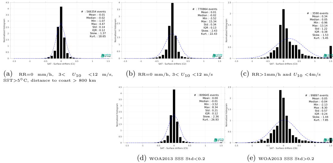
Figure 14: Normalized histogram of \Delta SSS (ISAS - Surface drifters) for 5 different subdatasets corresponding to: RR=0 mm/h, 3 < U_{10} < 12 m/s, SST>5°C, distance to coast > 800 km (a), RR=0 mm/h, 3 < U_{10} < 12 m/s (b), RR>1mm/h and U_{10} < 4 m/s (c), WOA2013 SSS Std<0.2 (d), WOA2013 SSS Std>0.2 (e).
