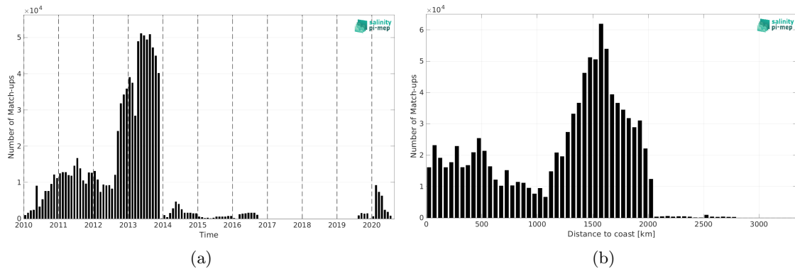
Figure 2: Number of match-ups between Surface drifters and ISAS SSS as a function of time (a) and as function of the distance to coast (b) over the Atlantic Ocean Pi-MEP region and for the full satellite product period.
