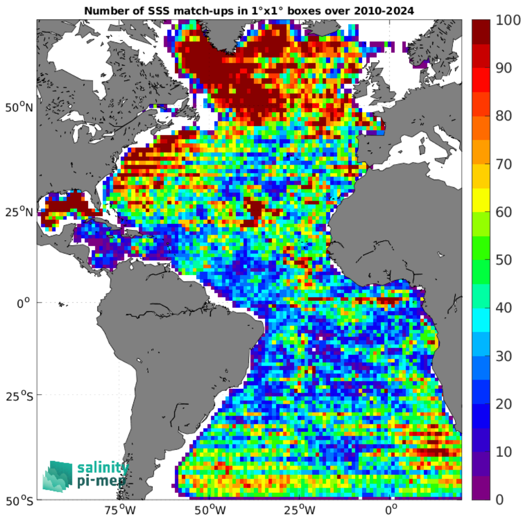
Figure 5: Number of SSS match-ups between Argo SSS and the ISAS SSS product for the Atlantic Ocean Pi-MEP region over 1^\circ \times 1^\circ boxes and for the full satellite product period.
