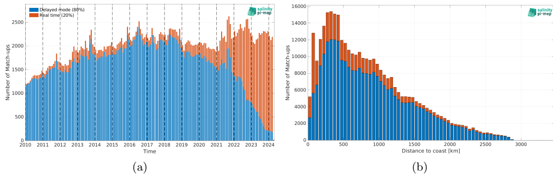
Figure 2: Number of match-ups between Argo and ISAS SSS as a function of time (a) and as function of the distance to coast (b) over the Atlantic Ocean Pi-MEP region and for the full satellite product period.
