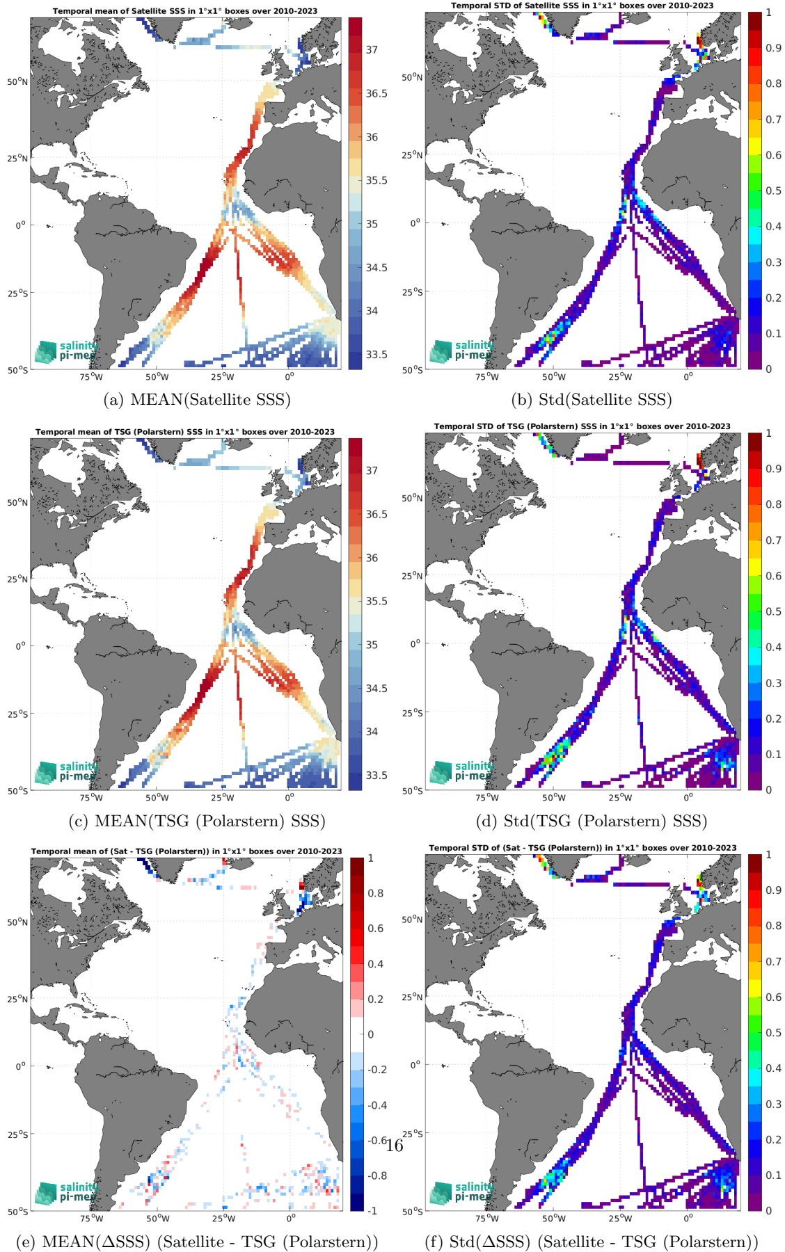
Figure 7: Temporal mean (left) and Std (right) of SSS from CCI SSS L4 Merged-OI v5.5 - 7-day running (ESA) (top), TSG (Polarstern) (middle), and of \Delta SSS (Satellite - TSG (Polarstern)). Only match-up pairs are used to generate these maps.
