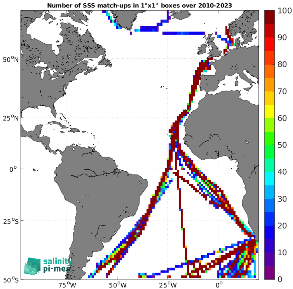
Figure 5: Number of SSS match-ups between TSG (Polarstern) SSS and the CCI SSS L4 Merged-OI v5.5 - 7-day running (ESA) SSS product for the Atlantic Ocean Pi-MEP region over 1°x1° boxes and for the full satellite product period.
