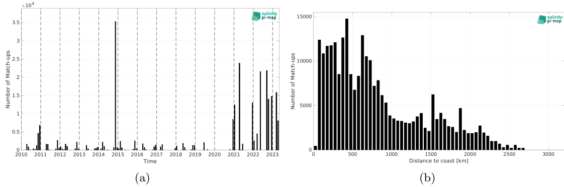
Figure 2: Number of match-ups between TSG (Polarstern) and CCI SSS L4 Merged-OI v5.5 - 7-day running (ESA) SSS as a function of time (a) and as function of the distance to coast (b) over the Atlantic Ocean Pi-MEP region and for the full satellite product period.
