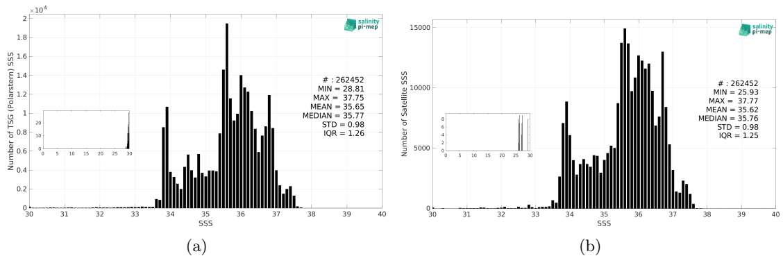
Figure 3: Histograms of SSS from TSG (Polarstern) (a) and CCI SSS L4 Merged-OI v5.5 - 7-day running (ESA) (b) considering all match-up pairs per bins of 0.1 over the Atlantic Ocean Pi-MEP region and for the full satellite product period.
