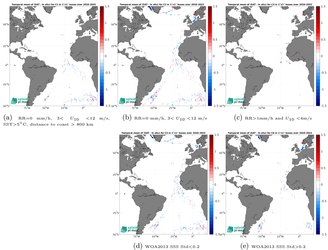
Figure 14: Temporal mean gridded over spatial boxes of size 1^\circ \times 1^\circ of \Delta\text{SSS} (CCI SSS L4 Merged-OI v5.5 - 7-day running (ESA) - TSG (Polarstern)) for 5 different subdatasets corresponding to:RR=0 mm/h, 3 < U_{10} < 12 m/s, SST >5^\circ\text{C} , distance to coast > 800 km (a), RR=0 mm/h, 3 < U_{10} < 12 m/s (b), RR >1 mm/h and U_{10} < 4 m/s (c), WOA2013 SSS Std <0.2 (d), WOA2013 SSS Std >0.2 (e).
