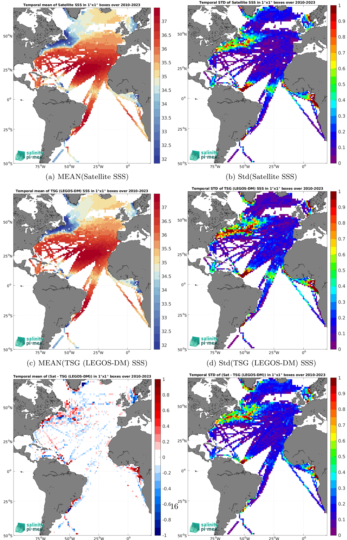
(e) MEAN( \Delta SSS) (Satellite - TSG (LEGOS-DM)) (f) Std( \Delta SSS) (Satellite - TSG (LEGOS-DM)) Figure 7: Temporal mean (left) and Std (right) of SSS from CCI SSS L4 Merged-OI v5.5 - 7-day running (ESA) (top), TSG (LEGOS-DM) (middle), and of \Delta SSS (Satellite - TSG (LEGOS-DM)). Only match-up pairs are used to generate these maps.
