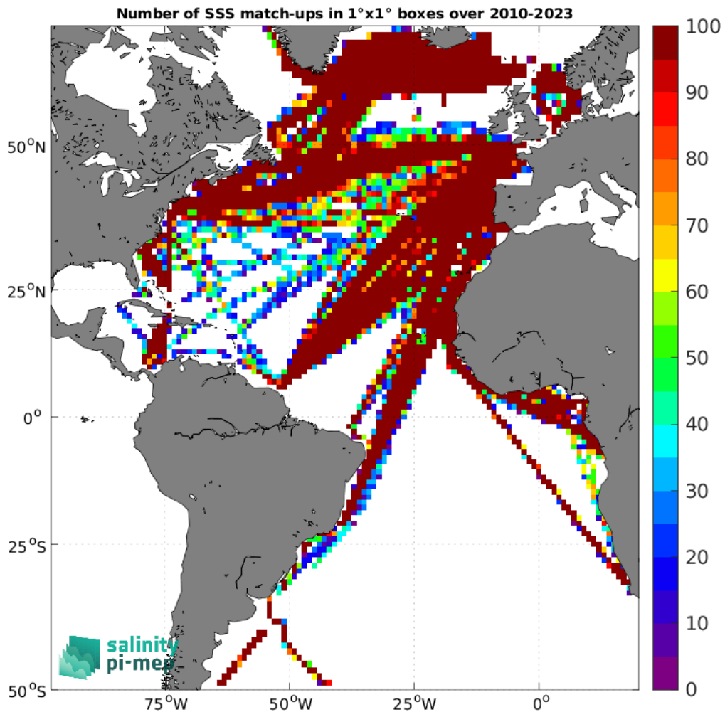
Figure 5: Number of SSS match-ups between TSG (LEGOS-DM) SSS and the CCI SSS L4 Merged-OI v5.5 - 7-day running (ESA) SSS product for the Atlantic Ocean Pi-MEP region over 1^\circ \times 1^\circ boxes and for the full satellite product period.
