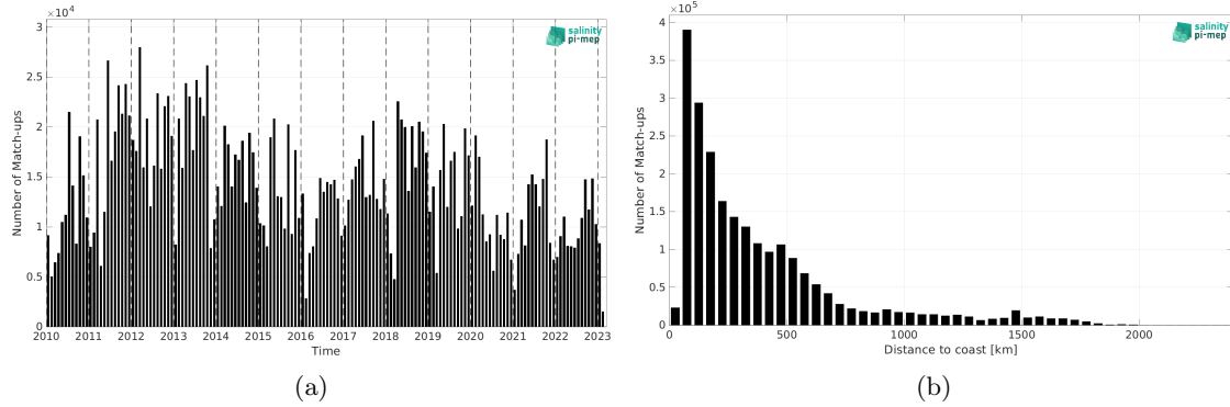
Figure 2: Number of match-ups between TSG (LEGOS-DM) and CCI SSS L4 Merged-OI v5.5 - 7-day running (ESA) SSS as a function of time (a) and as function of the distance to coast (b) over the Atlantic Ocean Pi-MEP region and for the full satellite product period.
