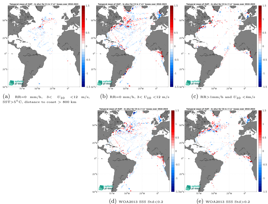
Figure 14: Temporal mean gridded over spatial boxes of size 1^\circ \times 1^\circ of \Delta\text{SSS} (CCI SSS L4 Merged-OI v5.5 - 7-day running (ESA) - TSG (LEGOS-DM)) for 5 different subdatasets corresponding to:RR=0 mm/h, 3 < U_{10} < 12 m/s, SST>5°C, distance to coast > 800 km (a), RR=0 mm/h, 3 < U_{10} < 12 m/s (b), RR>1mm/h and U_{10} < 4 m/s (c), WOA2013 SSS Std<0.2 (d), WOA2013 SSS Std>0.2 (e).
