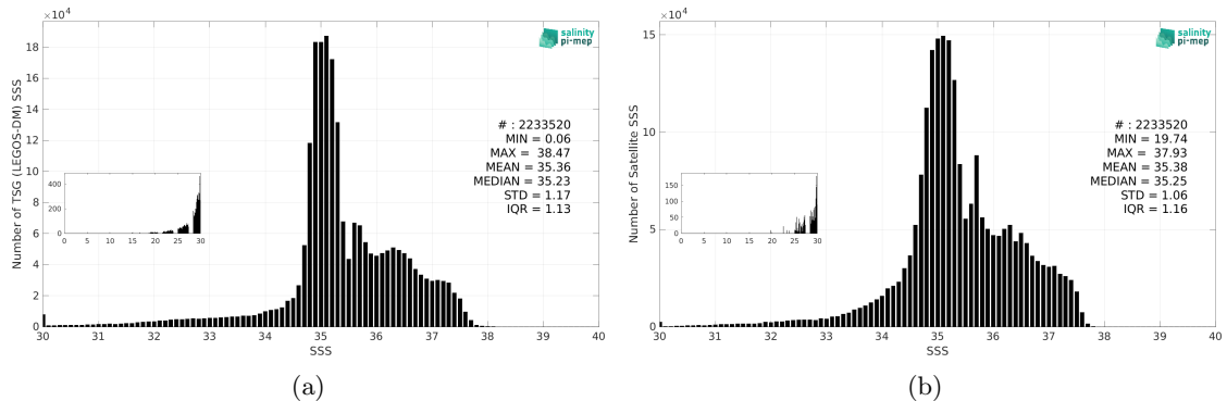
Figure 3: Histograms of SSS from TSG (LEGOS-DM) (a) and CCI SSS L4 Merged-OI v5.5 - 7-day running (ESA) (b) considering all match-up pairs per bins of 0.1 over the Atlantic Ocean Pi-MEP region and for the full satellite product period.
