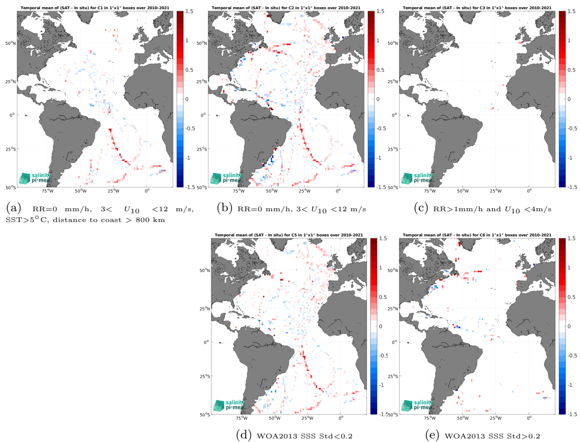
Figure 14: Temporal mean gridded over spatial boxes of size 1^\circ \times 1^\circ of \Delta\text{SSS} (CCI SSS L4 Merged-OI v5.5 - 7-day running (ESA) - TSG (GOSUD-Sailing-ship)) for 5 different subdatasets corresponding to:RR=0 mm/h, 3 < U_{10} < 12 m/s, SST>5°C, distance to coast > 800 km (a), RR=0 mm/h, 3 < U_{10} < 12 m/s (b), RR>1mm/h and U_{10} < 4 m/s (c), WOA2013 SSS Std<0.2 (d), WOA2013 SSS Std>0.2 (e).
