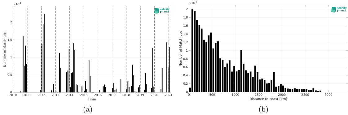
Figure 2: Number of match-ups between TSG (GOSUD-Sailing-ship) and CCI SSS L4 Merged-OI v5.5 - 7-day running (ESA) SSS as a function of time (a) and as function of the distance to coast (b) over the Atlantic Ocean Pi-MEP region and for the full satellite product period.
