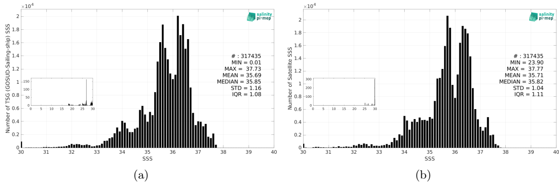
Figure 3: Histograms of SSS from TSG (GOSUD-Sailing-ship) (a) and CCI SSS L4 Merged-OI v5.5 - 7-day running (ESA) (b) considering all match-up pairs per bins of 0.1 over the Atlantic Ocean Pi-MEP region and for the full satellite product period.
