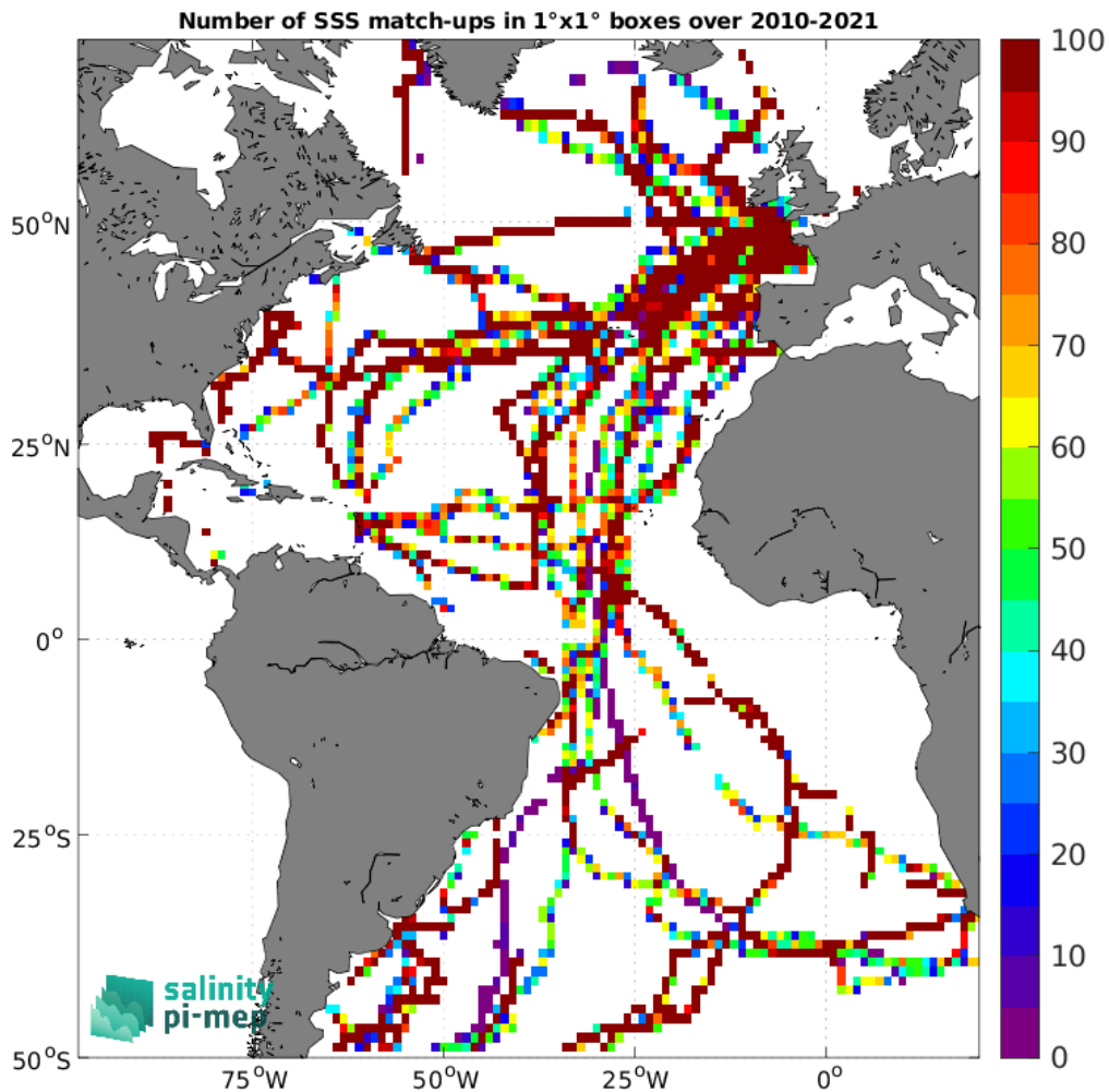
Figure 5: Number of SSS match-ups between TSG (GOSUD-Sailing-ship) SSS and the CCI SSS L4 Merged-OI v5.5 - 7-day running (ESA) SSS product for the Atlantic Ocean Pi-MEP region over 1°x1° boxes and for the full satellite product period.
