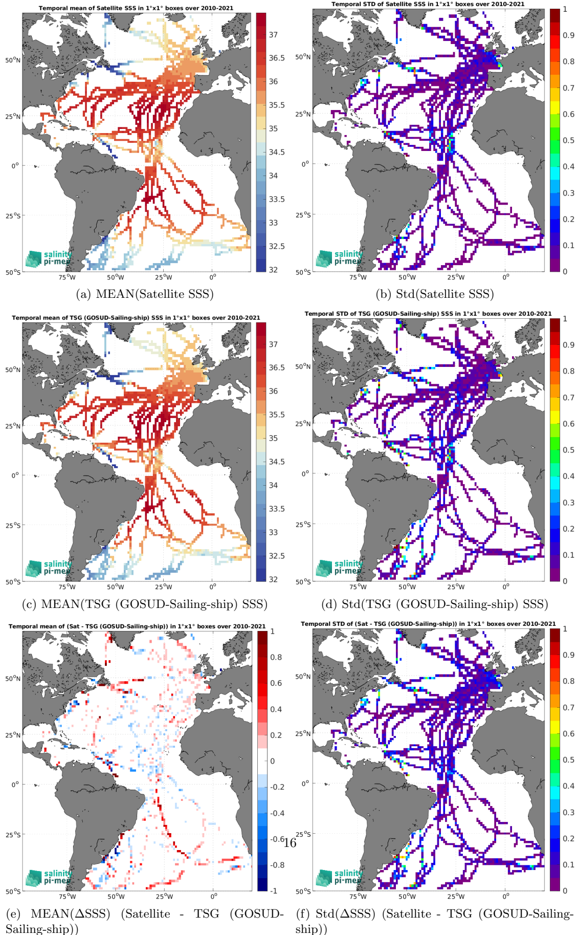
Figure 7: Temporal mean (left) and Std (right) of SSS from CCI SSS L4 Merged-OI v5.5 - 7-day running (ESA) (top), TSG (GOSUD-Sailing-ship) (middle), and of \Delta SSS (Satellite - TSG (GOSUD-Sailing-ship)). Only match-up pairs are used to generate these maps.
