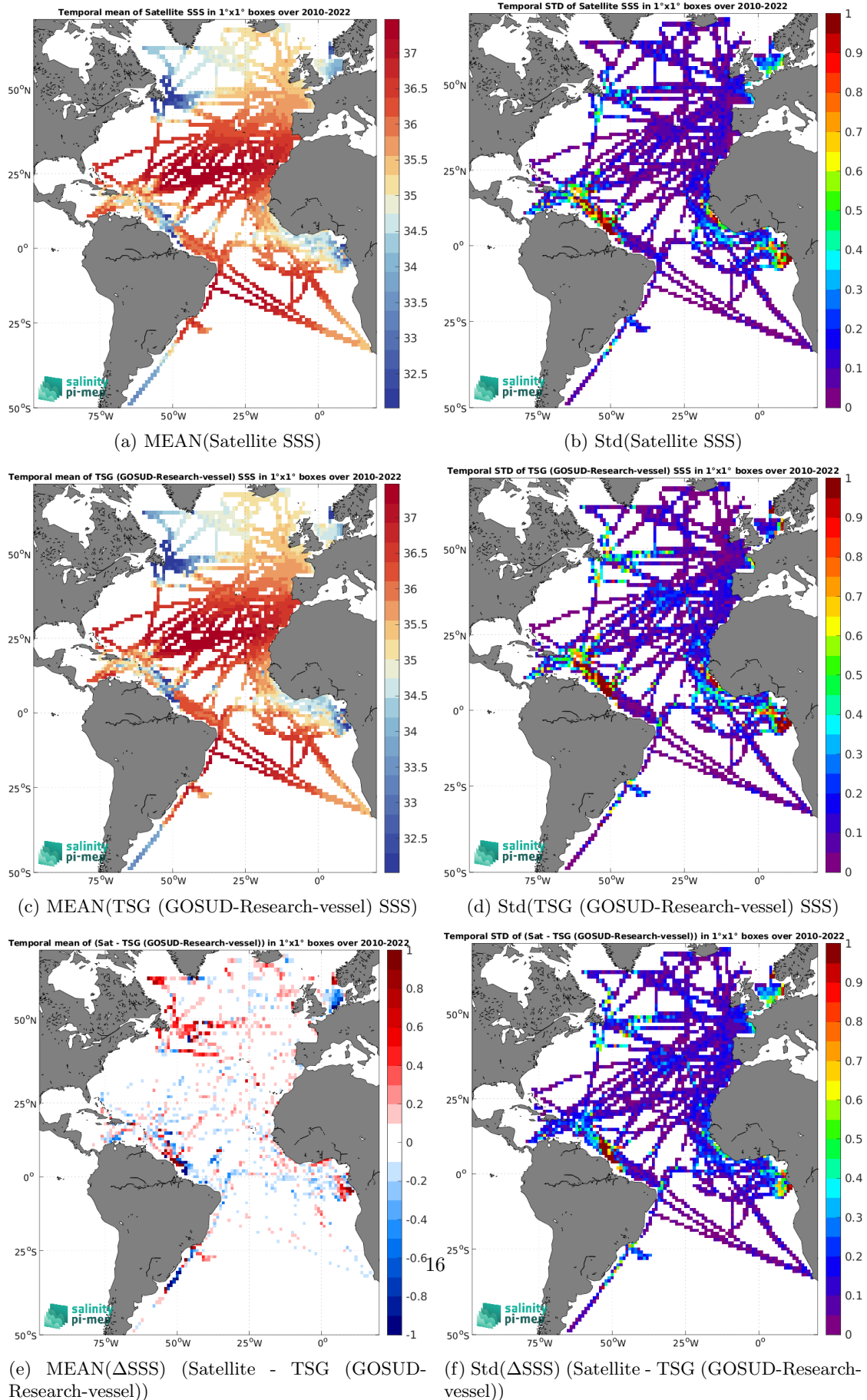
Figure 7: Temporal mean (left) and Std (right) of SSS from CCI SSS L4 Merged-OI v5.5 - 7-day running (ESA) (top), TSG (GOSUD-Research-vessel) (middle), and of \Delta\text{SSS} (Satellite - TSG (GOSUD-Research-vessel)). Only match-up pairs are used to generate these maps.
