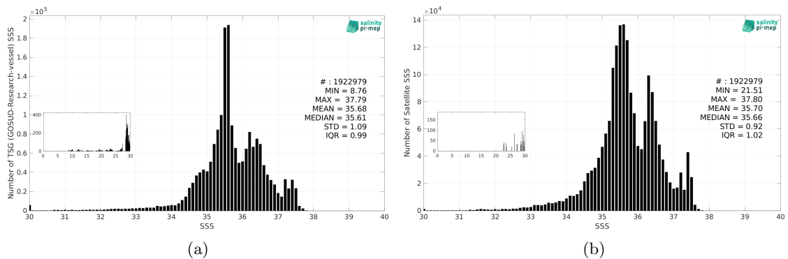
Figure 3: Histograms of SSS from TSG (GOSUD-Research-vessel) (a) and CCI SSS L4 Merged-OI v5.5 - 7-day running (ESA) (b) considering all match-up pairs per bins of 0.1 over the Atlantic Ocean Pi-MEP region and for the full satellite product period.
