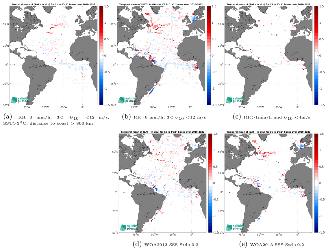
Figure 14: Temporal mean gridded over spatial boxes of size 1^\circ \times 1^\circ of \Delta\text{SSS} (CCI SSS L4 Merged-OI v5.5 - 7-day running (ESA) - TSG (GOSUD-Research-vessel)) for 5 different subdatasets corresponding to:RR=0 mm/h, 3 < U_{10} < 12 m/s, SST>5°C, distance to coast > 800 km (a), RR=0 mm/h, 3 < U_{10} < 12 m/s (b), RR>1mm/h and U_{10} < 4 m/s (c), WOA2013 SSS Std<0.2 (d), WOA2013 SSS Std>0.2 (e).
