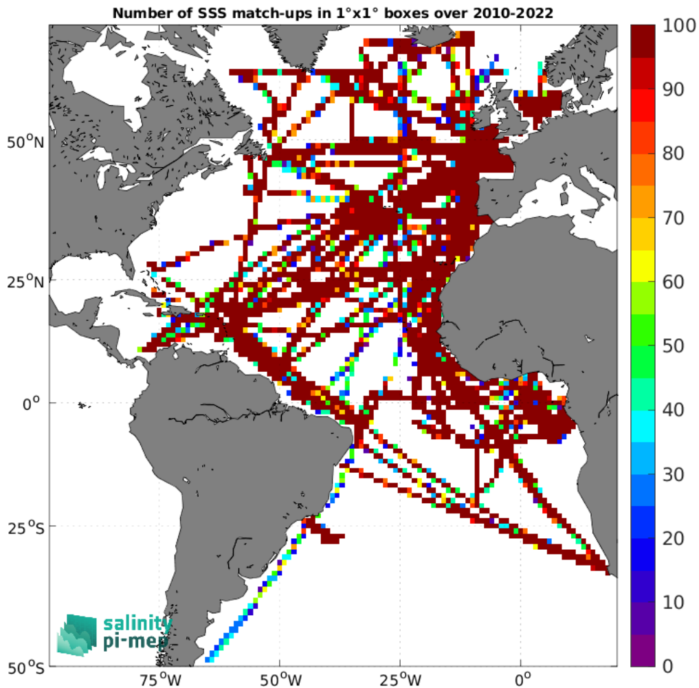
Figure 5: Number of SSS match-ups between TSG (GOSUD-Research-vessel) SSS and the CCI SSS L4 Merged-OI v5.5 - 7-day running (ESA) SSS product for the Atlantic Ocean Pi-MEP region over 1^\circ \times 1^\circ boxes and for the full satellite product period.
