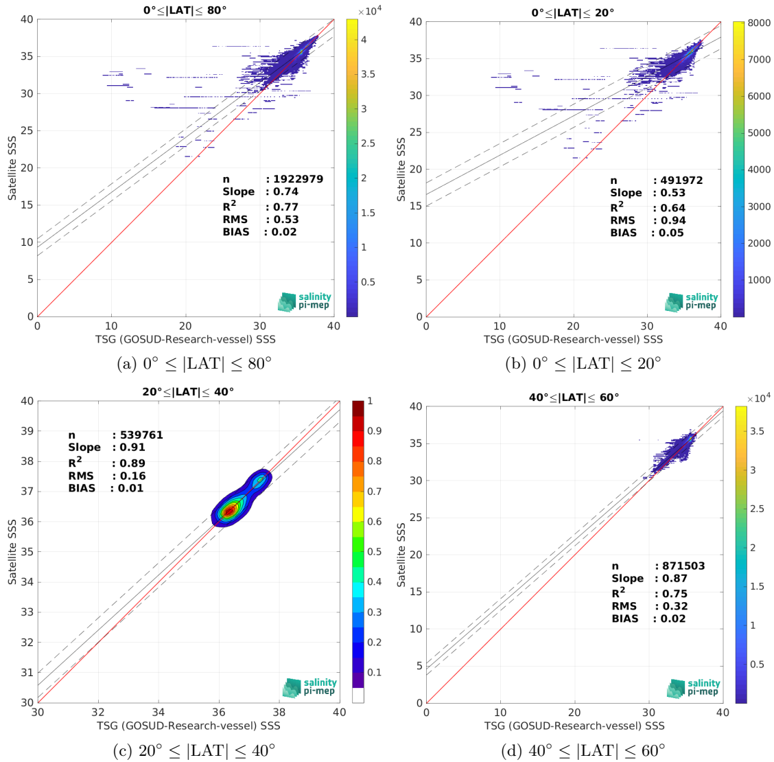
Figure 10: Contour maps of the concentration of CCI SSS L4 Merged-OI v5.5 - 7-day running (ESA) SSS (y-axis) versus TSG (GOSUD-Research-vessel) SSS (x-axis) at match-up pairs for different latitude bands. For each plot, the red line shows x=y . The black thin and dashed lines indicate a linear fit through the data cloud and the \pm 95\% confidence levels, respectively. The number match-up pairs n , the slope and R^2 coefficient of the linear fit, the root mean square (RMS) and the mean bias between satellite and in situ data are indicated for each latitude band in each plots.
