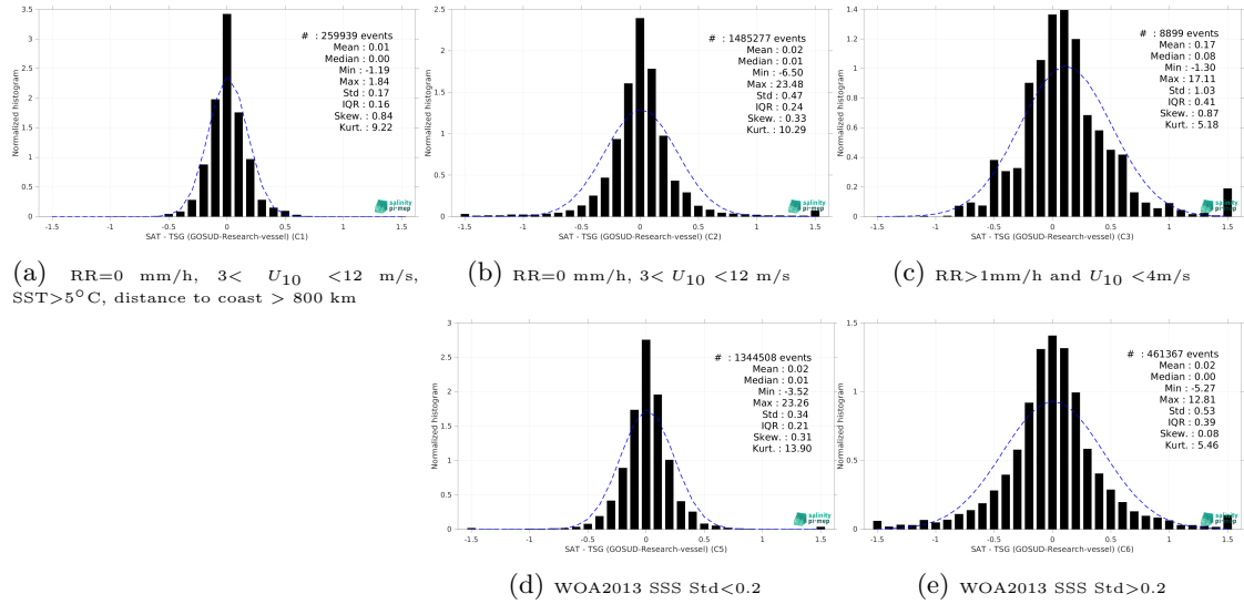
Figure 15: Normalized histogram of \Delta SSS (CCI SSS L4 Merged-OI v5.5 - 7-day running (ESA) - TSG (GOSUD-Research-vessel)) for 5 different subdatasets corresponding to: RR=0 mm/h, 3 < U_{10} < 12 m/s, SST>5°C, distance to coast > 800 km (a), RR=0 mm/h, 3 < U_{10} < 12 m/s (b), RR>1mm/h and U_{10} < 4 m/s (c), WOA2013 SSS Std<0.2 (d), WOA2013 SSS Std>0.2 (e).
