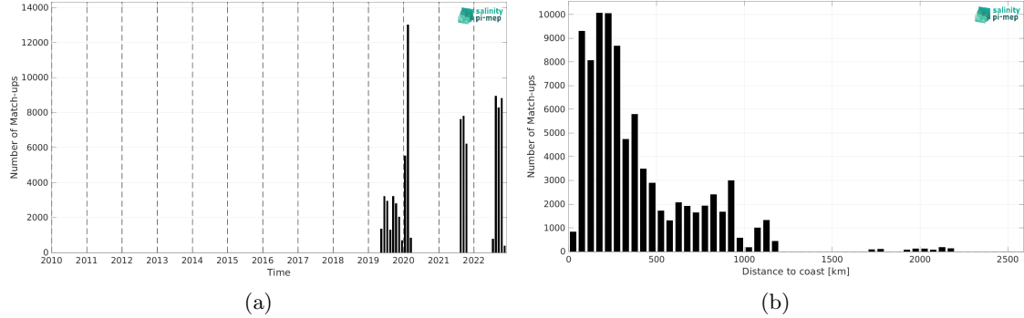
Figure 2: Number of match-ups between Saildrone and CCI SSS L4 Merged-OI v5.5 - 7-day running (ESA) SSS as a function of time (a) and as function of the distance to coast (b) over the Atlantic Ocean Pi-MEP region and for the full satellite product period.
