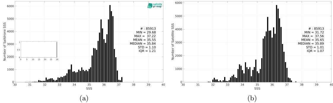
Figure 3: Histograms of SSS from Saildrone (a) and CCI SSS L4 Merged-OI v5.5 - 7-day running (ESA) (b) considering all match-up pairs per bins of 0.1 over the Atlantic Ocean Pi-MEP region and for the full satellite product period.
