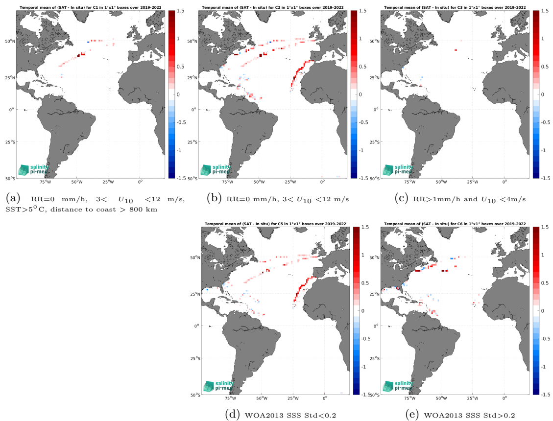
Figure 14: Temporal mean gridded over spatial boxes of size 1^\circ \times 1^\circ of \Delta\text{SSS} (CCI SSS L4 Merged-OI v5.5 - 7-day running (ESA) - Sailability) for 5 different subdatasets corresponding to:RR=0 mm/h, 3 < U_{10} < 12 m/s, SST >5^\circ\text{C} , distance to coast > 800 km (a), RR=0 mm/h, 3 < U_{10} < 12 m/s (b), RR >1 mm/h and U_{10} < 4 m/s (c), WOA2013 SSS Std <0.2 (d), WOA2013 SSS Std >0.2 (e).
