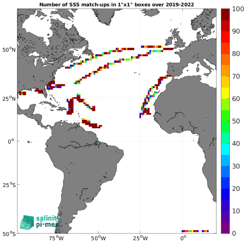
Figure 5: Number of SSS match-ups between Saildrone SSS and the CCI SSS L4 Merged-OI v5.5 - 7-day running (ESA) SSS product for the Atlantic Ocean Pi-MEP region over 1°×1° boxes and for the full satellite product period.
