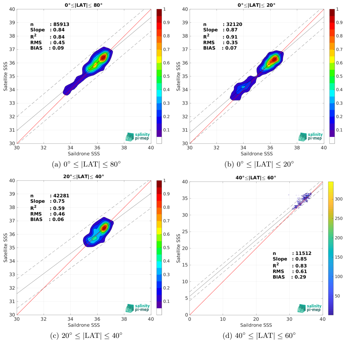
Figure 10: Contour maps of the concentration of CCI SSS L4 Merged-OI v5.5 - 7-day running (ESA) SSS (y-axis) versus Sailability SSS (x-axis) at match-up pairs for different latitude bands. For each plot, the red line shows x=y . The black thin and dashed lines indicate a linear fit through the data cloud and the \pm 95\% confidence levels, respectively. The number match-up pairs n , the slope and R^2 coefficient of the linear fit, the root mean square (RMS) and the mean bias between satellite and in situ data are indicated for each latitude band in each plots.
