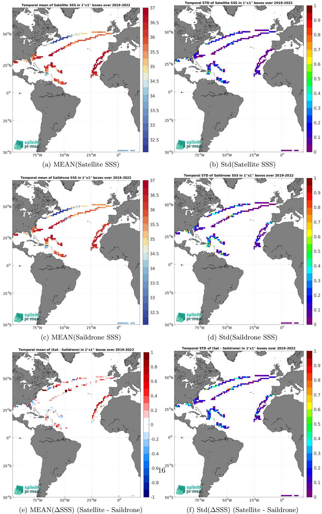
Figure 7: Temporal mean (left) and Std (right) of SSS from CCI SSS L4 Merged-OI v5.5 - 7-day running (ESA) (top), Saildrone (middle), and of \Delta\text{SSS} (Satellite - Saildrone). Only match-up pairs are used to generate these maps.
