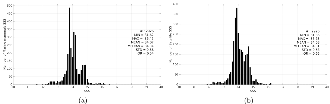
Figure 3: Histograms of SSS from Marine mammals (a) and CCI SSS L4 Merged-OI v5.5 - 7-day running (ESA) (b) considering all match-up pairs per bins of 0.1 over the Atlantic Ocean Pi-MEP region and for the full satellite product period.
