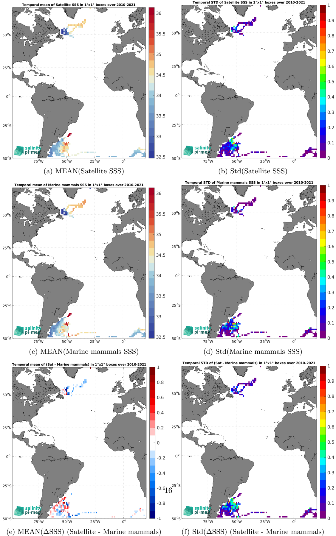
Figure 7: Temporal mean (left) and Std (right) of SSS from CCI SSS L4 Merged-OI v5.5 - 7-day running (ESA) (top), Marine mammals (middle), and of \Delta SSS (Satellite - Marine mammals). Only match-up pairs are used to generate these maps.
