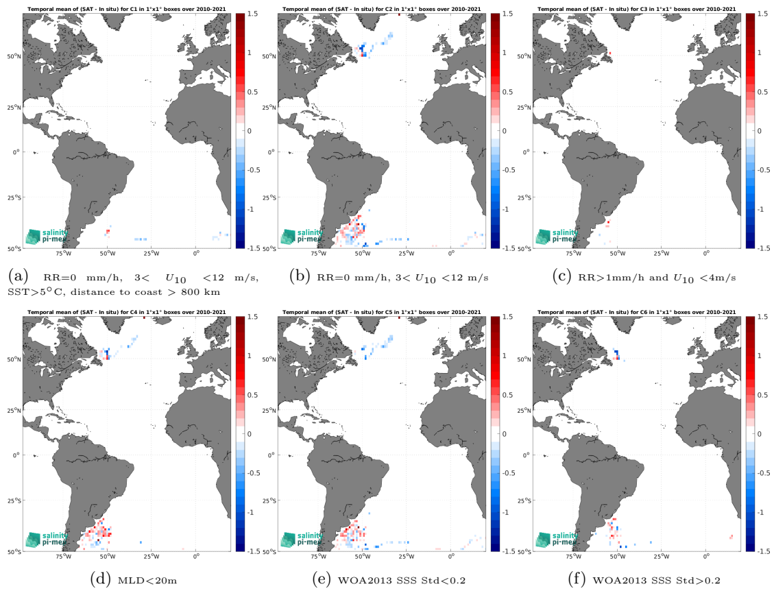
Figure 14: Temporal mean gridded over spatial boxes of size 1^\circ \times 1^\circ of \Delta SSS (CCI SSS L4 Merged-OI v5.5 - 7-day running (ESA) - Marine mammals) for 6 different subdatasets corresponding to:RR=0 mm/h, 3 < U_{10} < 12 m/s, SST >5^\circ C, distance to coast > 800 km (a), RR=0 mm/h, 3 < U_{10} < 12 m/s (b), RR >1 mm/h and U_{10} < 4 m/s (c),MLD <20 m (d),WOA2013 SSS Std <0.2 (e),WOA2013 SSS Std >0.2 (f).
