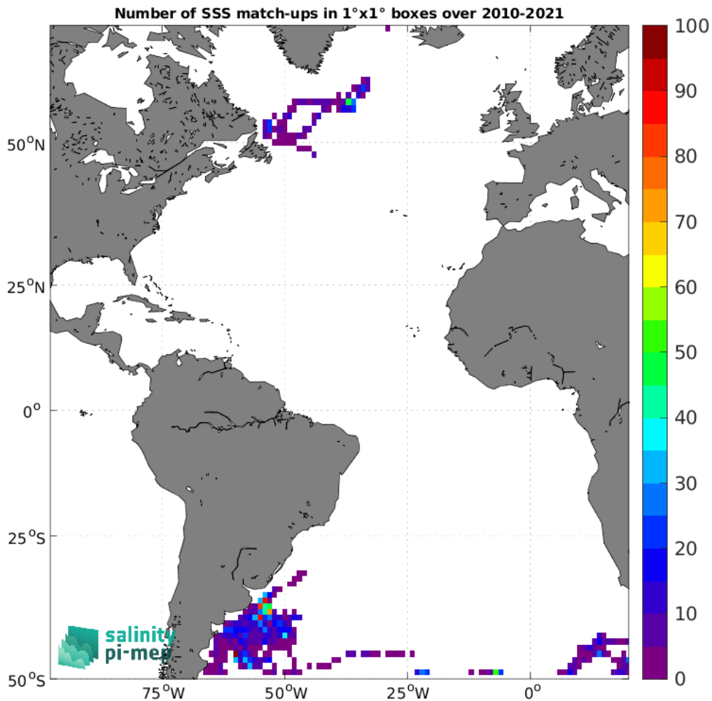
Figure 5: Number of SSS match-ups between Marine mammals SSS and the CCI SSS L4 Merged-OI v5.5 - 7-day running (ESA) SSS product for the Atlantic Ocean Pi-MEP region over 1°x1° boxes and for the full satellite product period.
