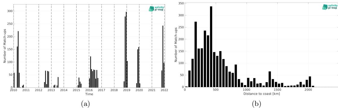
Figure 2: Number of match-ups between Marine mammals and CCI SSS L4 Merged-OI v5.5 - 7-day running (ESA) SSS as a function of time (a) and as function of the distance to coast (b) over the Atlantic Ocean Pi-MEP region and for the full satellite product period.
