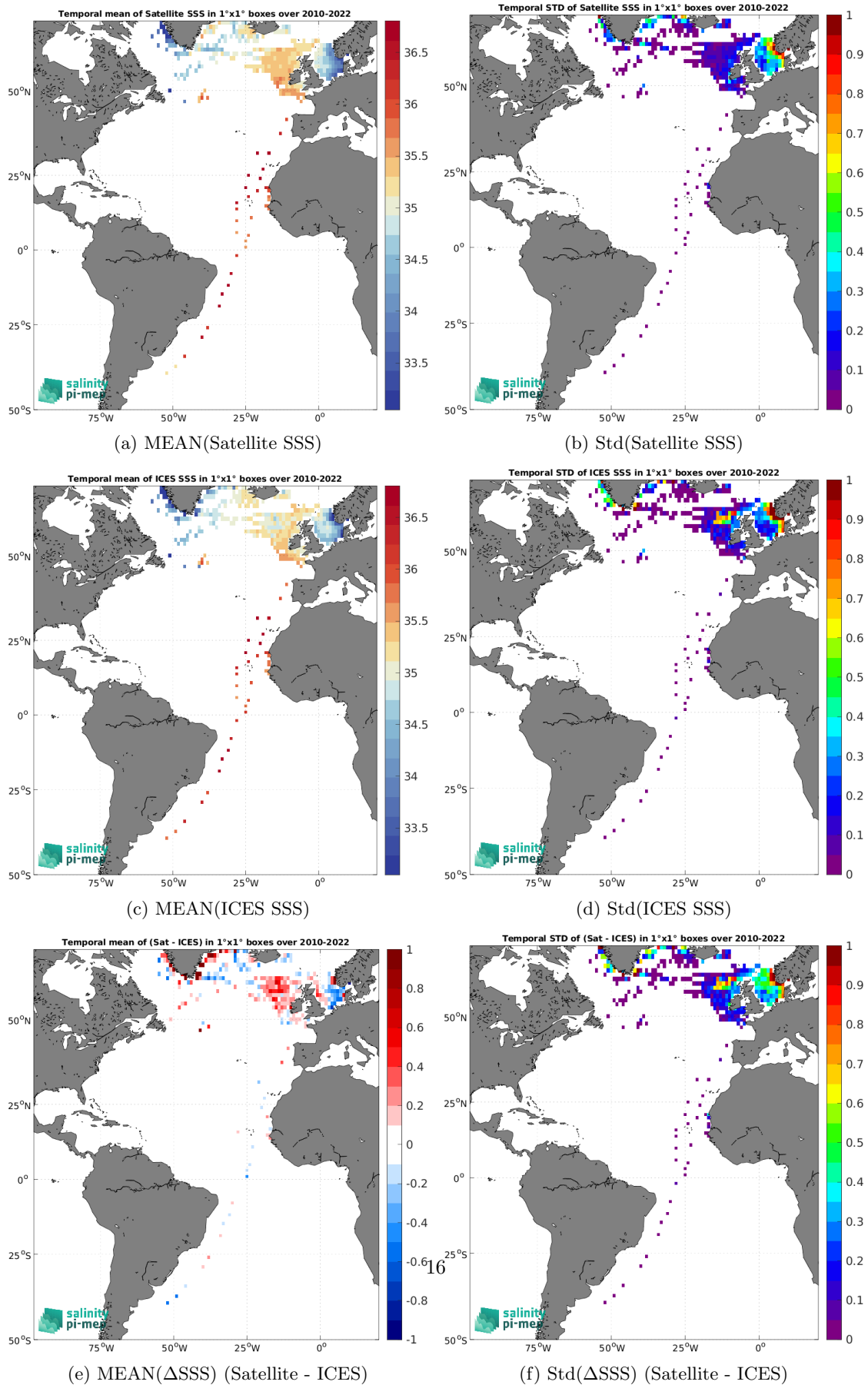
Figure 7: Temporal mean (left) and Std (right) of SSS from CCI SSS L4 Merged-OI v5.5 - 7-day running (ESA) (top), ICES (middle), and of \Delta\text{SSS} (Satellite - ICES). Only match-up pairs are used to generate these maps.
