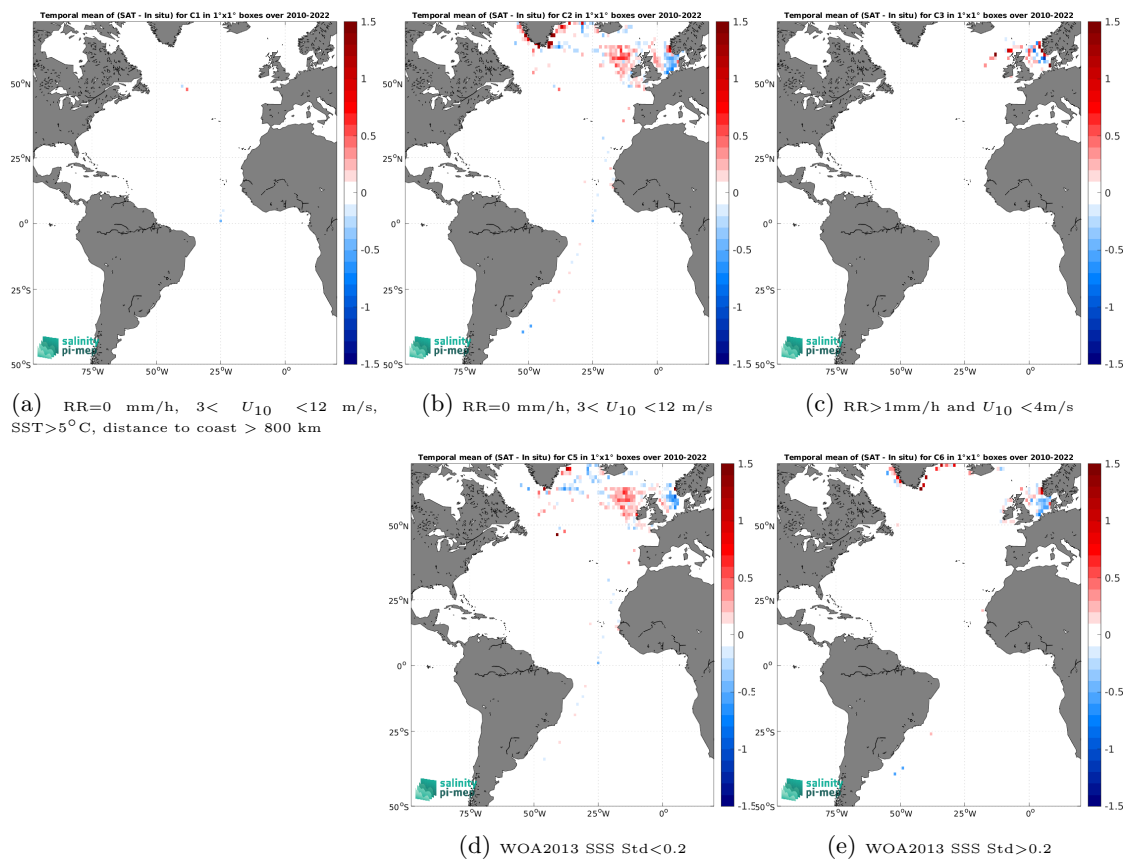
Figure 14: Temporal mean gridded over spatial boxes of size 1^\circ \times 1^\circ of \Delta\text{SSS} (CCI SSS L4 Merged-OI v5.5 - 7-day running (ESA) - ICES) for 5 different subdatasets corresponding to:RR=0 mm/h, 3 < U_{10} < 12 m/s, SST>5°C, distance to coast > 800 km (a), RR=0 mm/h, 3 < U_{10} < 12 m/s (b), RR>1mm/h and U_{10} < 4 m/s (c), WOA2013 SSS Std<0.2 (d), WOA2013 SSS Std>0.2 (e).
