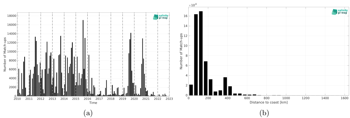
Figure 2: Number of match-ups between ICES and CCI SSS L4 Merged-OI v5.5 - 7-day running (ESA) SSS as a function of time (a) and as function of the distance to coast (b) over the Atlantic Ocean Pi-MEP region and for the full satellite product period.
