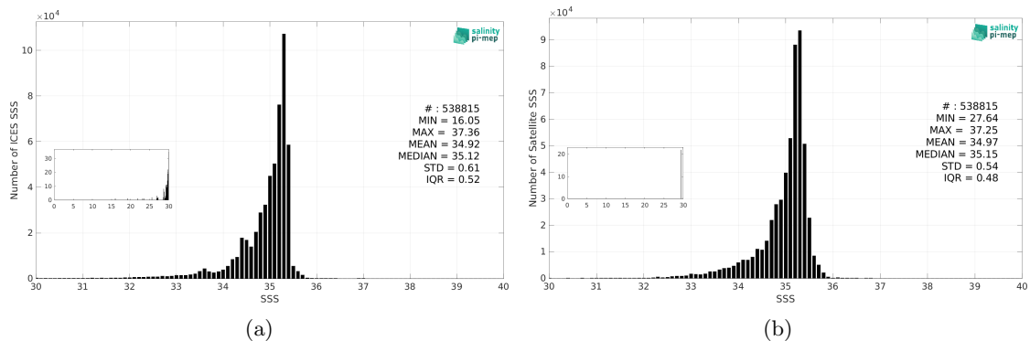
Figure 3: Histograms of SSS from ICES (a) and CCI SSS L4 Merged-OI v5.5 - 7-day running (ESA) (b) considering all match-up pairs per bins of 0.1 over the Atlantic Ocean Pi-MEP region and for the full satellite product period.
