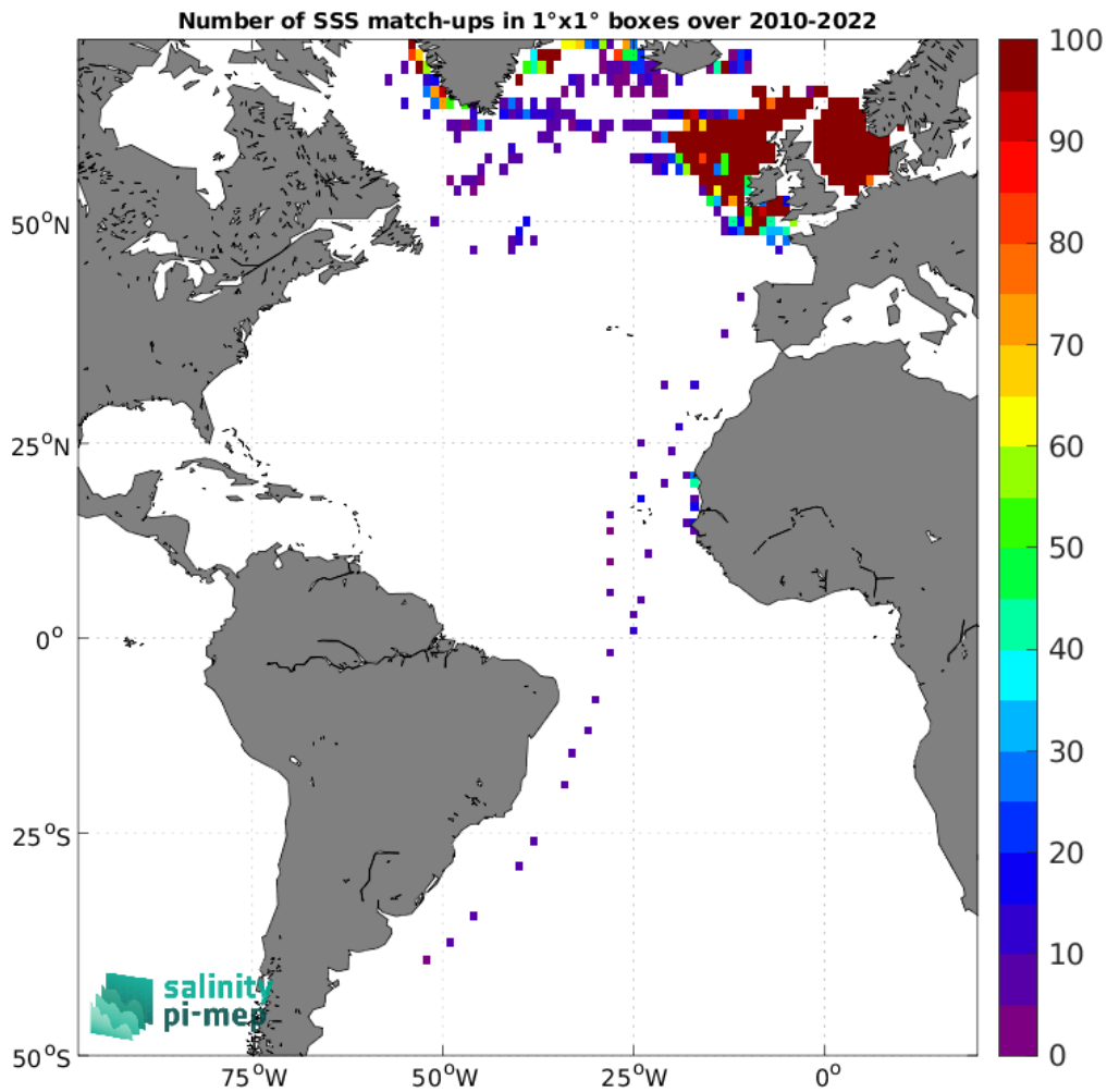
Figure 5: Number of SSS match-ups between ICES SSS and the CCI SSS L4 Merged-OI v5.5 - 7-day running (ESA) SSS product for the Atlantic Ocean Pi-MEP region over 1^\circ \times 1^\circ boxes and for the full satellite product period.
