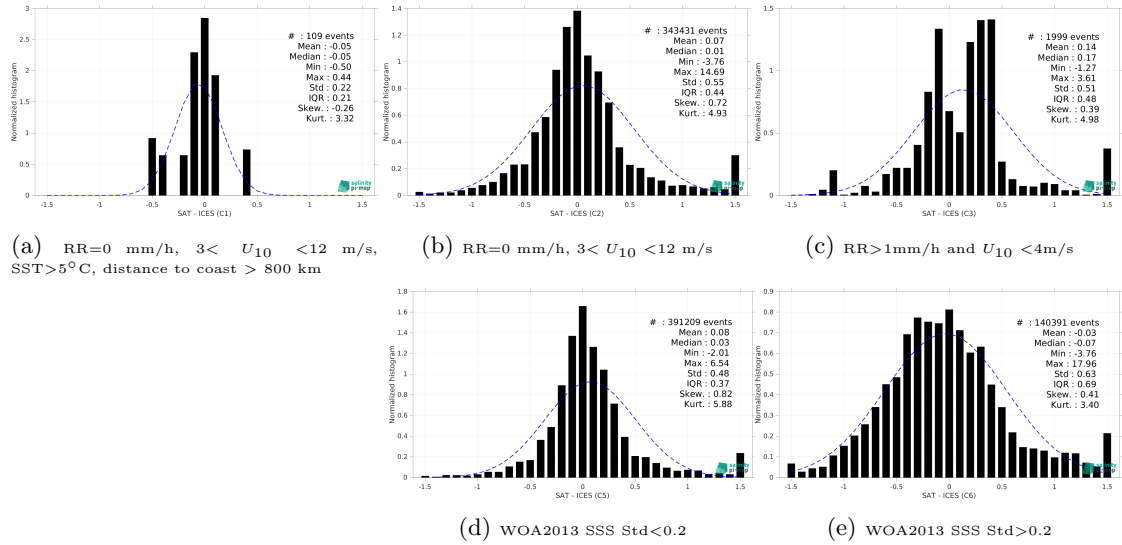
Figure 15: Normalized histogram of \Delta\text{SSS} (CCI SSS L4 Merged-OI v5.5 - 7-day running (ESA) - ICES) for 5 different subdatasets corresponding to: RR=0 mm/h, 3 < U_{10} < 12 m/s, SST>5°C, distance to coast > 800 km (a), RR=0 mm/h, 3 < U_{10} < 12 m/s (b), RR>1mm/h and U_{10} < 4 m/s (c), WOA2013 SSS Std<0.2 (d), WOA2013 SSS Std>0.2 (e).
