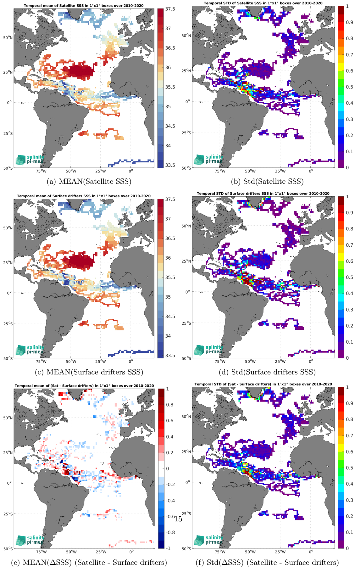
Figure 6: Temporal mean (left) and Std (right) of SSS from CCI SSS L4 Merged-OI v5.5 - 7-day running (ESA) (top), Surface drifters (middle), and of \Delta SSS (Satellite - Surface drifters). Only match-up pairs are used to generate these maps.
