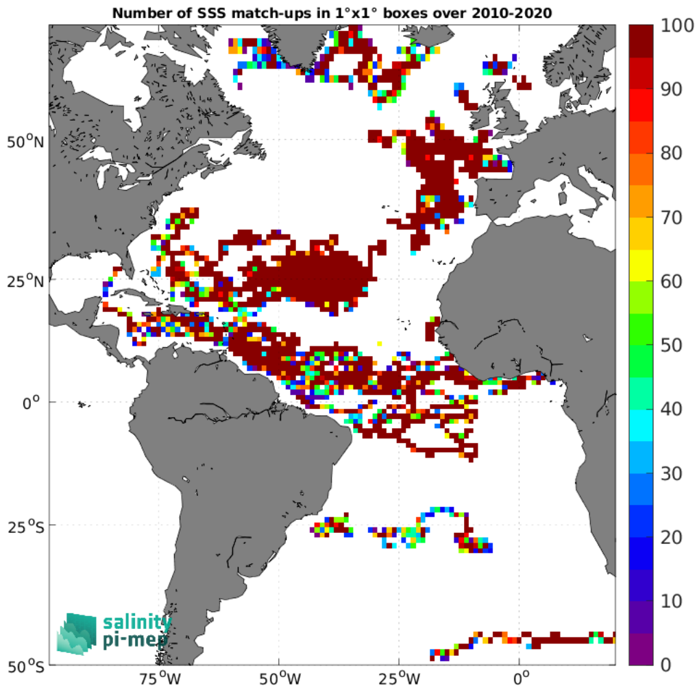
Figure 4: Number of SSS match-ups between Surface drifters SSS and the CCI SSS L4 Merged-OI v5.5 - 7-day running (ESA) SSS product for the Atlantic Ocean Pi-MEP region over 1^\circ \times 1^\circ boxes and for the full satellite product period.
