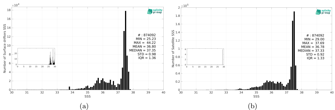
Figure 3: Histograms of SSS from Surface drifters (a) and CCI SSS L4 Merged-OI v5.5 - 7-day running (ESA) (b) considering all match-up pairs per bins of 0.1 over the Atlantic Ocean Pi-MEP region and for the full satellite product period.
