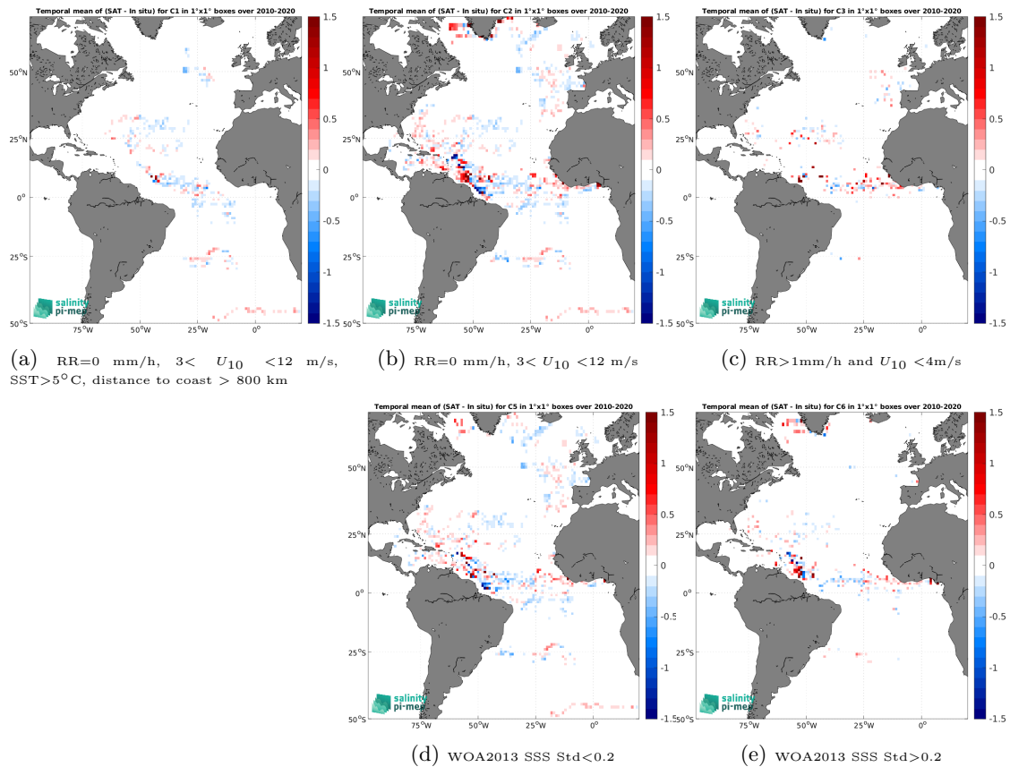
Figure 13: Temporal mean gridded over spatial boxes of size 1^\circ \times 1^\circ of \Delta\text{SSS} (CCI SSS L4 Merged-OI v5.5 - 7-day running (ESA) - Surface drifters) for 5 different subdatasets corresponding to:RR=0 mm/h, 3 < U_{10} < 12 m/s, SST >5^\circ\text{C} , distance to coast > 800 km (a), RR=0 mm/h, 3 < U_{10} < 12 m/s (b), RR >1 mm/h and U_{10} < 4 m/s (c), WOA2013 SSS Std <0.2 (d), WOA2013 SSS Std >0.2 (e).
