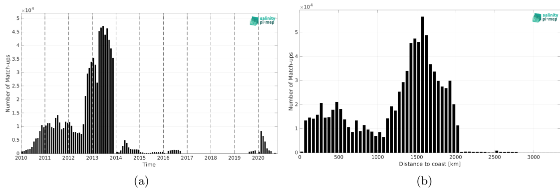
Figure 2: Number of match-ups between Surface drifters and CCI SSS L4 Merged-OI v5.5 - 7-day running (ESA) SSS as a function of time (a) and as function of the distance to coast (b) over the Atlantic Ocean Pi-MEP region and for the full satellite product period.
