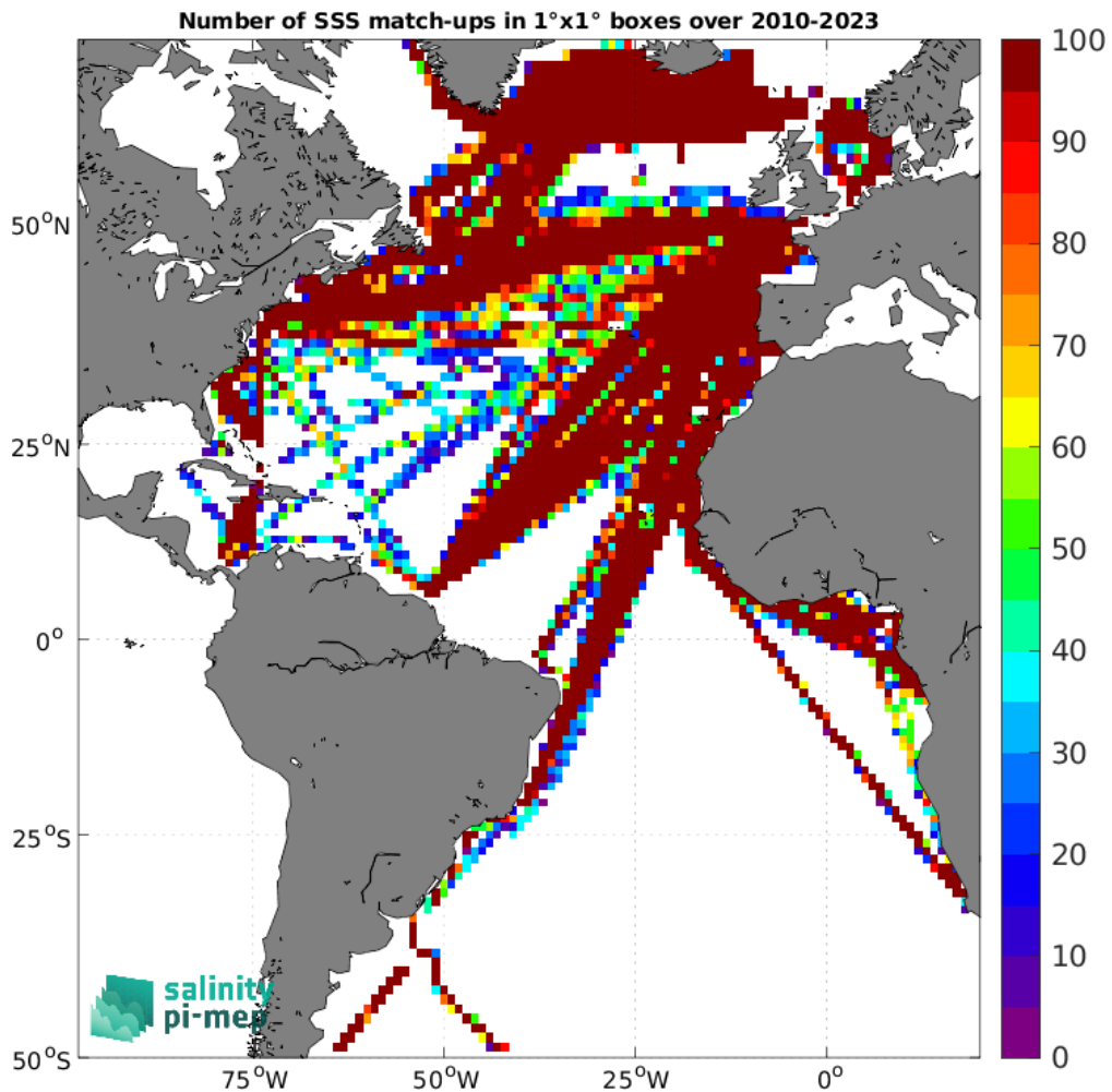
Figure 5: Number of SSS match-ups between TSG (LEGOS-DM) SSS and the CCI SSS L4 Merged-OI v5.5 - 30-day running (ESA) SSS product for the Atlantic Ocean Pi-MEP region over 1^\circ \times 1^\circ boxes and for the full satellite product period.
