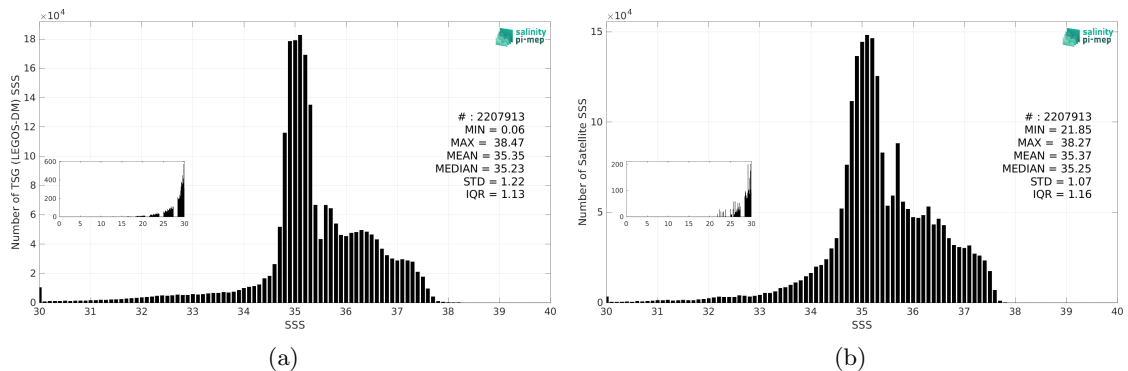
Figure 3: Histograms of SSS from TSG (LEGOS-DM) (a) and CCI SSS L4 Merged-OI v5.5 - 30-day running (ESA) (b) considering all match-up pairs per bins of 0.1 over the Atlantic Ocean Pi-MEP region and for the full satellite product period.
