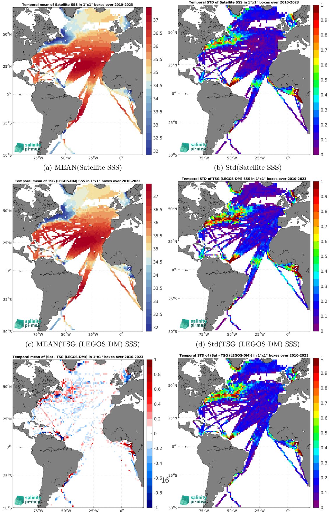
Figure 7: Temporal mean (left) and Std (right) of SSS from CCI SSS L4 Merged-OI v5.5 - 30-day running (ESA) (top), TSG (LEGOS-DM) (middle), and of \Delta SSS (Satellite - TSG (LEGOS-DM)). Only match-up pairs are used to generate these maps.
