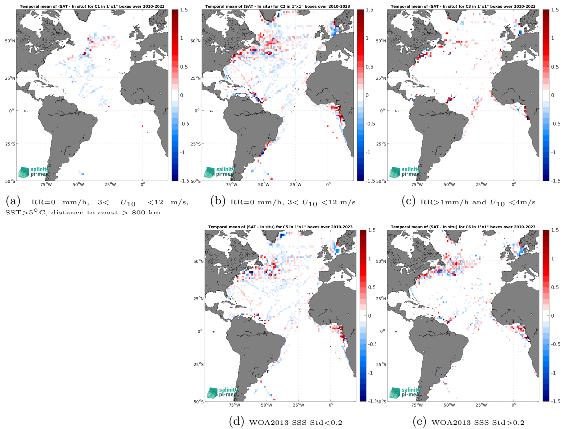
Figure 14: Temporal mean gridded over spatial boxes of size 1^\circ \times 1^\circ of \Delta\text{SSS} (CCI SSS L4 Merged-OI v5.5 - 30-day running (ESA) - TSG (LEGOS-DM)) for 5 different subdatasets corresponding to:RR=0 mm/h, 3 < U_{10} < 12 m/s, SST>5°C, distance to coast > 800 km (a), RR=0 mm/h, 3 < U_{10} < 12 m/s (b), RR>1mm/h and U_{10} < 4 m/s (c), WOA2013 SSS Std<0.2 (d), WOA2013 SSS Std>0.2 (e).
