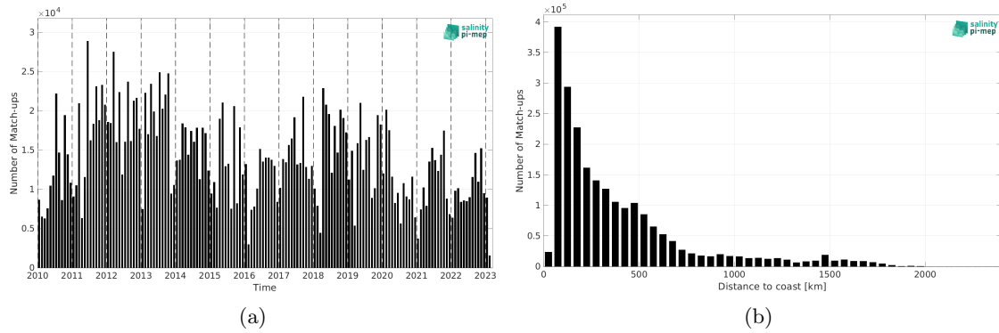
Figure 2: Number of match-ups between TSG (LEGOS-DM) and CCI SSS L4 Merged-OI v5.5 - 30-day running (ESA) SSS as a function of time (a) and as function of the distance to coast (b) over the Atlantic Ocean Pi-MEP region and for the full satellite product period.
