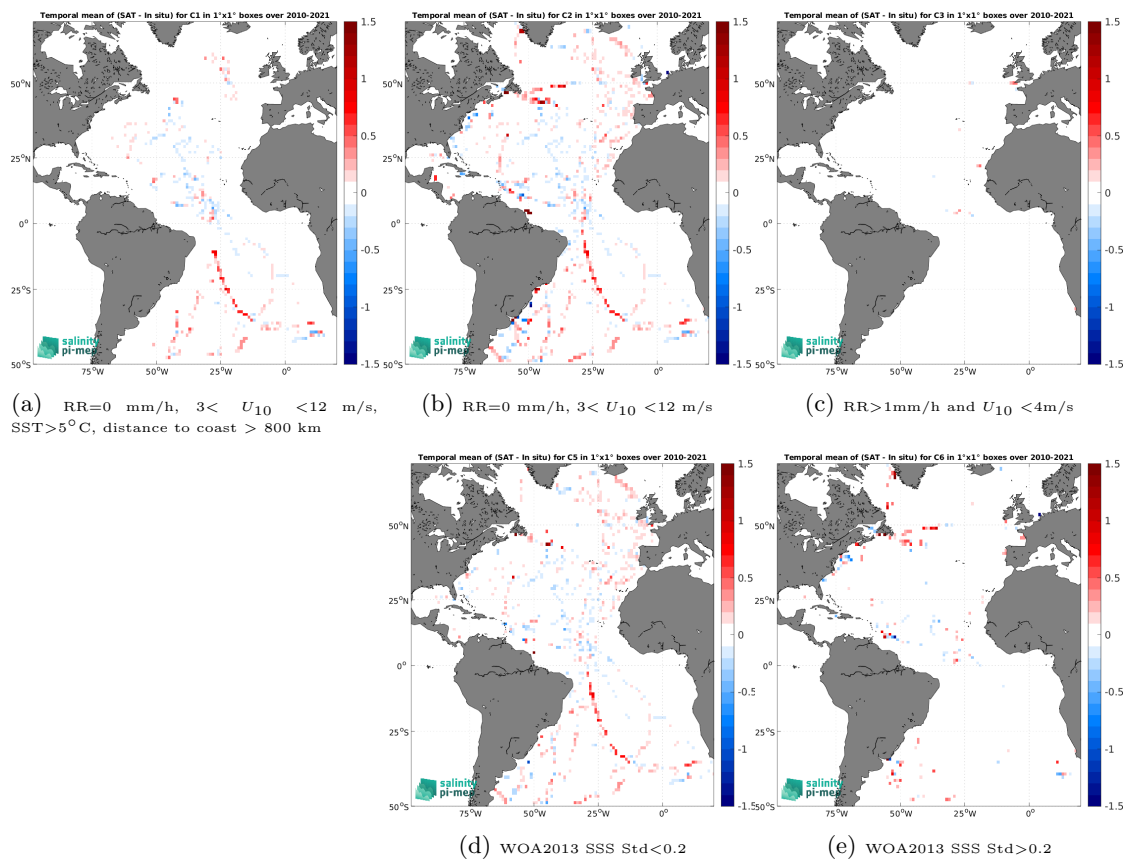
Figure 14: Temporal mean gridded over spatial boxes of size 1^\circ \times 1^\circ of \Delta\text{SSS} (CCI SSS L4 Merged-OI v5.5 - 30-day running (ESA) - TSG (GOSUD-Sailing-ship)) for 5 different subdatasets corresponding to:RR=0 mm/h, 3 < U_{10} < 12 m/s, SST >5^\circ\text{C} , distance to coast > 800 km (a), RR=0 mm/h, 3 < U_{10} < 12 m/s (b), RR >1 mm/h and U_{10} < 4 m/s (c), WOA2013 SSS Std <0.2 (d), WOA2013 SSS Std >0.2 (e).
