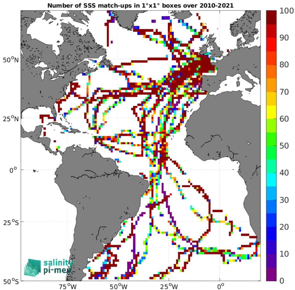
Figure 5: Number of SSS match-ups between TSG (GOSUD-Sailing-ship) SSS and the CCI SSS L4 Merged-OI v5.5 - 30-day running (ESA) SSS product for the Atlantic Ocean Pi-MEP region over 1°x1° boxes and for the full satellite product period.
