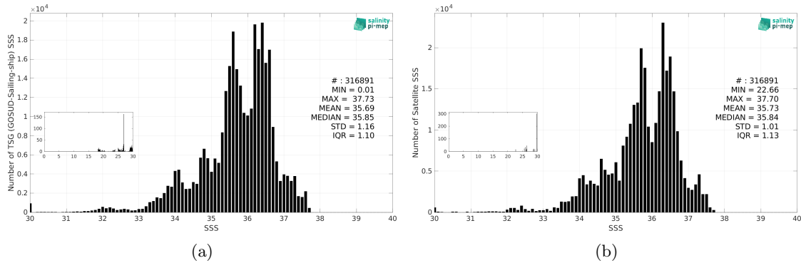
Figure 3: Histograms of SSS from TSG (GOSUD-Sailing-ship) (a) and CCI SSS L4 Merged-OI v5.5 - 30-day running (ESA) (b) considering all match-up pairs per bins of 0.1 over the Atlantic Ocean Pi-MEP region and for the full satellite product period.
