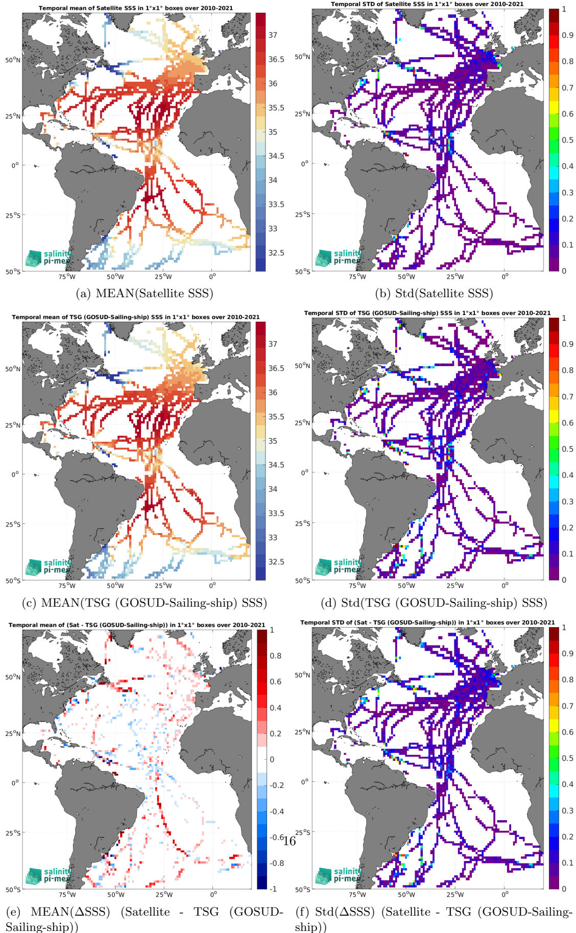
Figure 7: Temporal mean (left) and Std (right) of SSS from CCI SSS L4 Merged-OI v5.5 - 30-day running (ESA) (top), TSG (GOSUD-Sailing-ship) (middle), and of \Delta SSS (Satellite - TSG (GOSUD-Sailing-ship)). Only match-up pairs are used to generate these maps.
