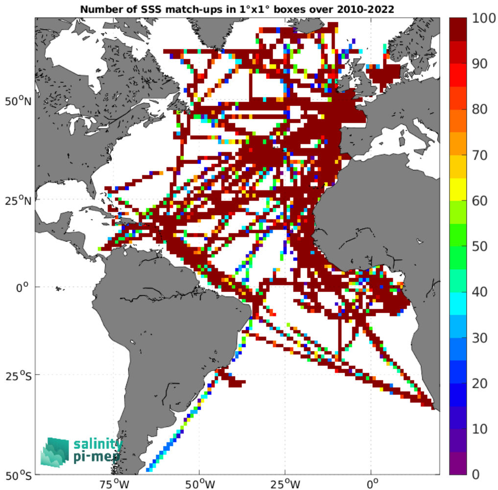
Figure 5: Number of SSS match-ups between TSG (GOSUD-Research-vessel) SSS and the CCI SSS L4 Merged-OI v5.5 - 30-day running (ESA) SSS product for the Atlantic Ocean Pi-MEP region over 1°x1° boxes and for the full satellite product period.
