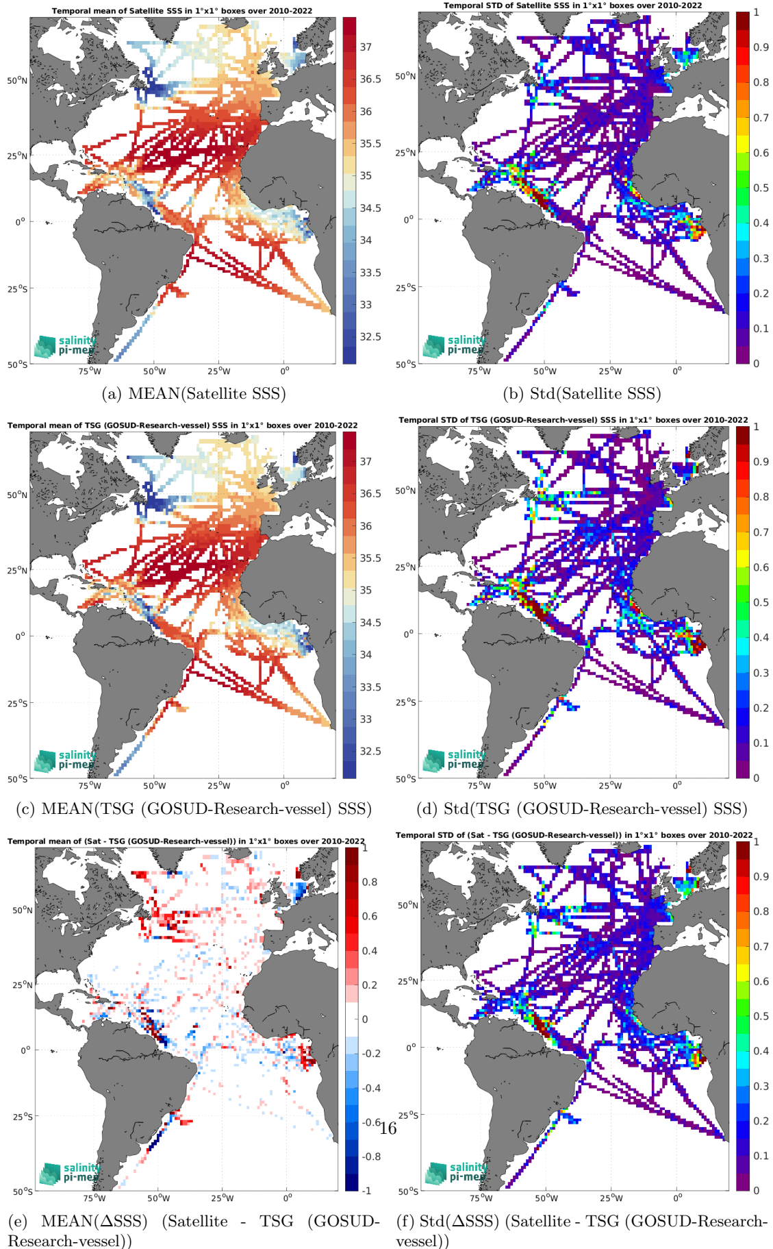
Figure 7: Temporal mean (left) and Std (right) of SSS from CCI SSS L4 Merged-OI v5.5 - 30-day running (ESA) (top), TSG (GOSUD-Research-vessel) (middle), and of \Delta SSS (Satellite - TSG (GOSUD-Research-vessel)). Only match-up pairs are used to generate these maps.
