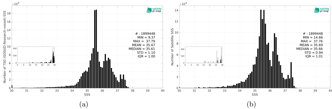
Figure 3: Histograms of SSS from TSG (GOSUD-Research-vessel) (a) and CCI SSS L4 Merged-OI v5.5 - 30-day running (ESA) (b) considering all match-up pairs per bins of 0.1 over the Atlantic Ocean Pi-MEP region and for the full satellite product period.
