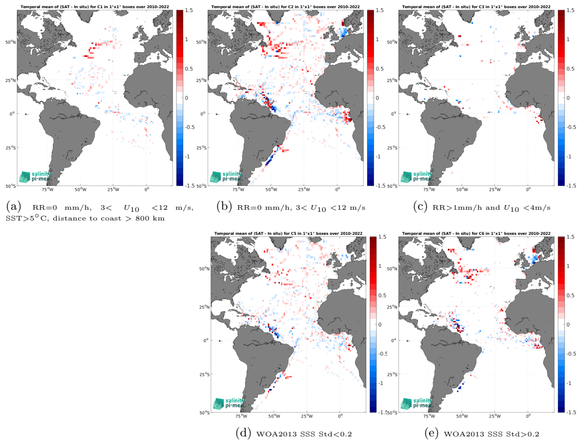
Figure 14: Temporal mean gridded over spatial boxes of size 1^\circ \times 1^\circ of \Delta\text{SSS} (CCI SSS L4 Merged-OI v5.5 - 30-day running (ESA) - TSG (GOSUD-Research-vessel)) for 5 different subdatasets corresponding to:RR=0 mm/h, 3 < U_{10} < 12 m/s, SST >5^\circ\text{C} , distance to coast > 800 km (a), RR=0 mm/h, 3 < U_{10} < 12 m/s (b), RR >1 mm/h and U_{10} < 4 m/s (c), WOA2013 SSS Std <0.2 (d), WOA2013 SSS Std >0.2 (e).
