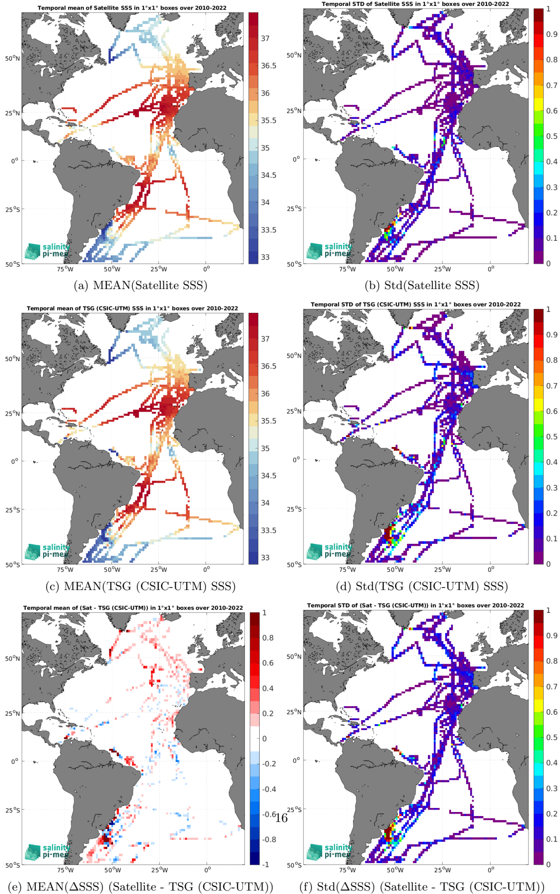
Figure 7: Temporal mean (left) and Std (right) of SSS from CCI SSS L4 Merged-OI v5.5 - 30-day running (ESA) (top), TSG (CSIC-UTM) (middle), and of \Delta SSS (Satellite - TSG (CSIC-UTM)). Only match-up pairs are used to generate these maps.
