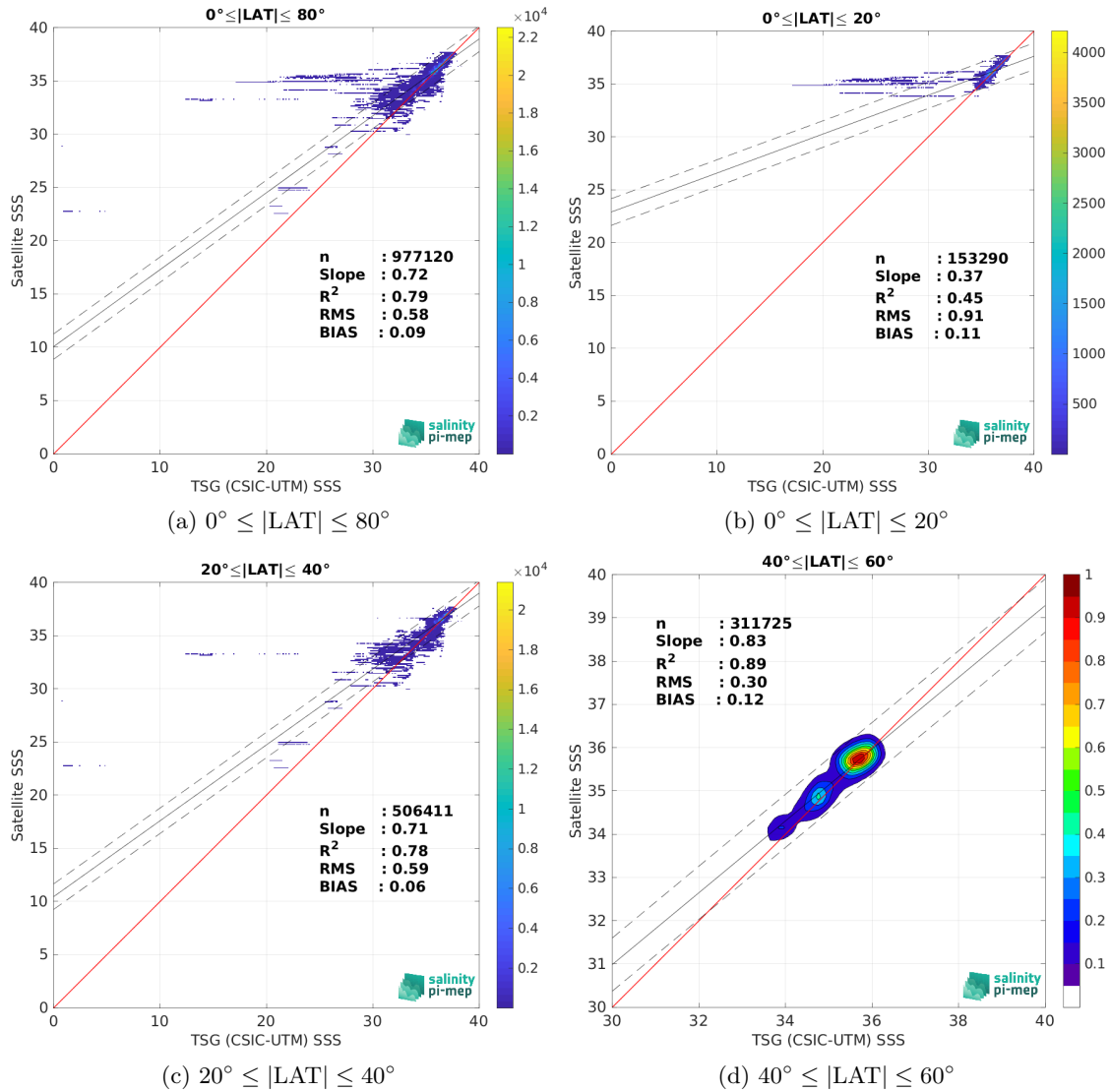
Figure 10: Contour maps of the concentration of CCI SSS L4 Merged-OI v5.5 - 30-day running (ESA) SSS (y-axis) versus TSG (CSIC-UTM) SSS (x-axis) at match-up pairs for different latitude bands. For each plot, the red line shows x=y . The black thin and dashed lines indicate a linear fit through the data cloud and the \pm 95\% confidence levels, respectively. The number match-up pairs n , the slope and R^2 coefficient of the linear fit, the root mean square (RMS) and the mean bias between satellite and in situ data are indicated for each latitude band in each plots.
