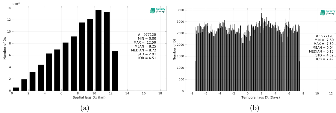
Figure 6: Histograms of the spatial (a) and temporal (b) lags between the location/time of the TSG (CSIC-UTM) measurement and the date of the corresponding CCI SSS L4 Merged-OI v5.5 - 30-day running (ESA) SSS pixel.
