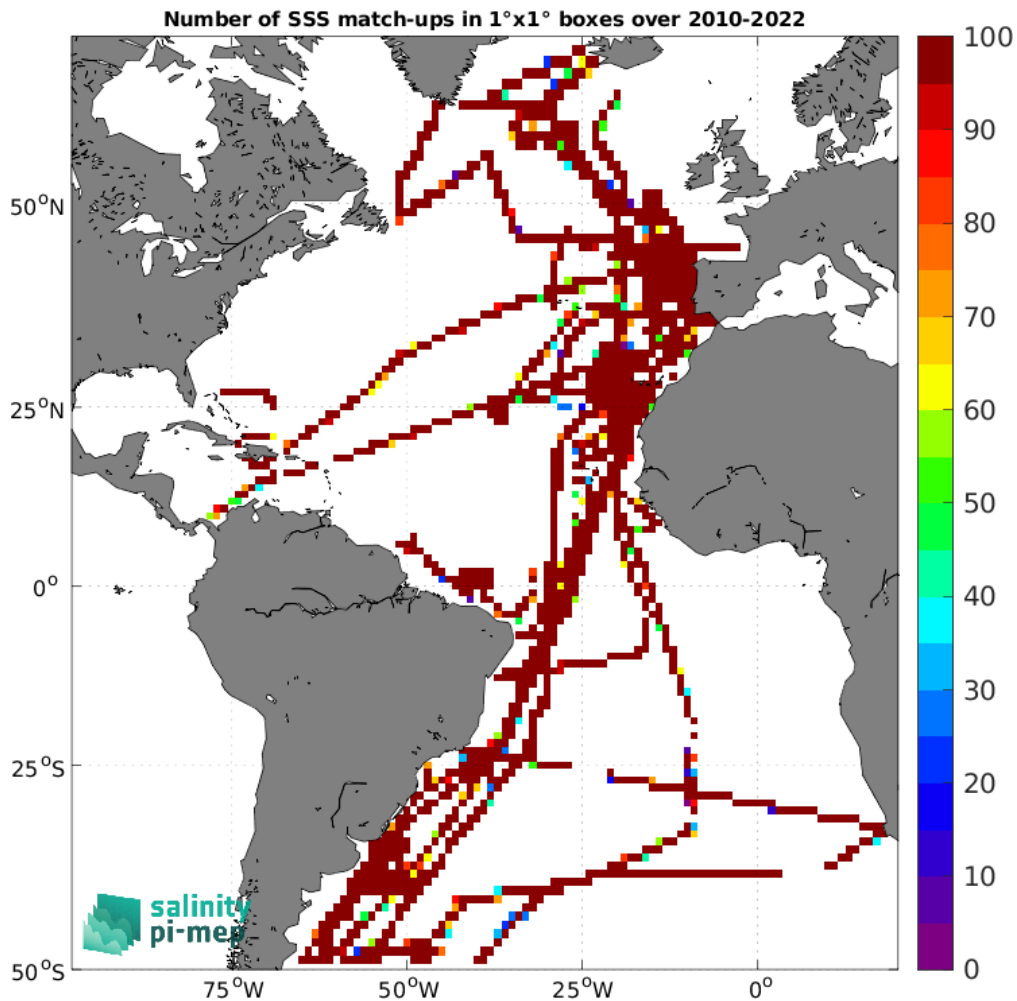
Figure 5: Number of SSS match-ups between TSG (CSIC-UTM) SSS and the CCI SSS L4 Merged-OI v5.5 - 30-day running (ESA) SSS product for the Atlantic Ocean Pi-MEP region over 1^\circ \times 1^\circ boxes and for the full satellite product period.
