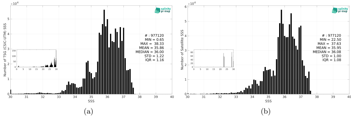
Figure 3: Histograms of SSS from TSG (CSIC-UTM) (a) and CCI SSS L4 Merged-OI v5.5 - 30-day running (ESA) (b) considering all match-up pairs per bins of 0.1 over the Atlantic Ocean Pi-MEP region and for the full satellite product period.
