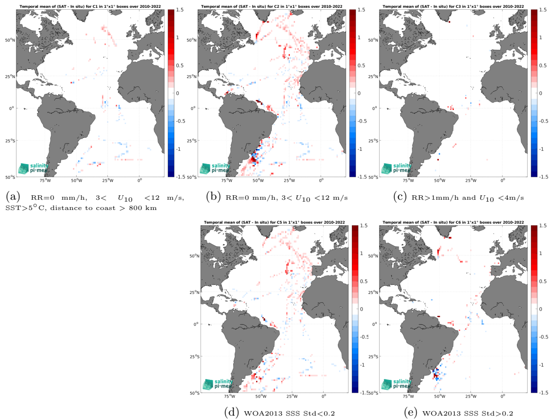
Figure 14: Temporal mean gridded over spatial boxes of size 1^\circ \times 1^\circ of \Delta\text{SSS} (CCI SSS L4 Merged-OI v5.5 - 30-day running (ESA) - TSG (CSIC-UTM)) for 5 different subdatasets corresponding to:RR=0 mm/h, 3 < U_{10} < 12 m/s, SST>5°C, distance to coast > 800 km (a), RR=0 mm/h, 3 < U_{10} < 12 m/s (b), RR>1mm/h and U_{10} < 4 m/s (c), WOA2013 SSS Std<0.2 (d), WOA2013 SSS Std>0.2 (e).
