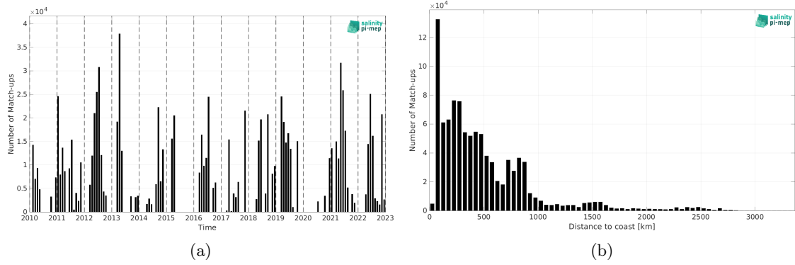
Figure 2: Number of match-ups between TSG (CSIC-UTM) and CCI SSS L4 Merged-OI v5.5 - 30-day running (ESA) SSS as a function of time (a) and as function of the distance to coast (b) over the Atlantic Ocean Pi-MEP region and for the full satellite product period.
