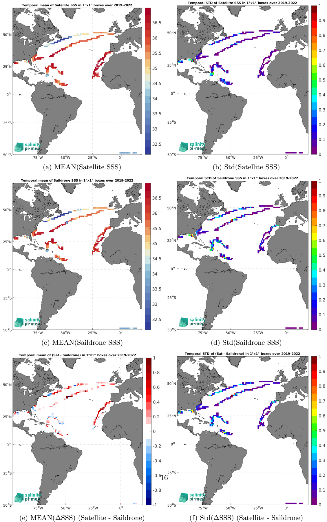
Figure 7: Temporal mean (left) and Std (right) of SSS from CCI SSS L4 Merged-OI v5.5 - 30-day running (ESA) (top), Saildrone (middle), and of \Delta SSS (Satellite - Saildrone). Only match-up pairs are used to generate these maps.
