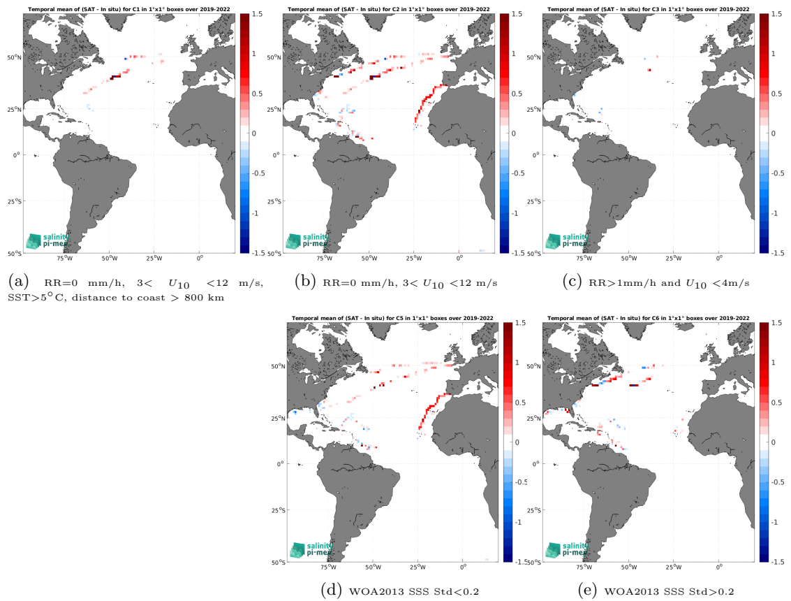
Figure 14: Temporal mean gridded over spatial boxes of size 1^\circ \times 1^\circ of \Delta SSS (CCI SSS L4 Merged-OI v5.5 - 30-day running (ESA) - Saildrone) for 5 different subdatasets corresponding to:RR=0 mm/h, 3 < U_{10} < 12 m/s, SST >5^\circ C, distance to coast > 800 km (a), RR=0 mm/h, 3 < U_{10} < 12 m/s (b), RR >1 mm/h and U_{10} < 4 m/s (c), WOA2013 SSS Std <0.2 (d), WOA2013 SSS Std >0.2 (e).
