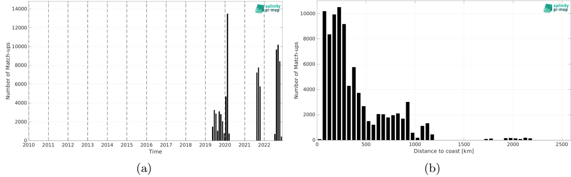
Figure 2: Number of match-ups between Saildrone and CCI SSS L4 Merged-OI v5.5 - 30-day running (ESA) SSS as a function of time (a) and as function of the distance to coast (b) over the Atlantic Ocean Pi-MEP region and for the full satellite product period.
