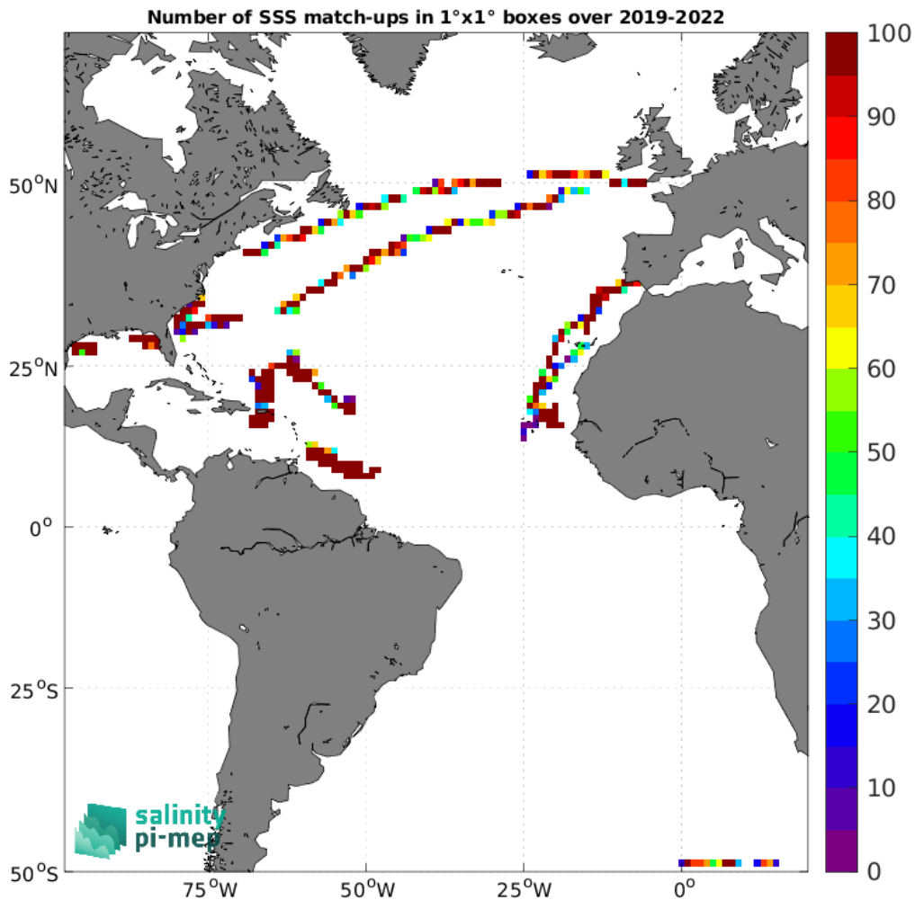
Figure 5: Number of SSS match-ups between Saildrone SSS and the CCI SSS L4 Merged-OI v5.5 - 30-day running (ESA) SSS product for the Atlantic Ocean Pi-MEP region over 1^\circ \times 1^\circ boxes and for the full satellite product period.
