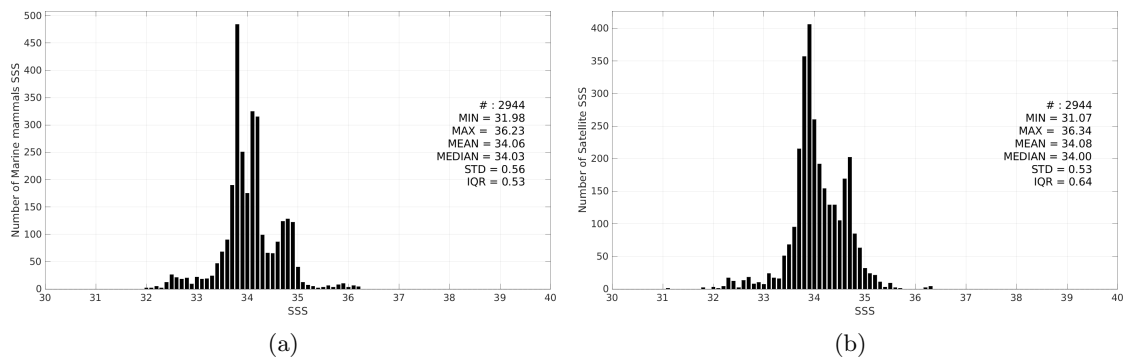
Figure 3: Histograms of SSS from Marine mammals (a) and CCI SSS L4 Merged-OI v5.5 - 30-day running (ESA) (b) considering all match-up pairs per bins of 0.1 over the Atlantic Ocean Pi-MEP region and for the full satellite product period.
