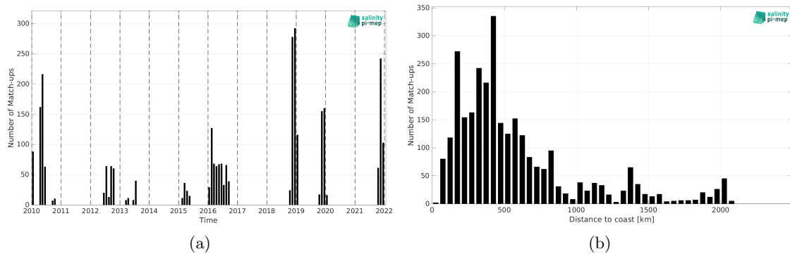
Figure 2: Number of match-ups between Marine mammals and CCI SSS L4 Merged-OI v5.5 - 30-day running (ESA) SSS as a function of time (a) and as function of the distance to coast (b) over the Atlantic Ocean Pi-MEP region and for the full satellite product period.
