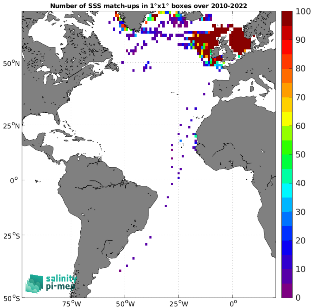
Figure 5: Number of SSS match-ups between ICES SSS and the CCI SSS L4 Merged-OI v5.5 - 30-day running (ESA) SSS product for the Atlantic Ocean Pi-MEP region over 1^\circ \times 1^\circ boxes and for the full satellite product period.
