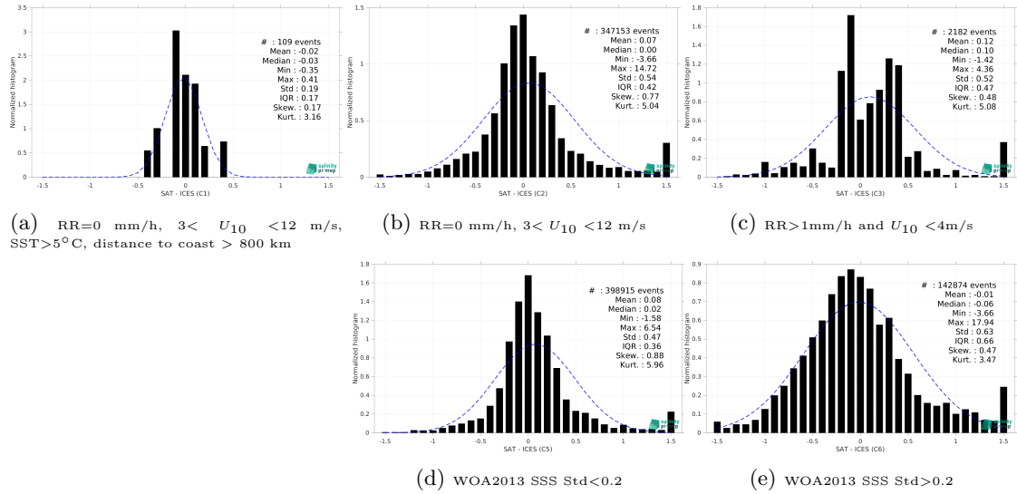
Figure 15: Normalized histogram of \Delta\text{SSS} (CCI SSS L4 Merged-OI v5.5 - 30-day running (ESA) - ICES) for 5 different subdatasets corresponding to: RR=0 mm/h, 3 < U_{10} < 12 m/s, SST>5°C, distance to coast > 800 km (a), RR=0 mm/h, 3 < U_{10} < 12 m/s (b), RR>1mm/h and U_{10} < 4 m/s (c), WOA2013 SSS Std<0.2 (d), WOA2013 SSS Std>0.2 (e).
