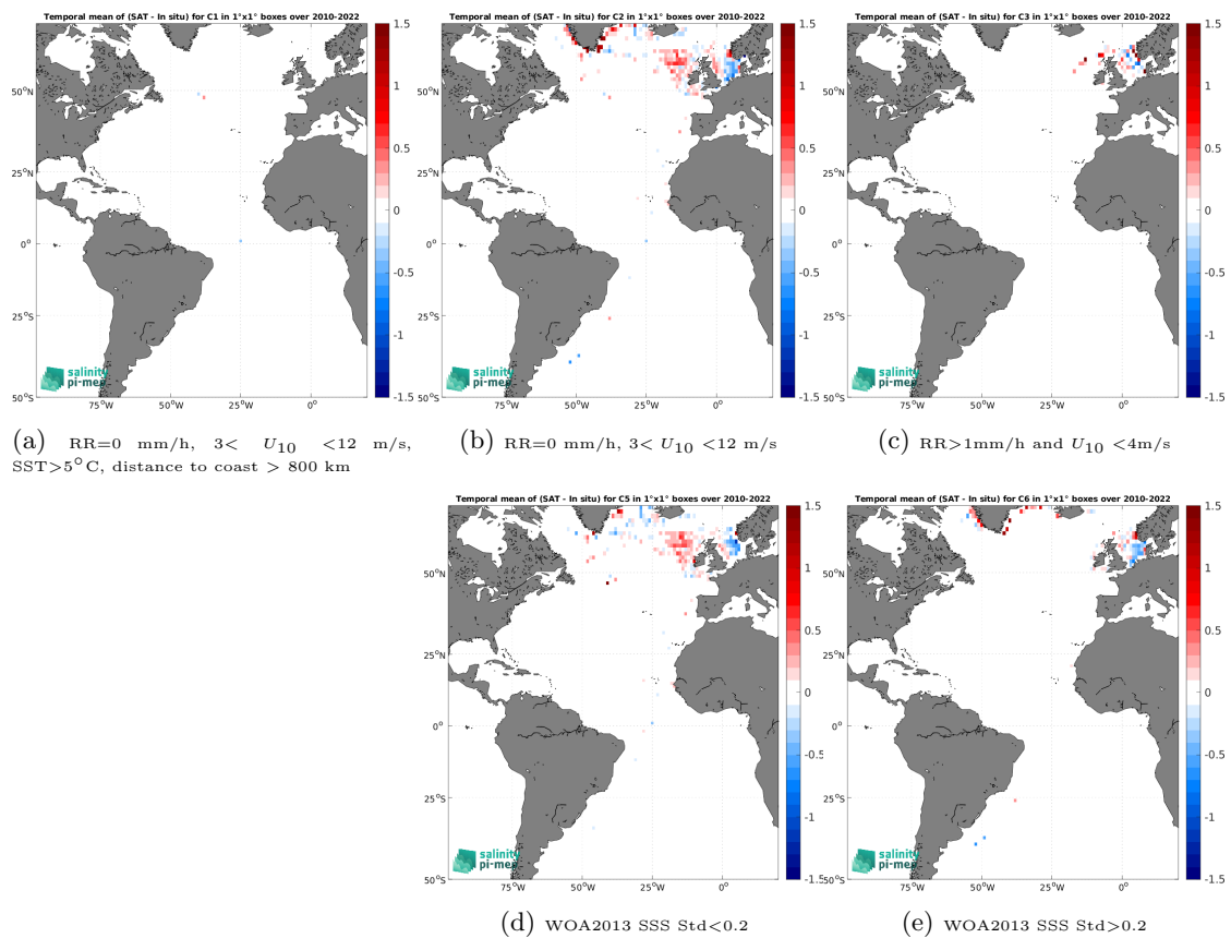
Figure 14: Temporal mean gridded over spatial boxes of size 1^\circ \times 1^\circ of \Delta\text{SSS} (CCI SSS L4 Merged-OI v5.5 - 30-day running (ESA) - ICES) for 5 different subdatasets corresponding to:RR=0 mm/h, 3 < U_{10} < 12 m/s, SST >5^\circ\text{C} , distance to coast > 800 km (a), RR=0 mm/h, 3 < U_{10} < 12 m/s (b), RR >1 mm/h and U_{10} < 4 m/s (c), WOA2013 SSS Std <0.2 (d), WOA2013 SSS Std >0.2 (e).
