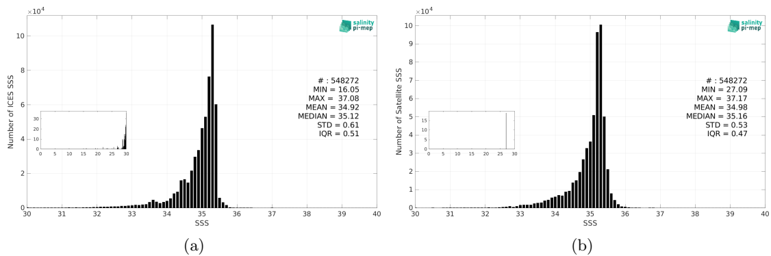
Figure 3: Histograms of SSS from ICES (a) and CCI SSS L4 Merged-OI v5.5 - 30-day running (ESA) (b) considering all match-up pairs per bins of 0.1 over the Atlantic Ocean Pi-MEP region and for the full satellite product period.
