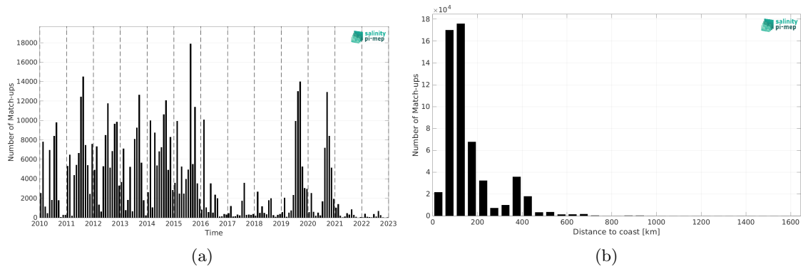
Figure 2: Number of match-ups between ICES and CCI SSS L4 Merged-OI v5.5 - 30-day running (ESA) SSS as a function of time (a) and as function of the distance to coast (b) over the Atlantic Ocean Pi-MEP region and for the full satellite product period.
