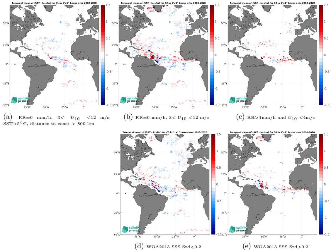
Figure 13: Temporal mean gridded over spatial boxes of size 1^\circ \times 1^\circ of \Delta\text{SSS} (CCI SSS L4 Merged-OI v5.5 - 30-day running (ESA) - Surface drifters) for 5 different subdatasets corresponding to:RR=0 mm/h, 3 < U_{10} < 12 m/s, SST >5^\circ\text{C} , distance to coast > 800 km (a), RR=0 mm/h, 3 < U_{10} < 12 m/s (b), RR >1 mm/h and U_{10} < 4 m/s (c), WOA2013 SSS Std <0.2 (d), WOA2013 SSS Std >0.2 (e).
