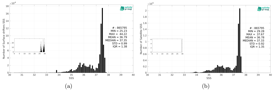
Figure 3: Histograms of SSS from Surface drifters (a) and CCI SSS L4 Merged-OI v5.5 - 30-day running (ESA) (b) considering all match-up pairs per bins of 0.1 over the Atlantic Ocean Pi-MEP region and for the full satellite product period.
