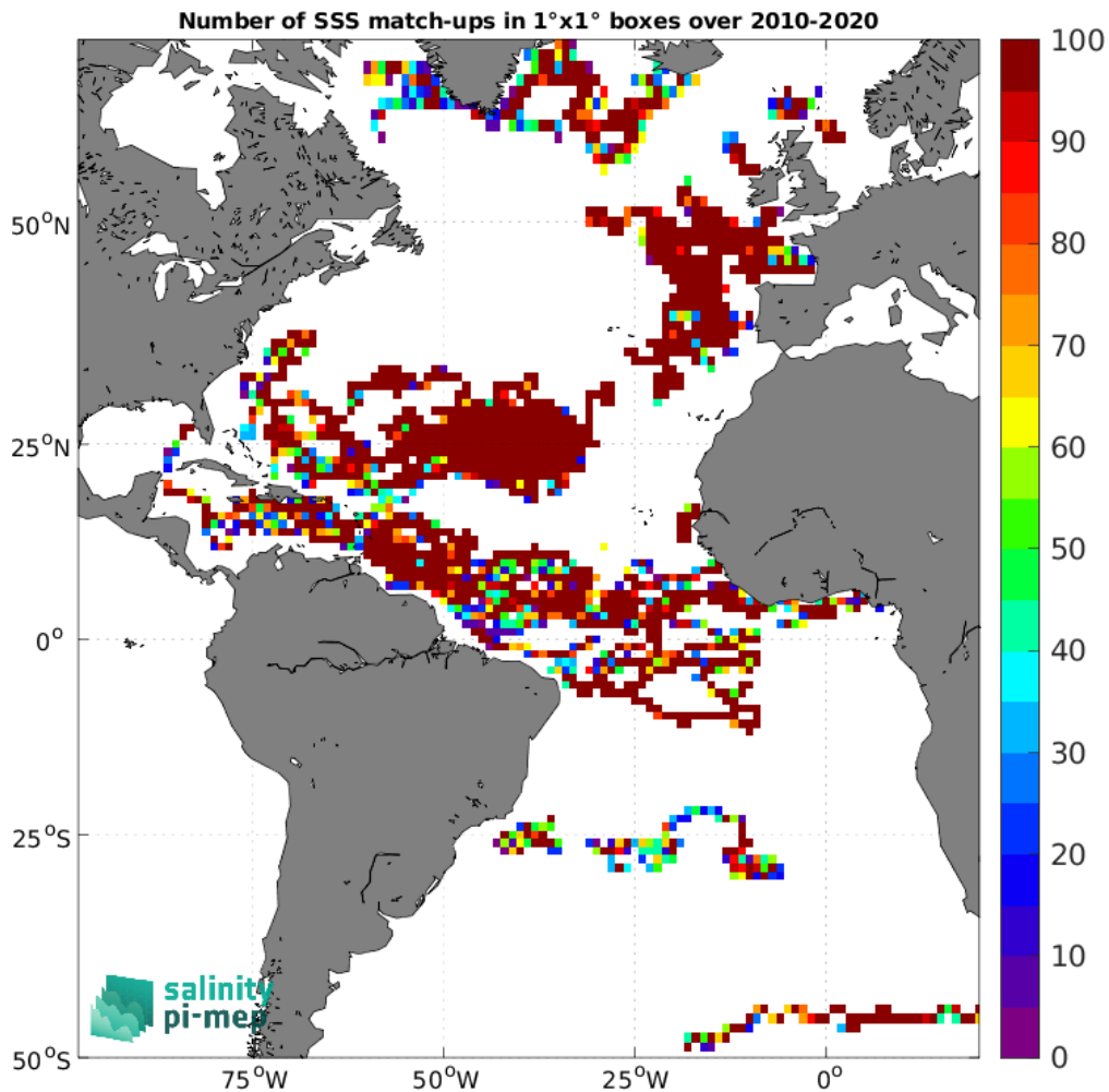
Figure 4: Number of SSS match-ups between Surface drifters SSS and the CCI SSS L4 Merged-OI v5.5 - 30-day running (ESA) SSS product for the Atlantic Ocean Pi-MEP region over 1^\circ \times 1^\circ boxes and for the full satellite product period.
