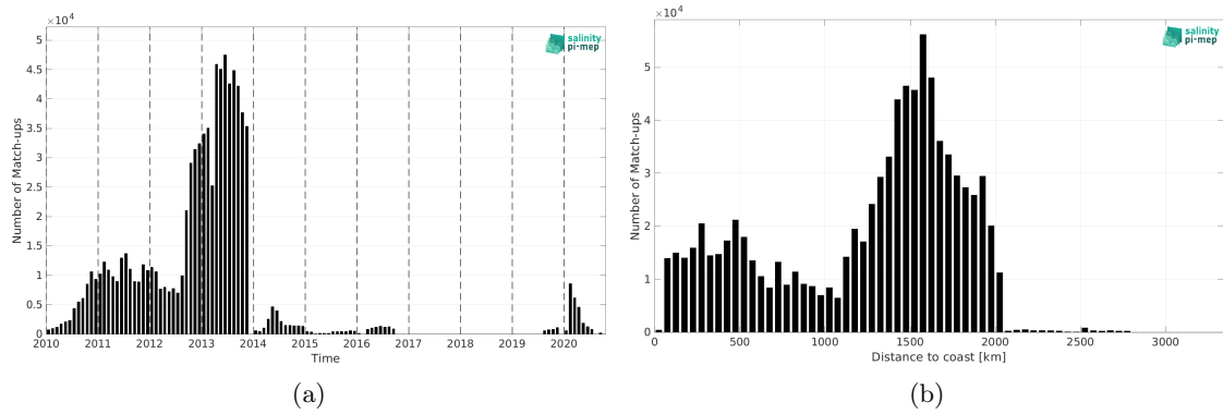
Figure 2: Number of match-ups between Surface drifters and CCI SSS L4 Merged-OI v5.5 - 30-day running (ESA) SSS as a function of time (a) and as function of the distance to coast (b) over the Atlantic Ocean Pi-MEP region and for the full satellite product period.
