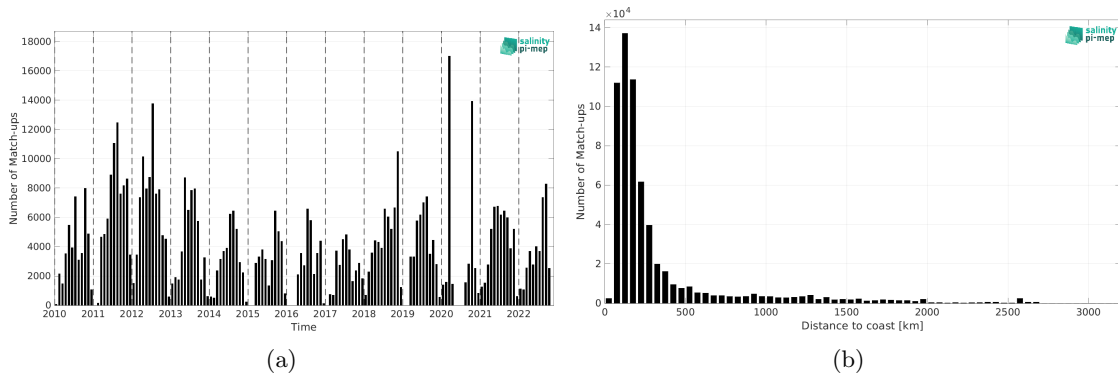
Figure 2: Number of match-ups between TSG (SAMOS) and CCI SSS L4 Merged-OI v4.41 - 7-day running (ESA) SSS as a function of time (a) and as function of the distance to coast (b) over the Atlantic Ocean Pi-MEP region and for the full satellite product period.
