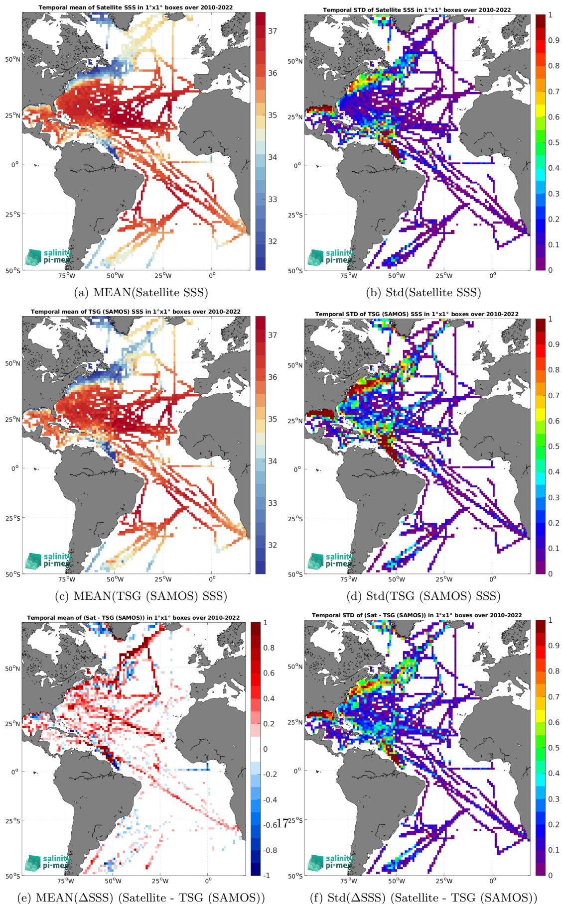
Figure 7: Temporal mean (left) and Std (right) of SSS from CCI SSS L4 Merged-OI v4.41 - 7-day running (ESA) (top), TSG (SAMOS) (middle), and of \Delta SSS (Satellite - TSG (SAMOS)). Only match-up pairs are used to generate these maps.
