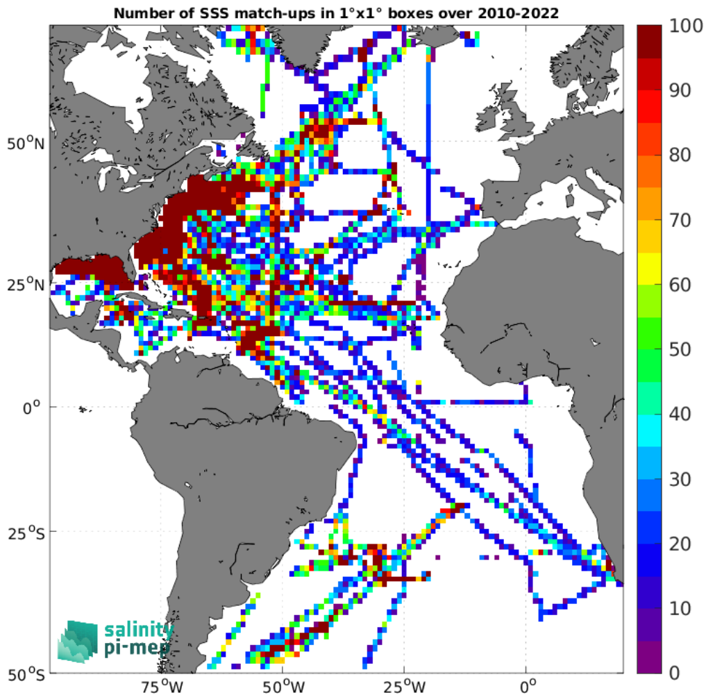
Figure 5: Number of SSS match-ups between TSG (SAMOS) SSS and the CCI SSS L4 Merged-OI v4.41 - 7-day running (ESA) SSS product for the Atlantic Ocean Pi-MEP region over 1^\circ \times 1^\circ boxes and for the full satellite product period.
