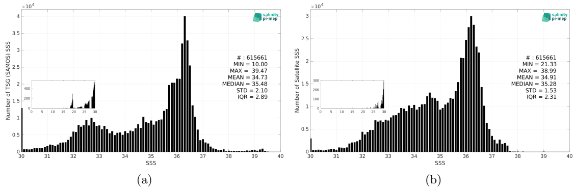
Figure 3: Histograms of SSS from TSG (SAMOS) (a) and CCI SSS L4 Merged-OI v4.41 - 7-day running (ESA) (b) considering all match-up pairs per bins of 0.1 over the Atlantic Ocean Pi-MEP region and for the full satellite product period.
