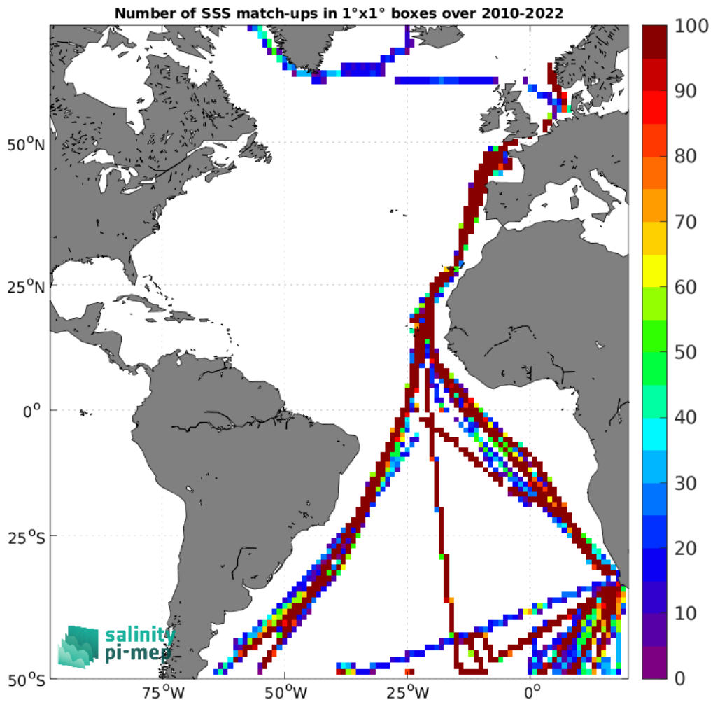
Figure 5: Number of SSS match-ups between TSG (Polarstern) SSS and the CCI SSS L4 Merged-OI v4.41 - 7-day running (ESA) SSS product for the Atlantic Ocean Pi-MEP region over 1°x1° boxes and for the full satellite product period.
