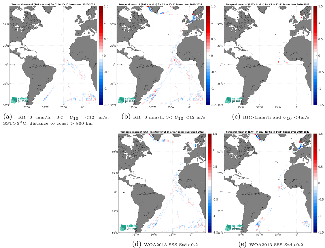
Figure 14: Temporal mean gridded over spatial boxes of size 1^\circ \times 1^\circ of \Delta\text{SSS} (CCI SSS L4 Merged-OI v4.41 - 7-day running (ESA) - TSG (Polarstern)) for 5 different subdatasets corresponding to:RR=0 mm/h, 3 < U_{10} < 12 m/s, SST>5°C, distance to coast > 800 km (a), RR=0 mm/h, 3 < U_{10} < 12 m/s (b), RR>1mm/h and U_{10} < 4 m/s (c), WOA2013 SSS Std<0.2 (d), WOA2013 SSS Std>0.2 (e).
