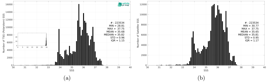
Figure 3: Histograms of SSS from TSG (Polarstern) (a) and CCI SSS L4 Merged-OI v4.41 - 7-day running (ESA) (b) considering all match-up pairs per bins of 0.1 over the Atlantic Ocean Pi-MEP region and for the full satellite product period.
