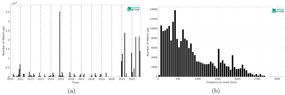
Figure 2: Number of match-ups between TSG (Polarstern) and CCI SSS L4 Merged-OI v4.41 - 7-day running (ESA) SSS as a function of time (a) and as function of the distance to coast (b) over the Atlantic Ocean Pi-MEP region and for the full satellite product period.
