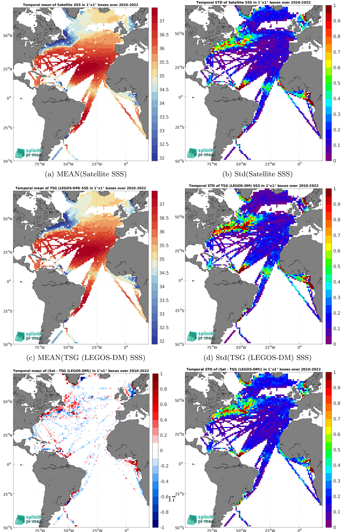
Figure 7: Temporal mean (left) and Std (right) of SSS from CCI SSS L4 Merged-OI v4.41 - 7-day running (ESA) (top), TSG (LEGOS-DM) (middle), and of \Delta SSS (Satellite - TSG (LEGOS-DM)). Only match-up pairs are used to generate these maps.
