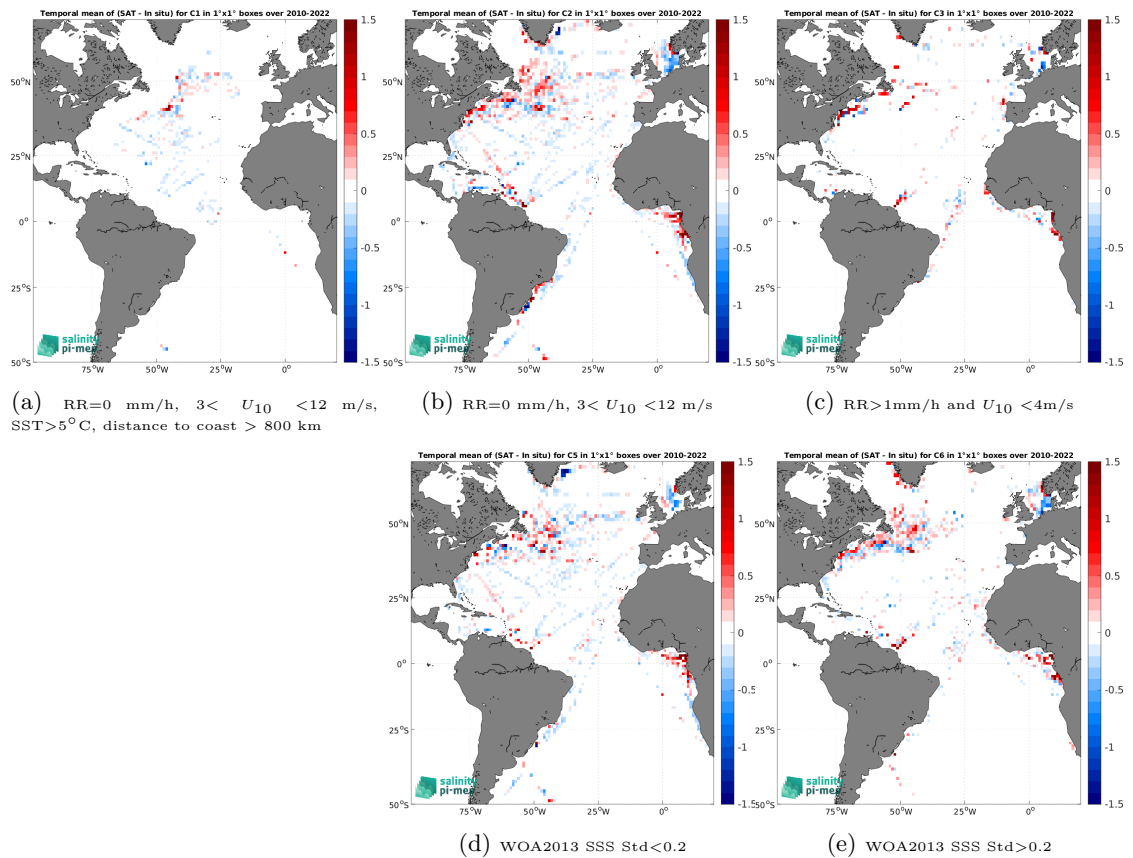
Figure 14: Temporal mean gridded over spatial boxes of size 1^\circ \times 1^\circ of \Delta\text{SSS} (CCI SSS L4 Merged-OI v4.41 - 7-day running (ESA) - TSG (LEGOS-DM)) for 5 different subdatasets corresponding to:RR=0 mm/h, 3 < U_{10} < 12 m/s, SST>5°C, distance to coast > 800 km (a), RR=0 mm/h, 3 < U_{10} < 12 m/s (b), RR>1mm/h and U_{10} < 4 m/s (c), WOA2013 SSS Std<0.2 (d), WOA2013 SSS Std>0.2 (e).
