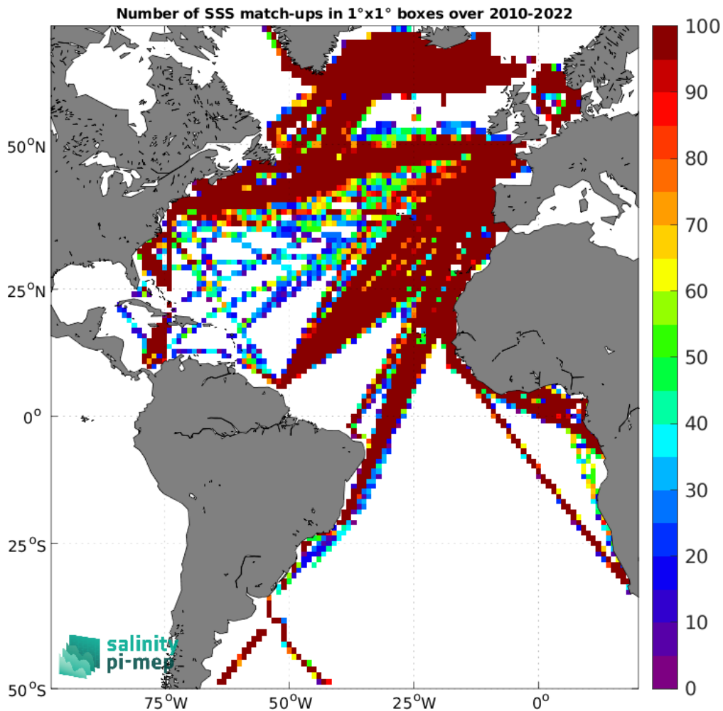
Figure 5: Number of SSS match-ups between TSG (LEGOS-DM) SSS and the CCI SSS L4 Merged-OI v4.41 - 7-day running (ESA) SSS product for the Atlantic Ocean Pi-MEP region over 1^\circ \times 1^\circ boxes and for the full satellite product period.
