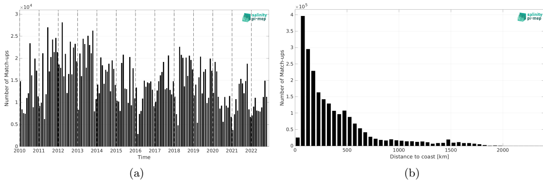
Figure 2: Number of match-ups between TSG (LEGOS-DM) and CCI SSS L4 Merged-OI v4.41 - 7-day running (ESA) SSS as a function of time (a) and as function of the distance to coast (b) over the Atlantic Ocean Pi-MEP region and for the full satellite product period.
