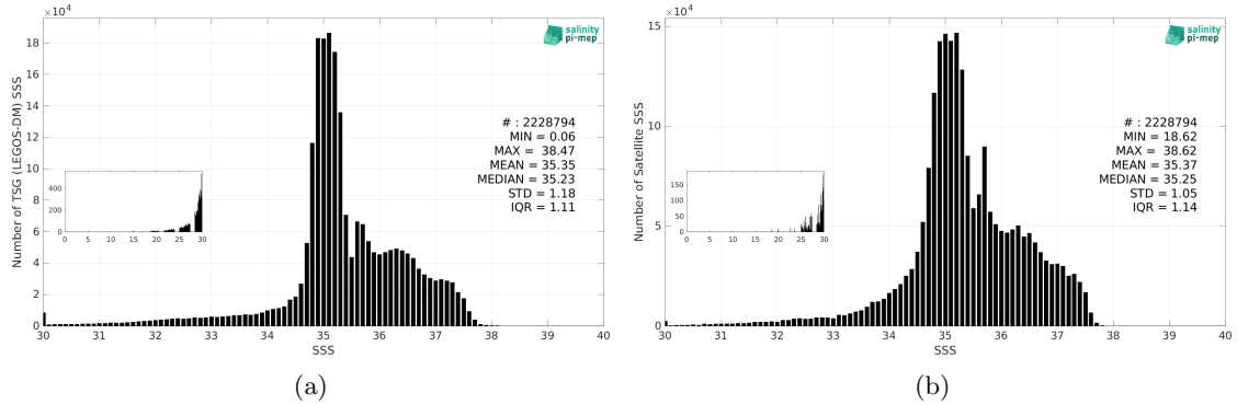
Figure 3: Histograms of SSS from TSG (LEGOS-DM) (a) and CCI SSS L4 Merged-OI v4.41 - 7-day running (ESA) (b) considering all match-up pairs per bins of 0.1 over the Atlantic Ocean Pi-MEP region and for the full satellite product period.
