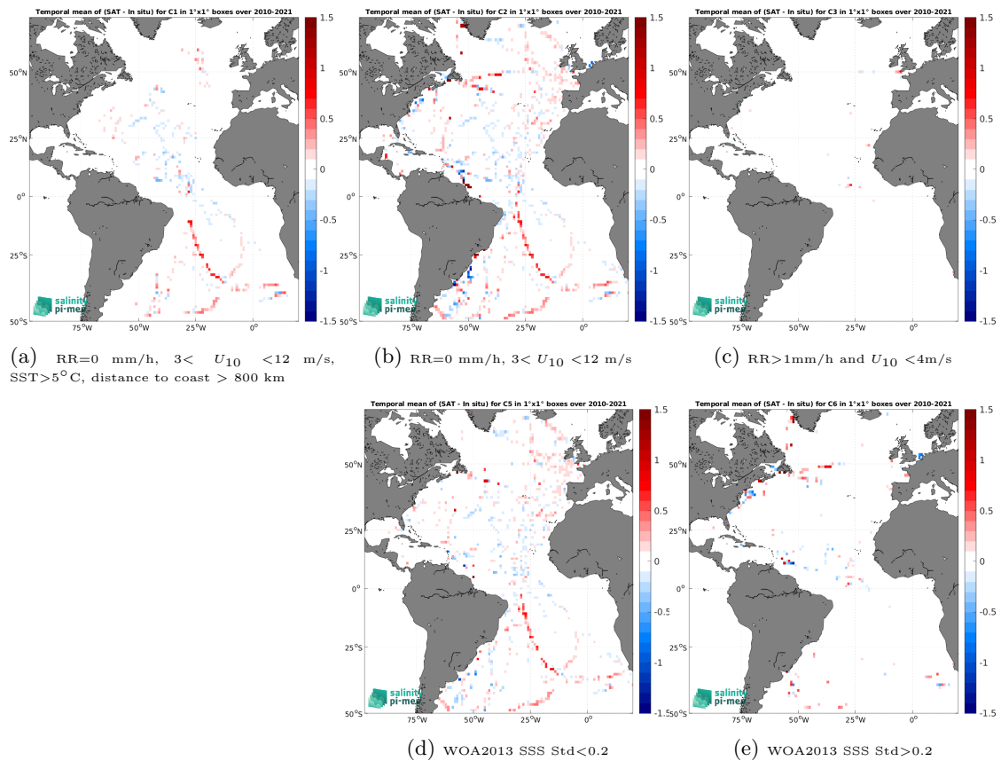
Figure 14: Temporal mean gridded over spatial boxes of size 1^\circ \times 1^\circ of \Delta\text{SSS} (CCI SSS L4 Merged-OI v4.41 - 7-day running (ESA) - TSG (GOSUD-Sailing-ship)) for 5 different subdatasets corresponding to:RR=0 mm/h, 3 < U_{10} < 12 m/s, SST >5^\circ\text{C} , distance to coast > 800 km (a), RR=0 mm/h, 3 < U_{10} < 12 m/s (b), RR >1 mm/h and U_{10} < 4 m/s (c), WOA2013 SSS Std <0.2 (d), WOA2013 SSS Std >0.2 (e).
