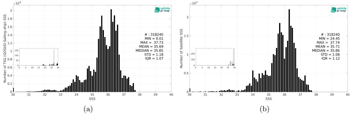
Figure 3: Histograms of SSS from TSG (GOSUD-Sailing-ship) (a) and CCI SSS L4 Merged-OI v4.41 - 7-day running (ESA) (b) considering all match-up pairs per bins of 0.1 over the Atlantic Ocean Pi-MEP region and for the full satellite product period.
