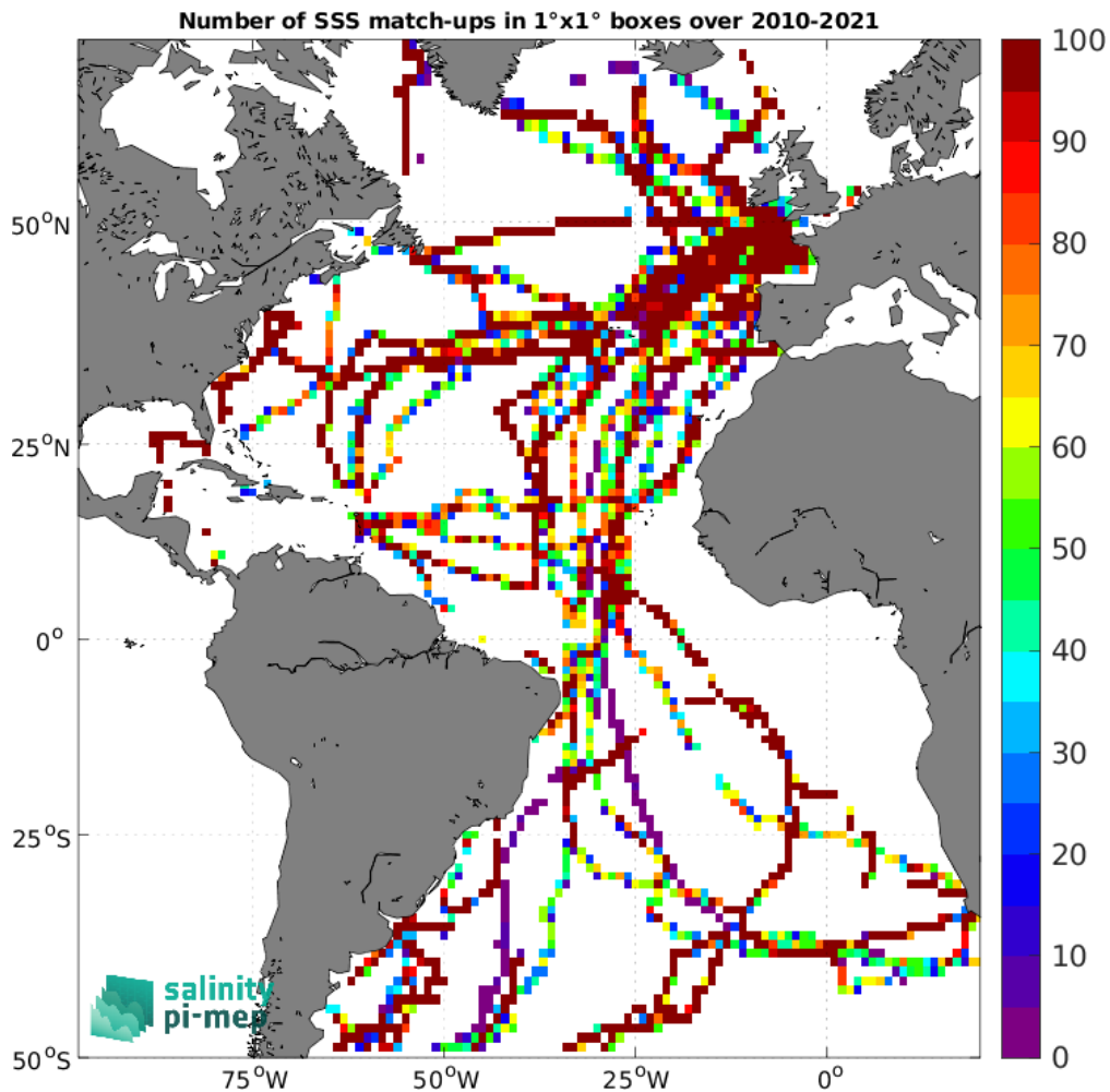
Figure 5: Number of SSS match-ups between TSG (GOSUD-Sailing-ship) SSS and the CCI SSS L4 Merged-OI v4.41 - 7-day running (ESA) SSS product for the Atlantic Ocean Pi-MEP region over 1^\circ \times 1^\circ boxes and for the full satellite product period.
