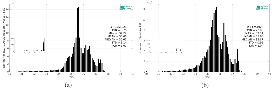
Figure 3: Histograms of SSS from TSG (GOSUD-Research-vessel) (a) and CCI SSS L4 Merged-OI v4.41 - 7-day running (ESA) (b) considering all match-up pairs per bins of 0.1 over the Atlantic Ocean Pi-MEP region and for the full satellite product period.
