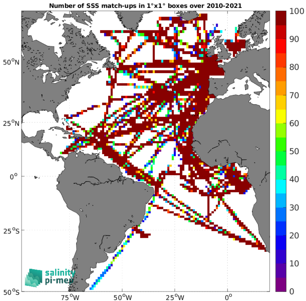
Figure 5: Number of SSS match-ups between TSG (GOSUD-Research-vessel) SSS and the CCI SSS L4 Merged-OI v4.41 - 7-day running (ESA) SSS product for the Atlantic Ocean Pi-MEP region over 1^\circ \times 1^\circ boxes and for the full satellite product period.
