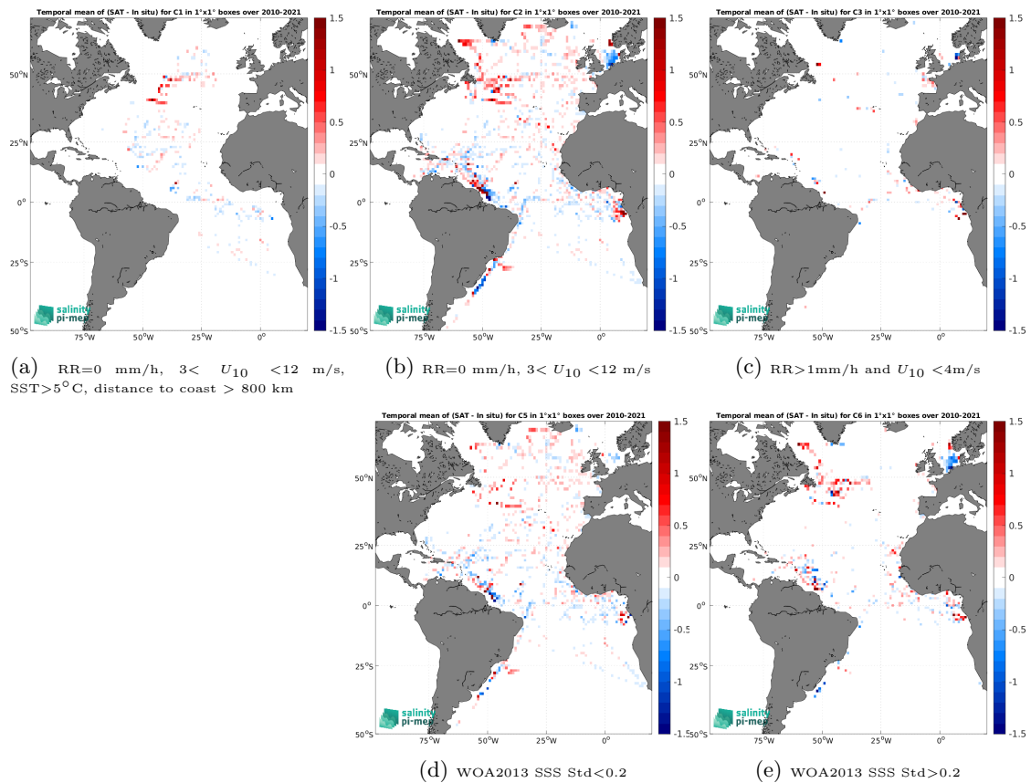
Figure 14: Temporal mean gridded over spatial boxes of size 1^\circ \times 1^\circ of \Delta\text{SSS} (CCI SSS L4 Merged-OI v4.41 - 7-day running (ESA) - TSG (GOSUD-Research-vessel)) for 5 different subdatasets corresponding to:RR=0 mm/h, 3 < U_{10} < 12 m/s, SST>5°C, distance to coast > 800 km (a), RR=0 mm/h, 3 < U_{10} < 12 m/s (b), RR>1mm/h and U_{10} < 4 m/s (c), WOA2013 SSS Std<0.2 (d), WOA2013 SSS Std>0.2 (e).
