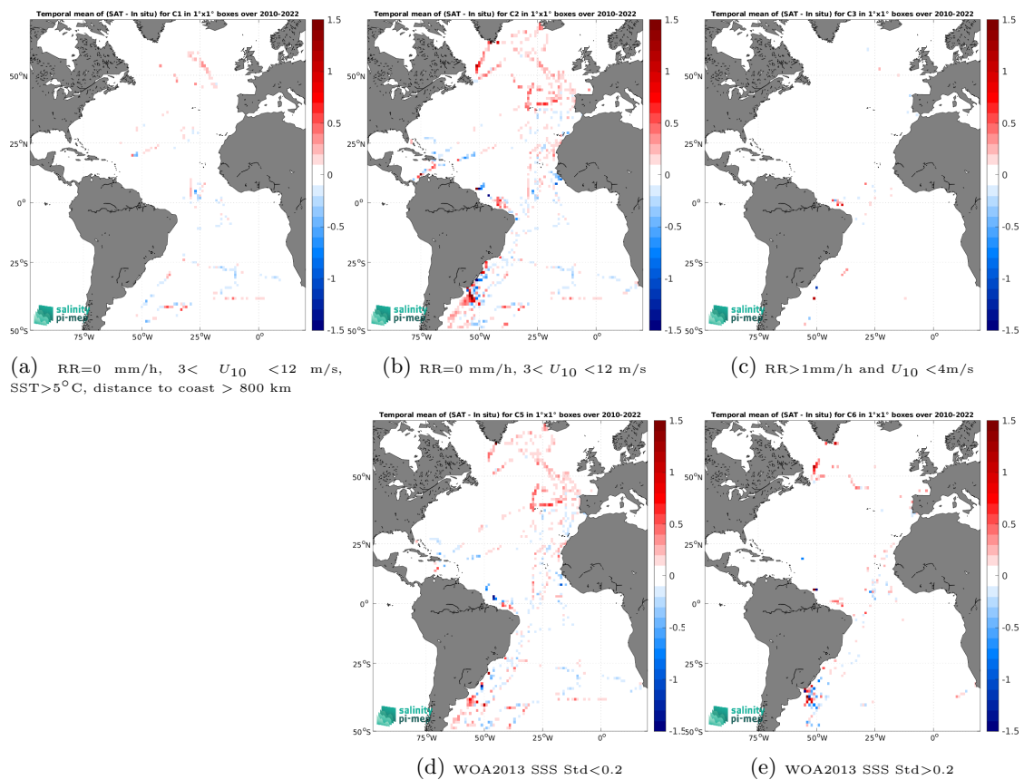
Figure 14: Temporal mean gridded over spatial boxes of size 1^\circ \times 1^\circ of \Delta\text{SSS} (CCI SSS L4 Merged-OI v4.41 - 7-day running (ESA) - TSG (CSIC-UTM)) for 5 different subdatasets corresponding to:RR=0 mm/h, 3 < U_{10} < 12 m/s, SST>5°C, distance to coast > 800 km (a), RR=0 mm/h, 3 < U_{10} < 12 m/s (b), RR>1mm/h and U_{10} < 4 m/s (c), WOA2013 SSS Std<0.2 (d), WOA2013 SSS Std>0.2 (e).
