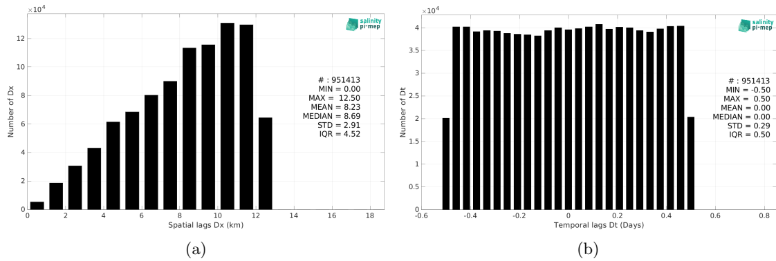
Figure 6: Histograms of the spatial (a) and temporal (b) lags between the location/time of the TSG (CSIC-UTM) measurement and the date of the corresponding CCI SSS L4 Merged-OI v4.41 - 7-day running (ESA) SSS pixel.
