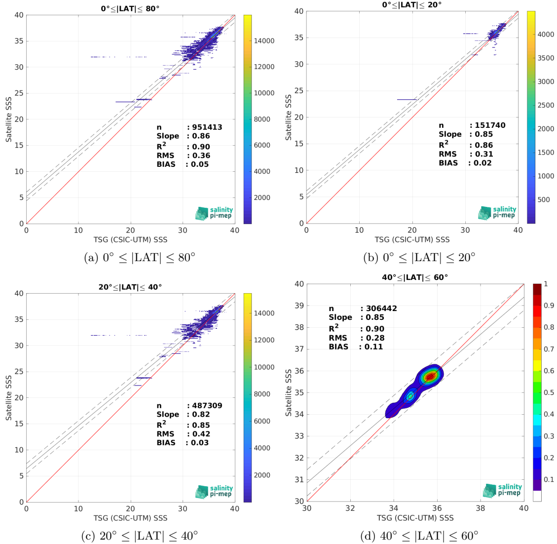
Figure 10: Contour maps of the concentration of CCI SSS L4 Merged-OI v4.41 - 7-day running (ESA) SSS (y-axis) versus TSG (CSIC-UTM) SSS (x-axis) at match-up pairs for different latitude bands. For each plot, the red line shows x=y . The black thin and dashed lines indicate a linear fit through the data cloud and the \pm 95\% confidence levels, respectively. The number match-up pairs n , the slope and R^2 coefficient of the linear fit, the root mean square (RMS) and the mean bias between satellite and in situ data are indicated for each latitude band in each plots.
