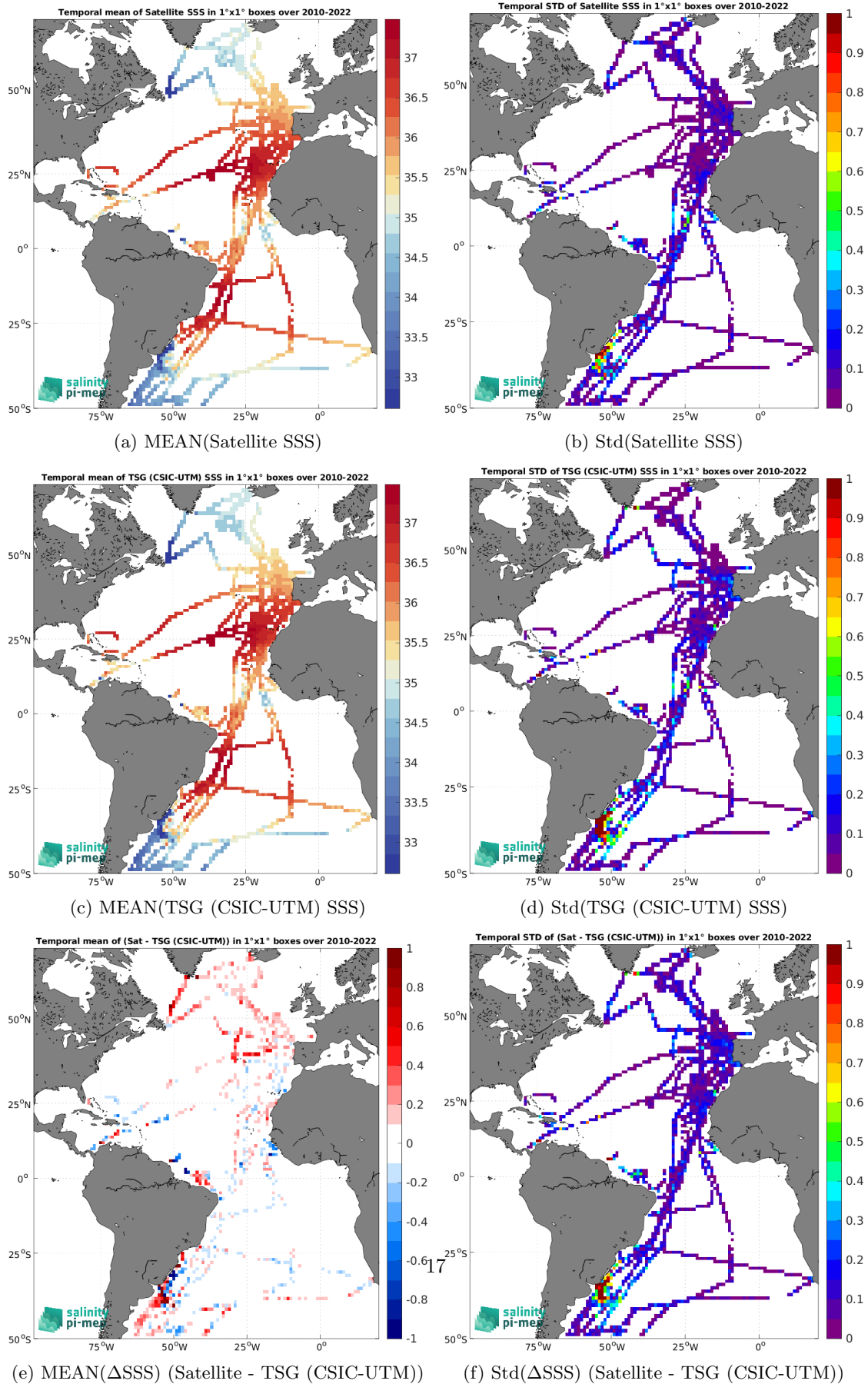
Figure 7: Temporal mean (left) and Std (right) of SSS from CCI SSS L4 Merged-OI v4.41 - 7-day running (ESA) (top), TSG (CSIC-UTM) (middle), and of \Delta SSS (Satellite - TSG (CSIC-UTM)). Only match-up pairs are used to generate these maps.
