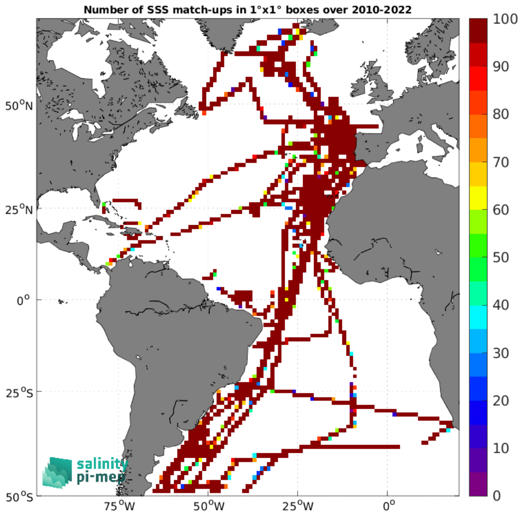
Figure 5: Number of SSS match-ups between TSG (CSIC-UTM) SSS and the CCI SSS L4 Merged-OI v4.41 - 7-day running (ESA) SSS product for the Atlantic Ocean Pi-MEP region over 1^\circ \times 1^\circ boxes and for the full satellite product period.
