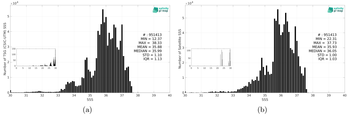
Figure 3: Histograms of SSS from TSG (CSIC-UTM) (a) and CCI SSS L4 Merged-OI v4.41 - 7-day running (ESA) (b) considering all match-up pairs per bins of 0.1 over the Atlantic Ocean Pi-MEP region and for the full satellite product period.
