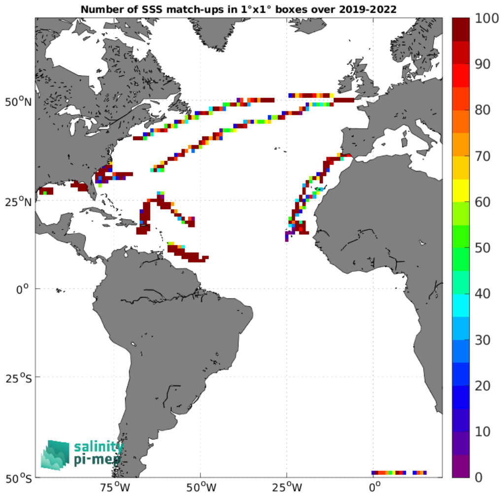
Figure 5: Number of SSS match-ups between Saildrone SSS and the CCI SSS L4 Merged-OI v4.41 - 7-day running (ESA) SSS product for the Atlantic Ocean Pi-MEP region over 1°x1° boxes and for the full satellite product period.
