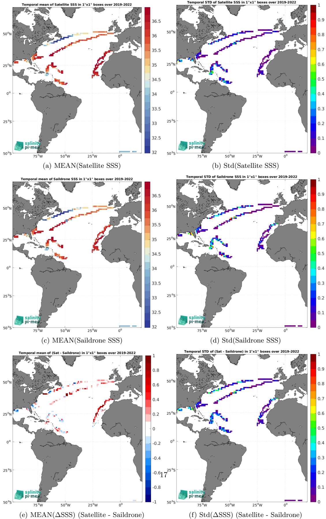
Figure 7: Temporal mean (left) and Std (right) of SSS from CCI SSS L4 Merged-OI v4.41 - 7-day running (ESA) (top), Saildrone (middle), and of \Delta\text{SSS} (Satellite - Saildrone). Only match-up pairs are used to generate these maps.
