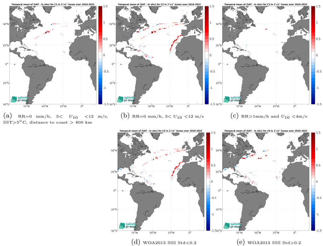
Figure 14: Temporal mean gridded over spatial boxes of size 1^\circ \times 1^\circ of \Delta\text{SSS} (CCI SSS L4 Merged-OI v4.41 - 7-day running (ESA) - Saildrone) for 5 different subdatasets corresponding to:RR=0 mm/h, 3 < U_{10} < 12 m/s, SST >5^\circ\text{C} , distance to coast > 800 km (a), RR=0 mm/h, 3 < U_{10} < 12 m/s (b), RR >1 mm/h and U_{10} < 4 m/s (c), WOA2013 SSS Std <0.2 (d), WOA2013 SSS Std >0.2 (e).
