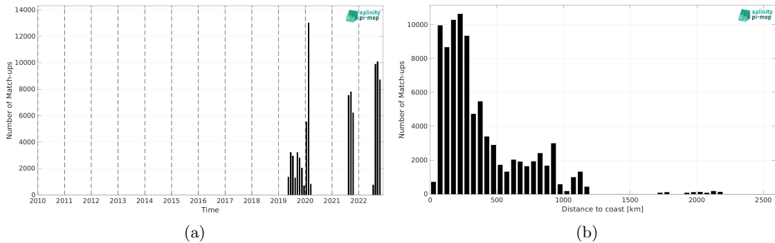
Figure 2: Number of match-ups between Saildrone and CCI SSS L4 Merged-OI v4.41 - 7-day running (ESA) SSS as a function of time (a) and as function of the distance to coast (b) over the Atlantic Ocean Pi-MEP region and for the full satellite product period.
